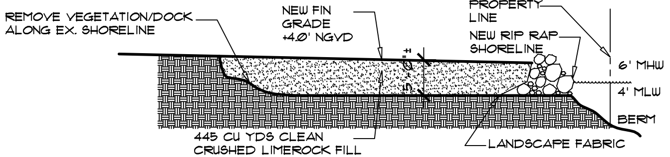
CROSS SECTION 'A' 1/16"
