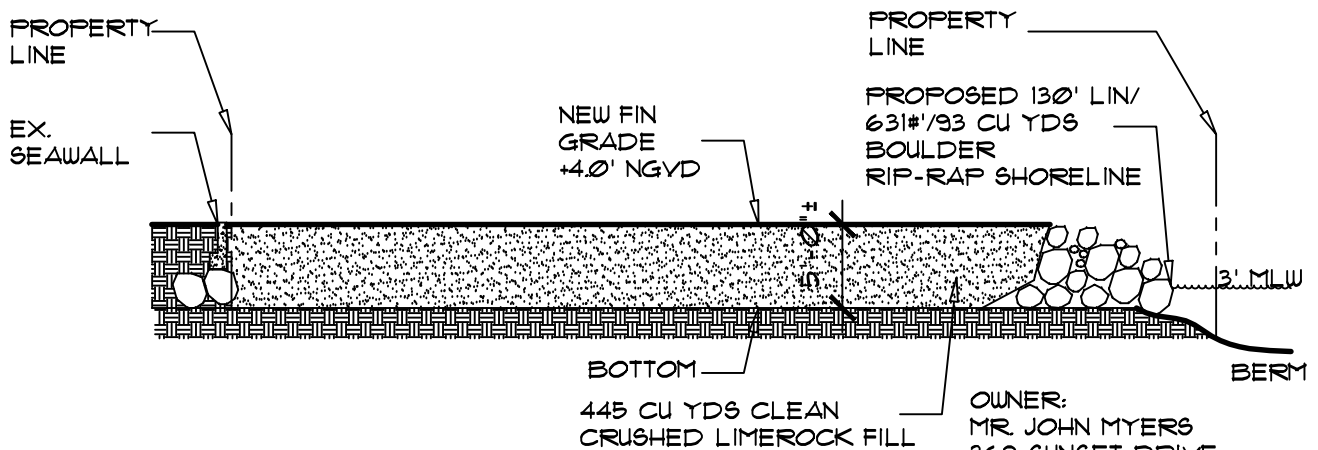
CROSS SECTION 'A' 1/16"
