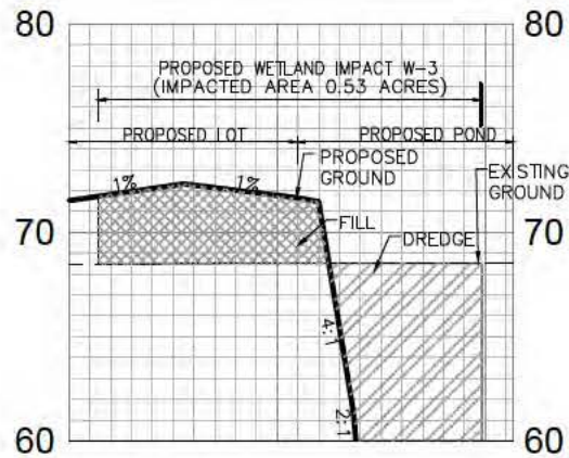
SECTION G
