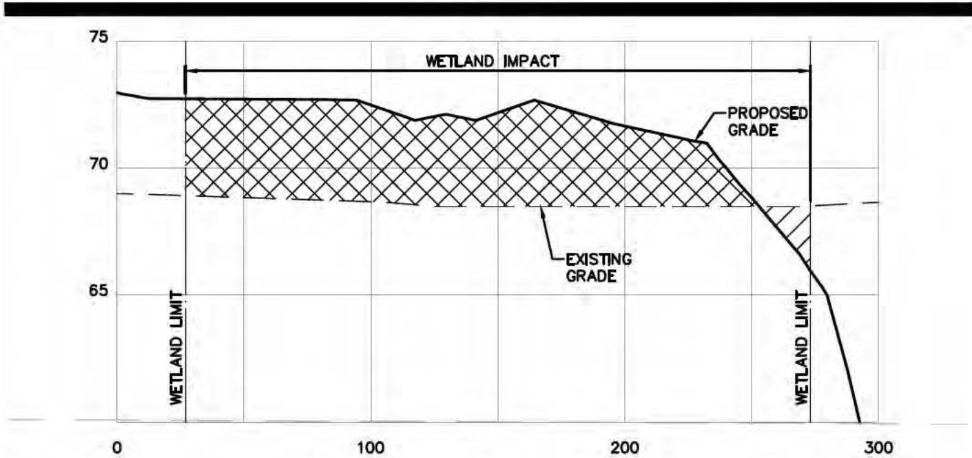
SECTION B-B'
