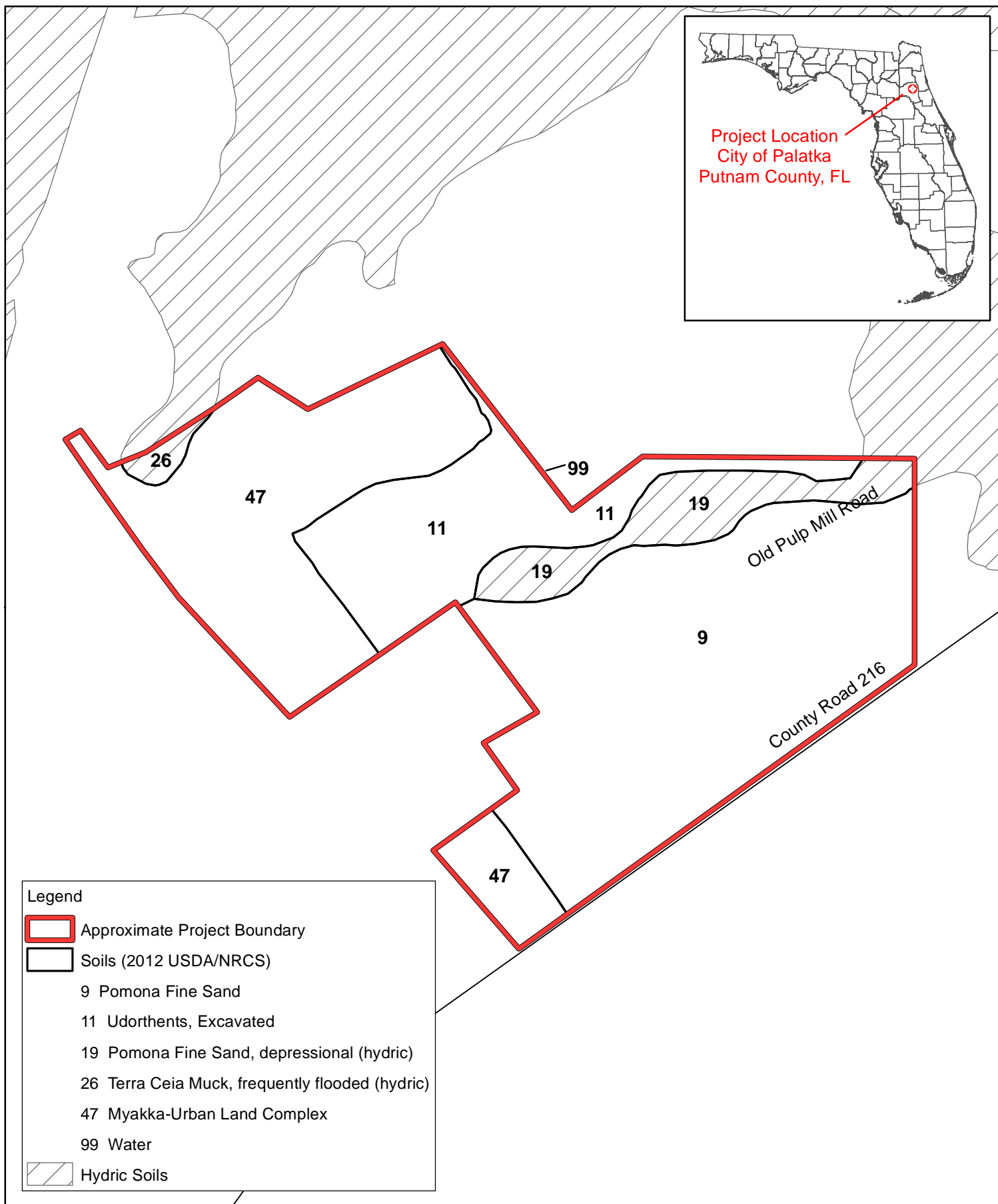
Figure 6 Soils
