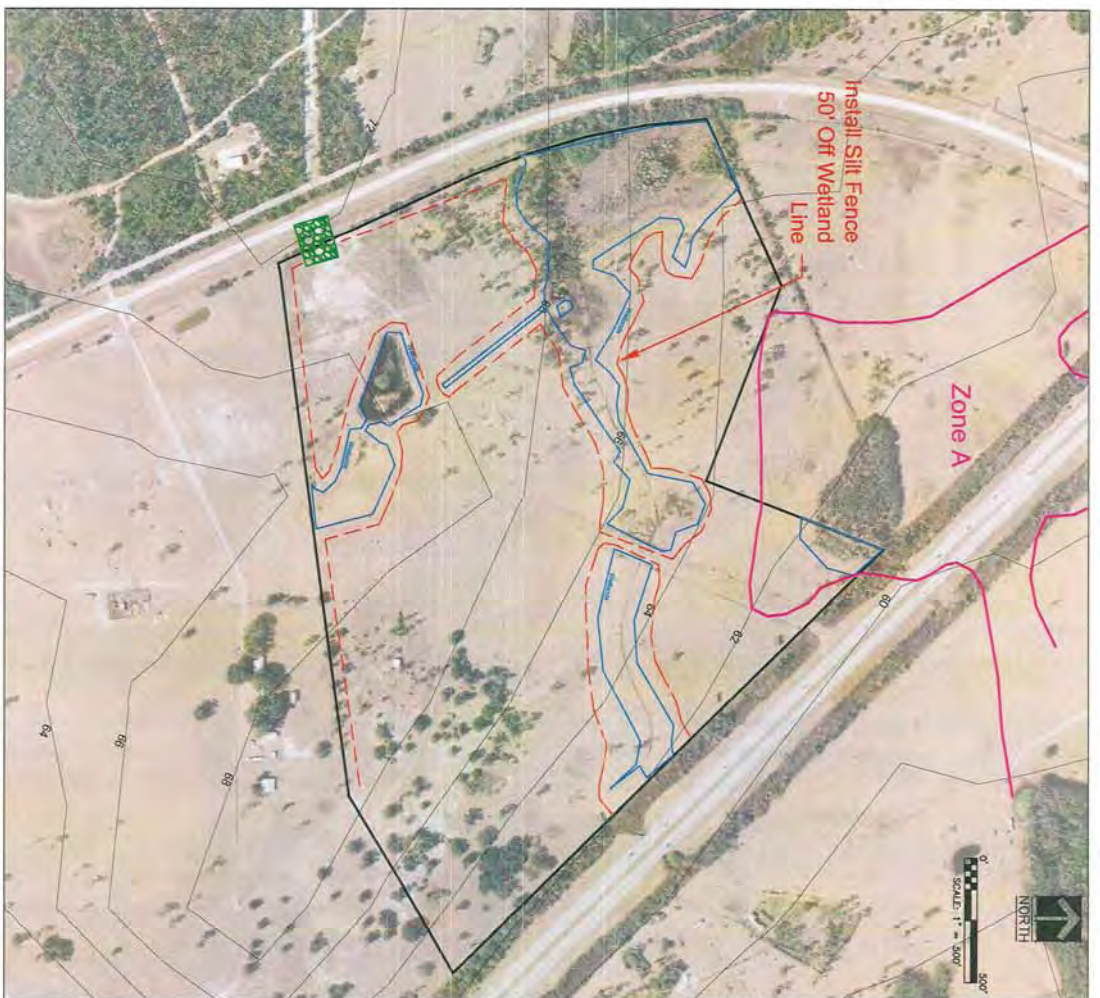
MP 72 Contractor Yard Site Layout
