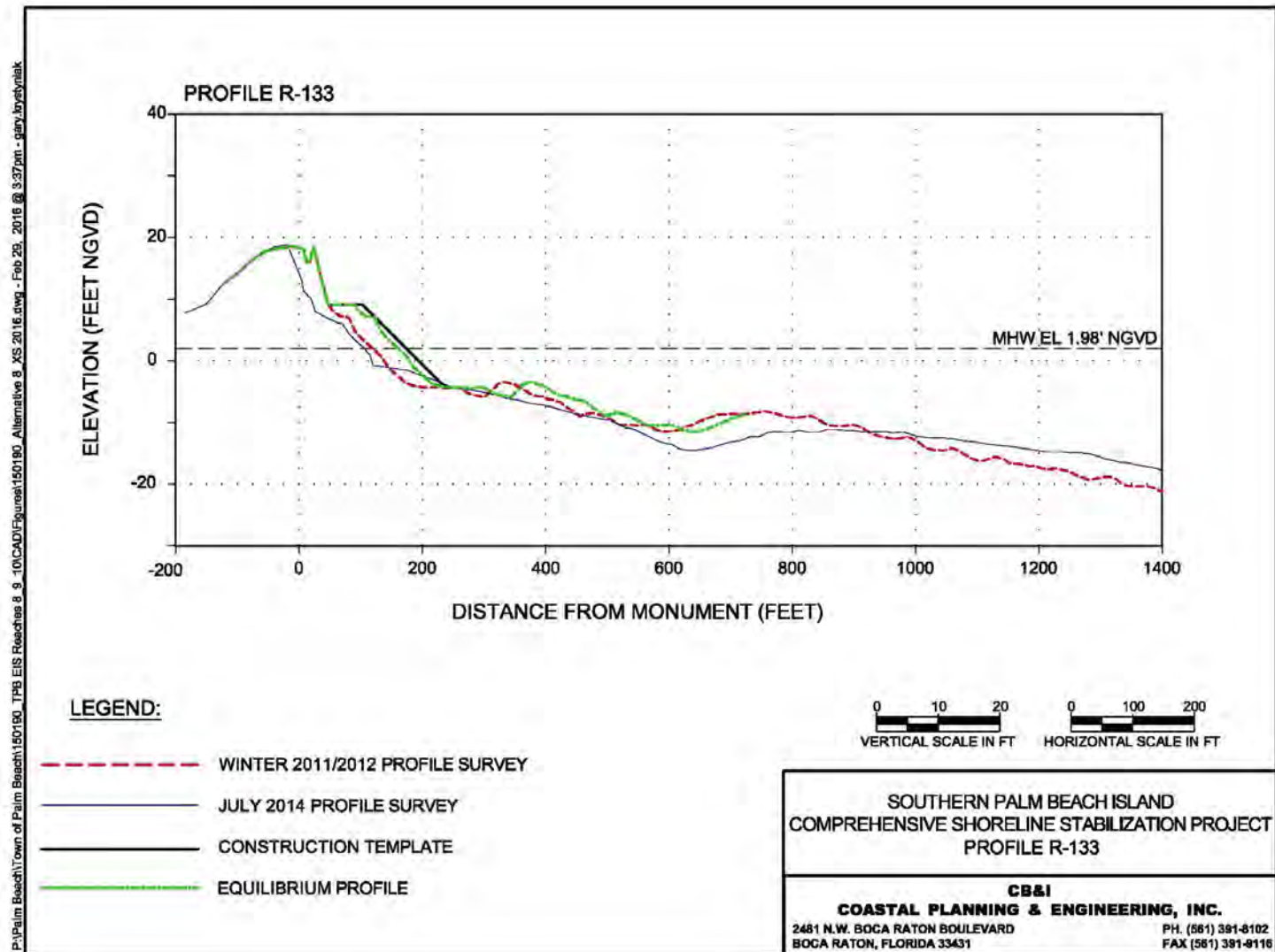
Figure 55. Alternative 7b Profile R-133.
