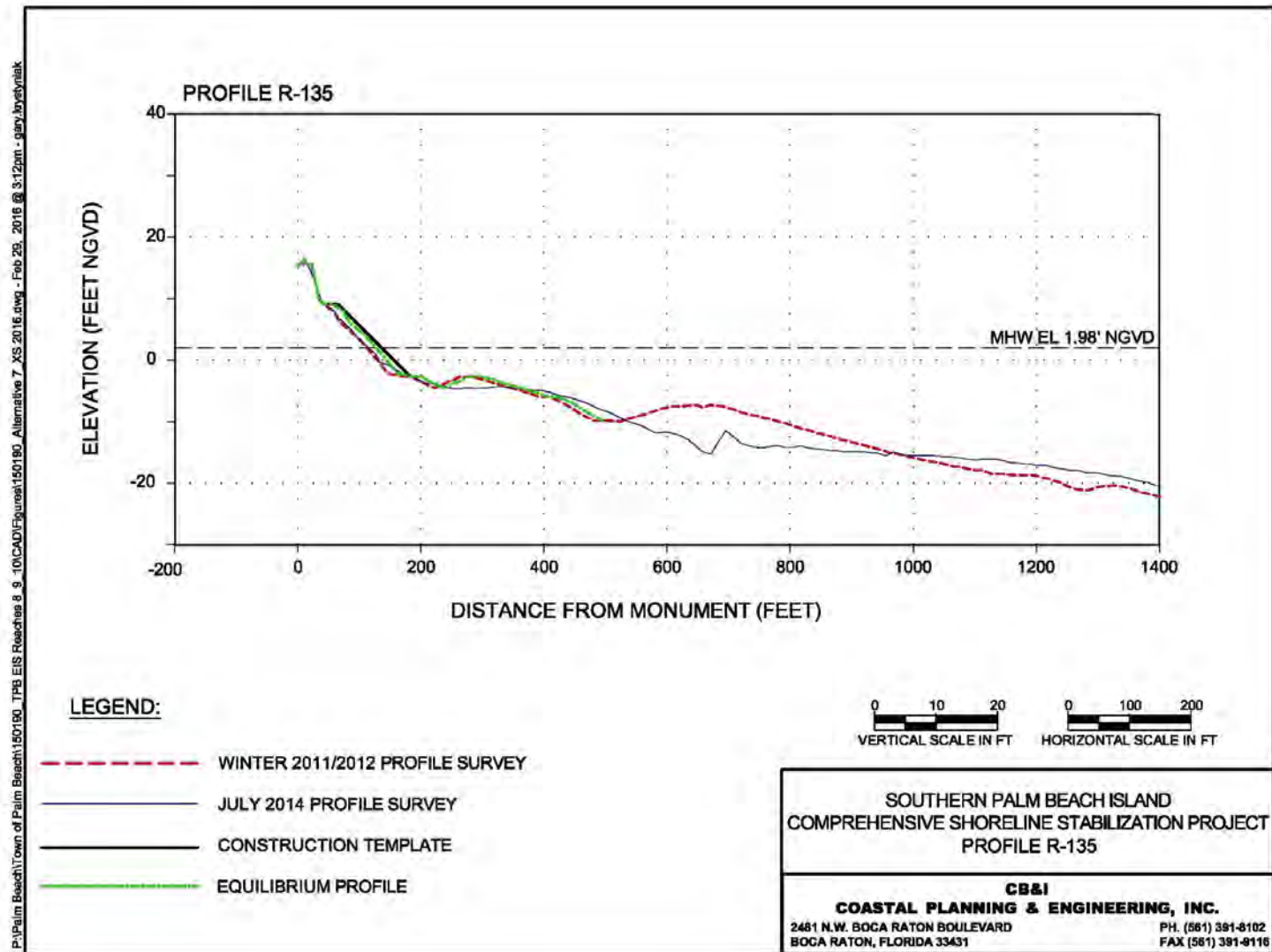
Figure 47. Alternative 7a Profile R-135.
