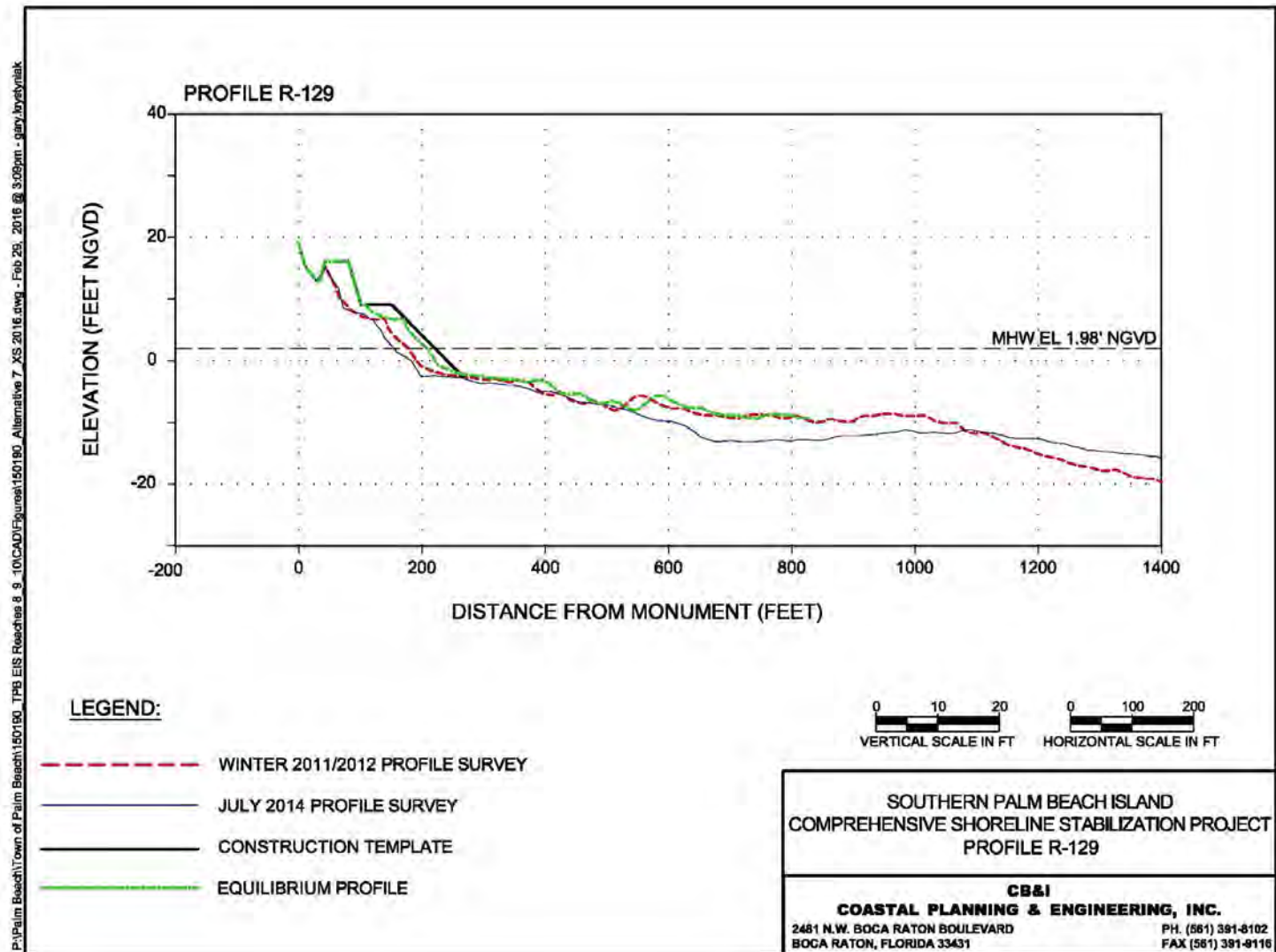
Figure 41. Alternative 7a Profile R-129.
