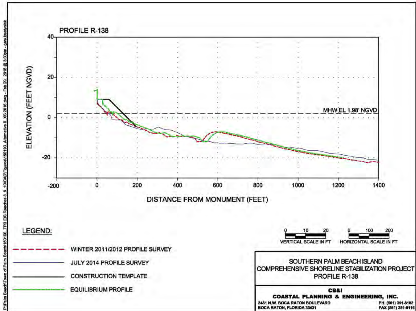
Figure 40. Alternative 6 Profile R-138.
