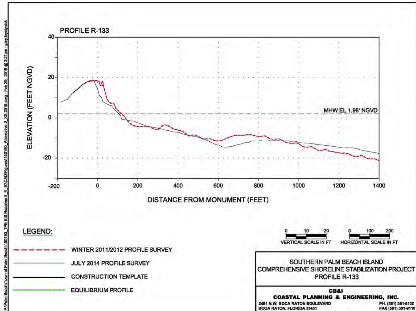
Figure 15. Alternative 4 Profile R-133.
