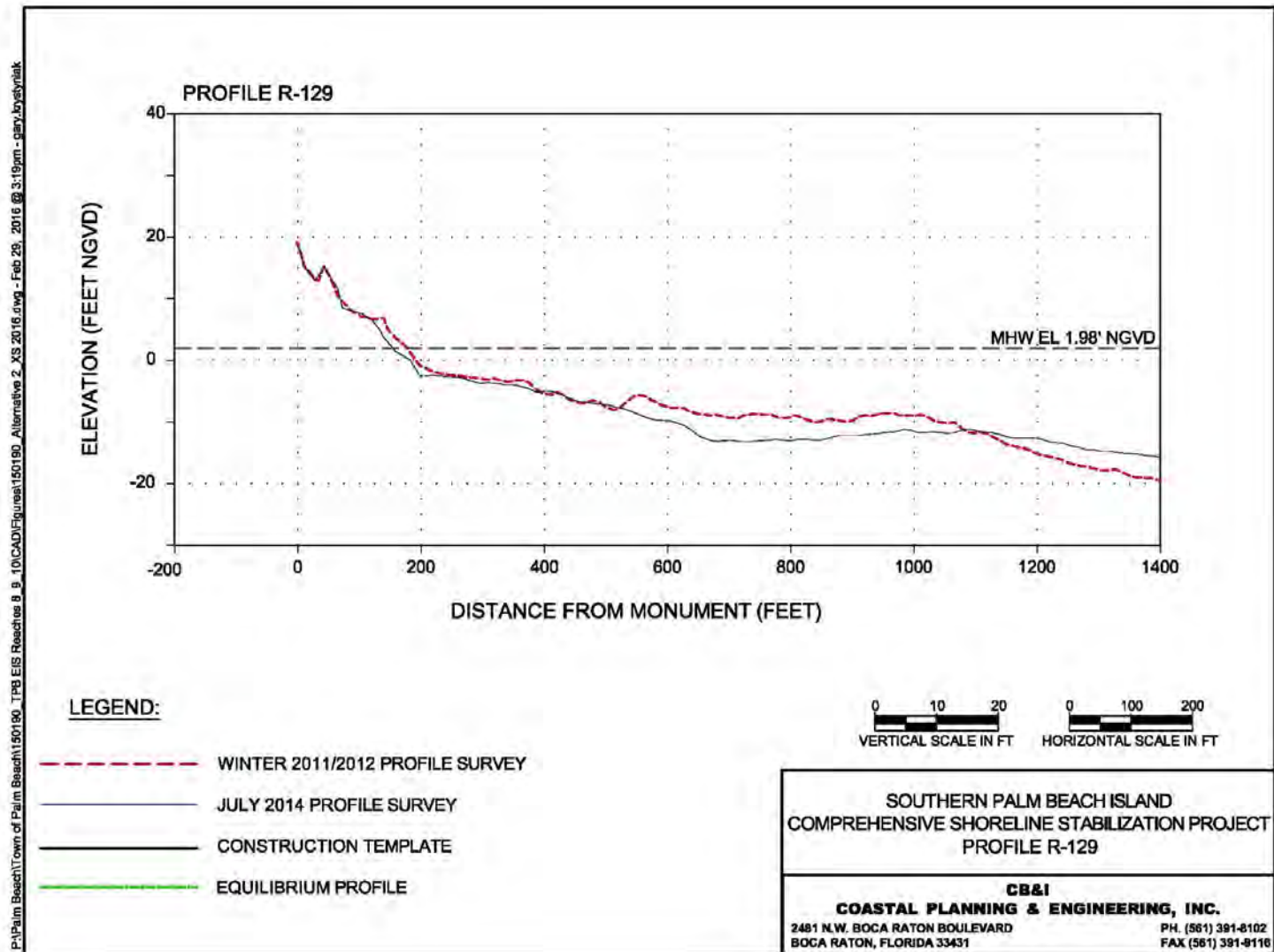
Figure 1. Alternative 2/Alternative 3 Profile R-129.
