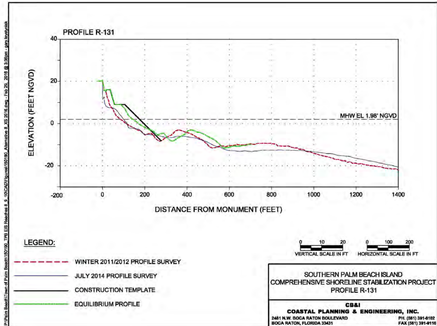
Figure 53. Alternative 7b Profile R-131.
