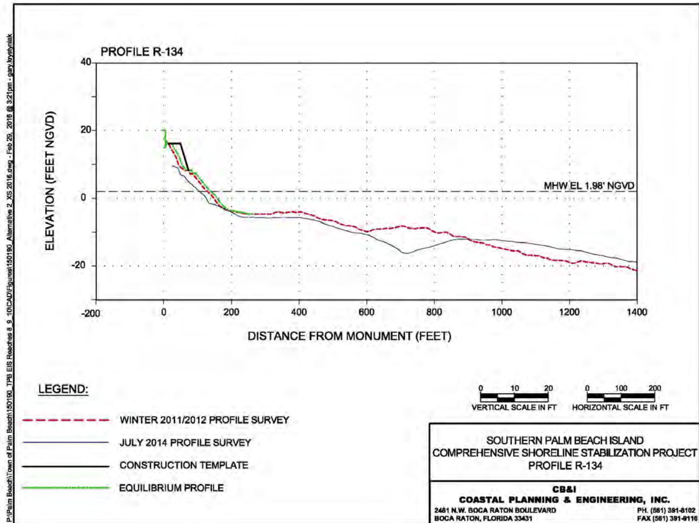
Figure 6. Alternative 2/Alternative 3 Profile R-134.
