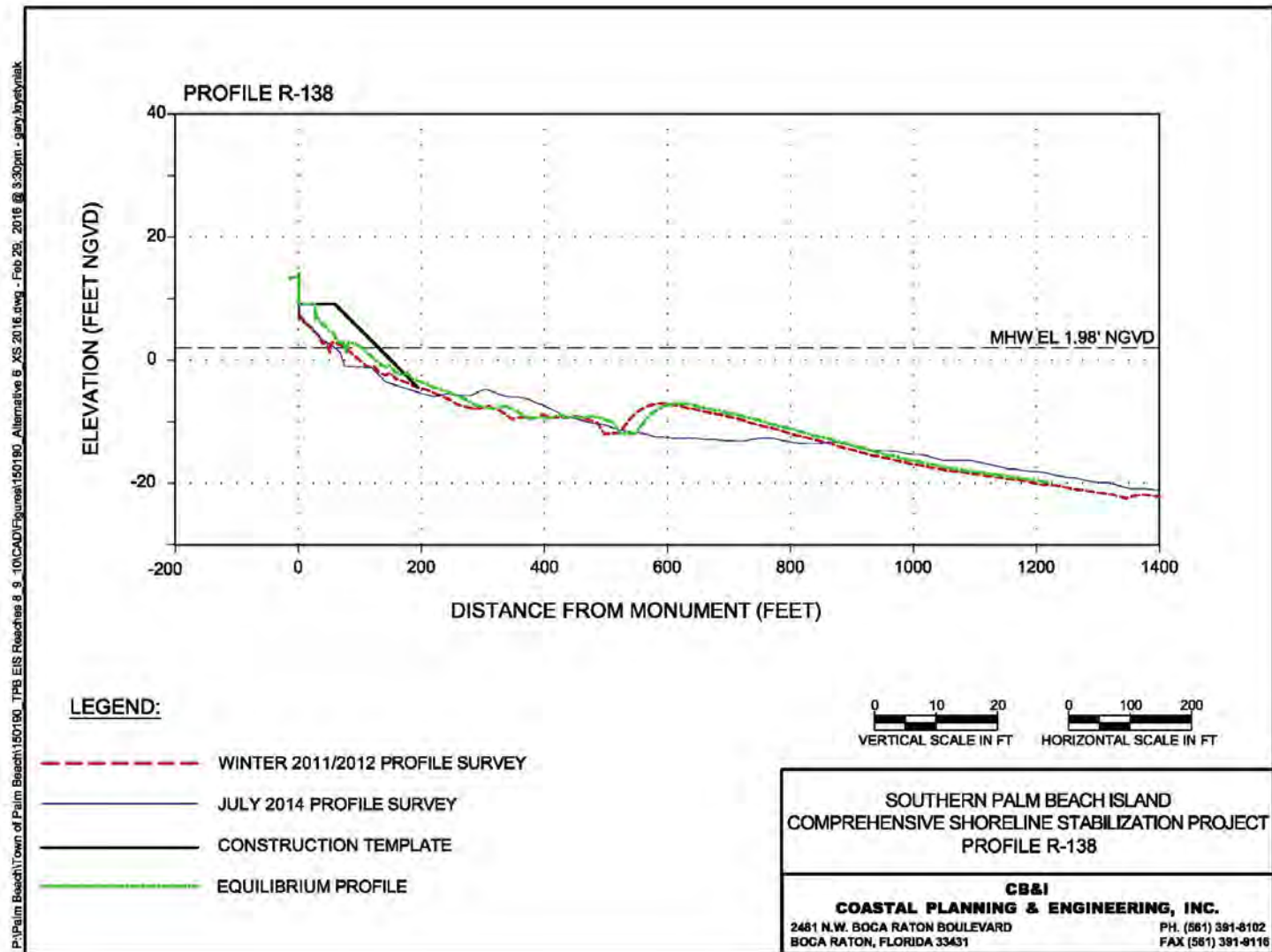
Figure 20. Alternative 4 Profile R-138.
