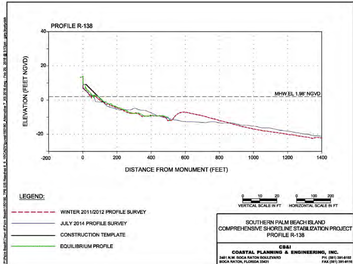
Figure 50. Alternative 7a Profile R-138.
