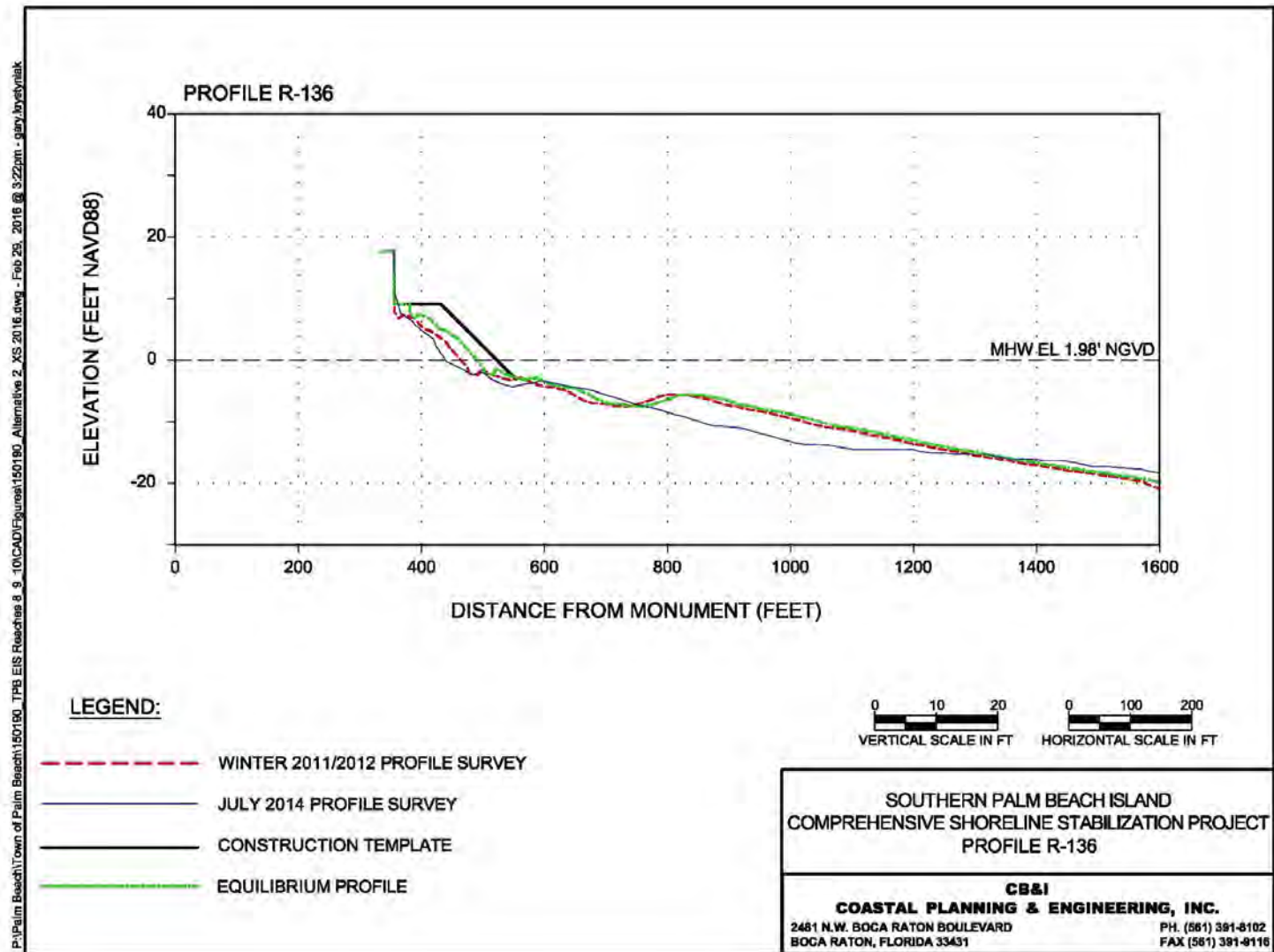
Figure 28. Alternative 5 Profile R-136.
