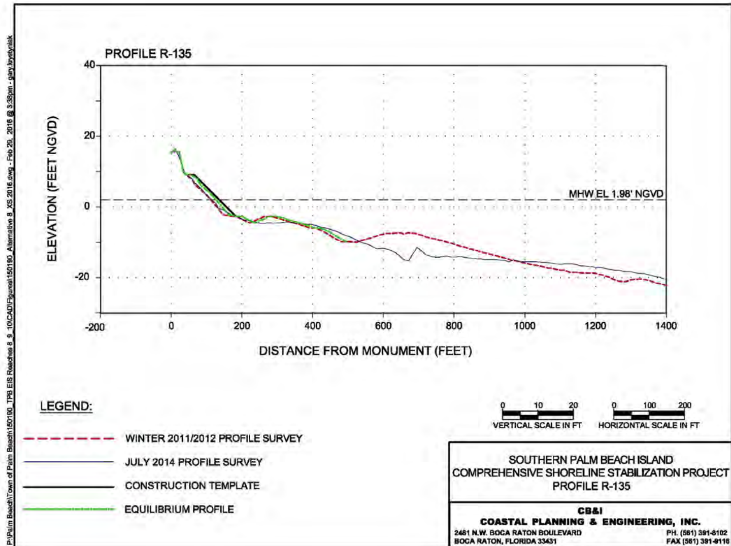
Figure 57. Alternative 7b Profile R-135.
