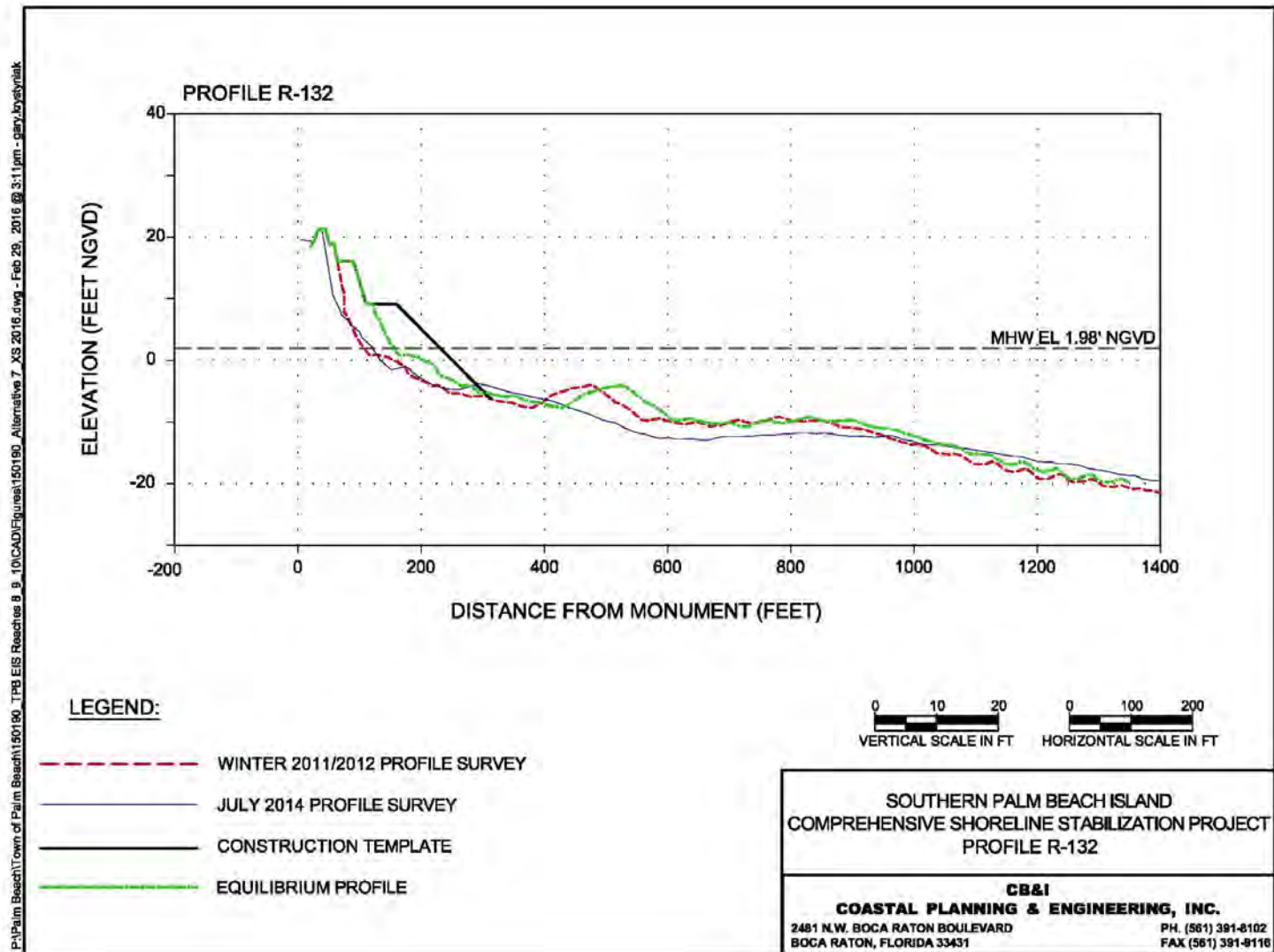
Figure 44. Alternative 7a Profile R-132.
