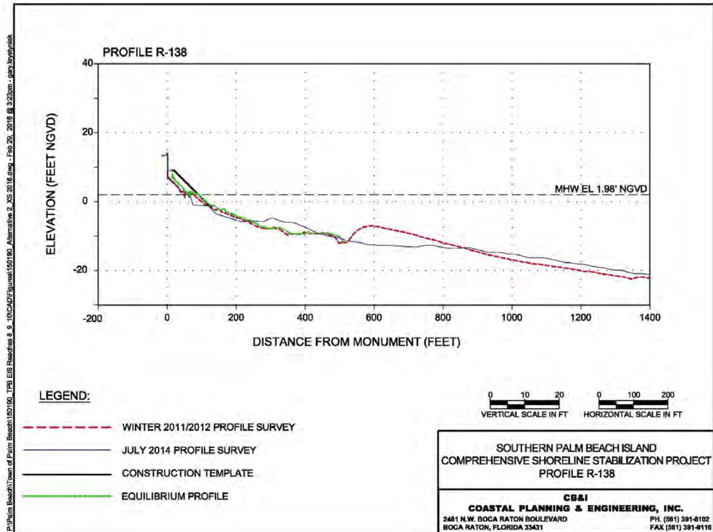
Figure 10. Alternative 2/Alternative 3 Profile R-138.
