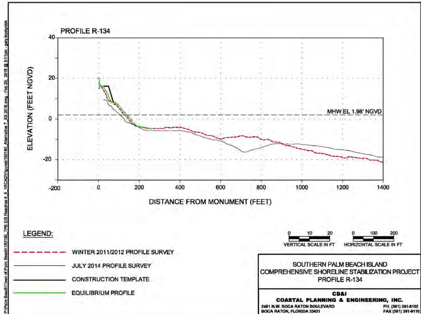
Figure 46. Alternative 7a Profile R-134.
