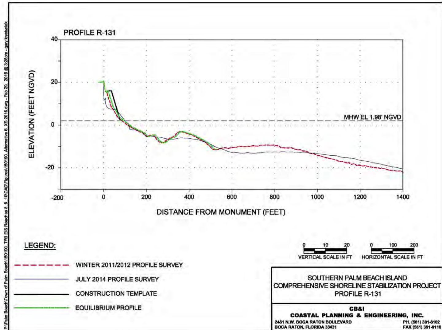
Figure 23. Alternative 5 Profile R-131.
