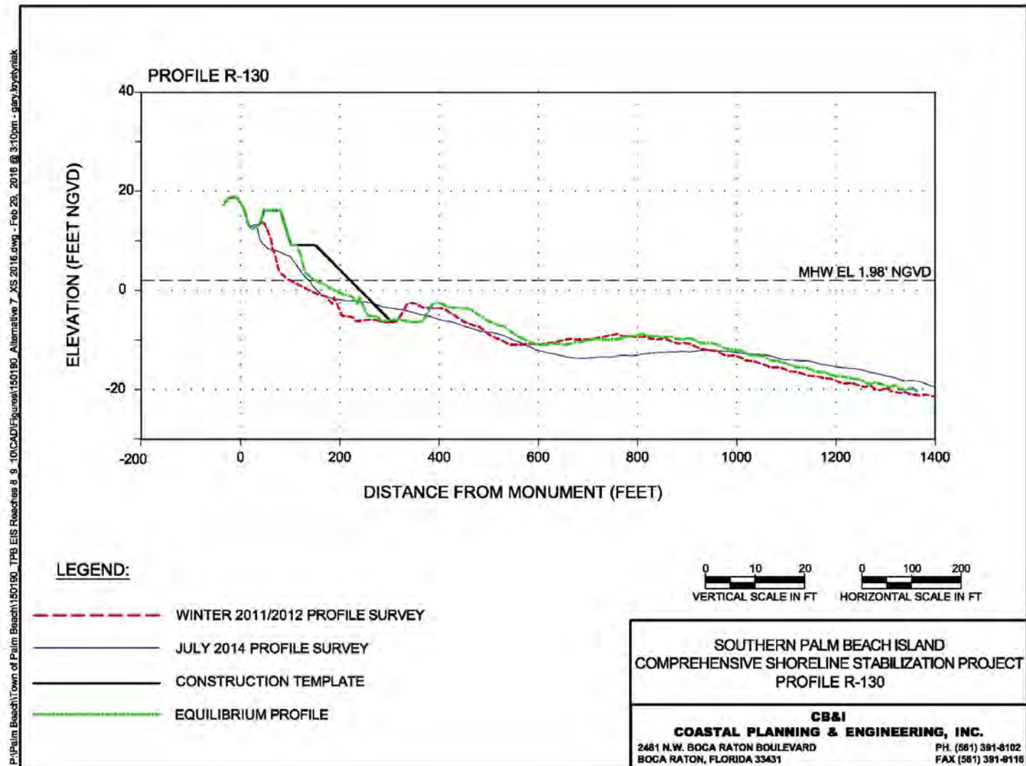
Figure 42. Alternative 7a Profile R-130.
