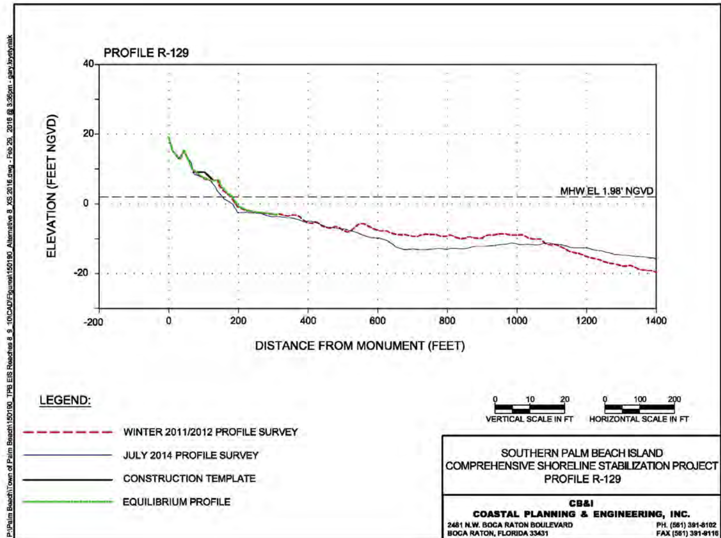
Figure 51. Alternative 7b Profile R-129.
