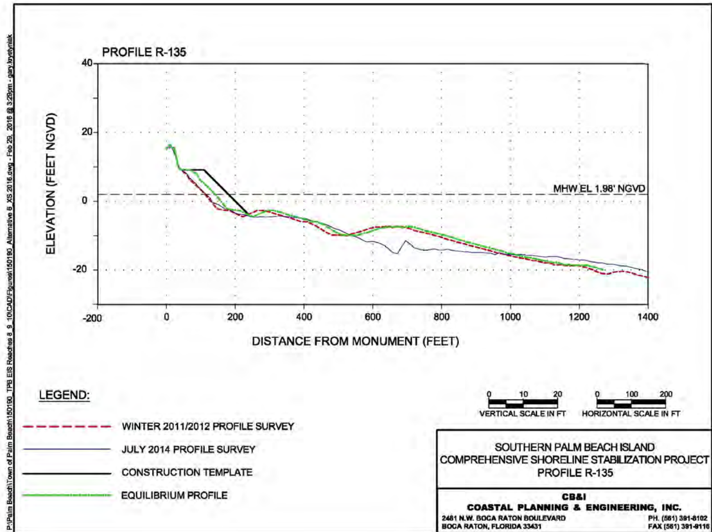
Figure 17. Alternative 4 Profile R-135.
