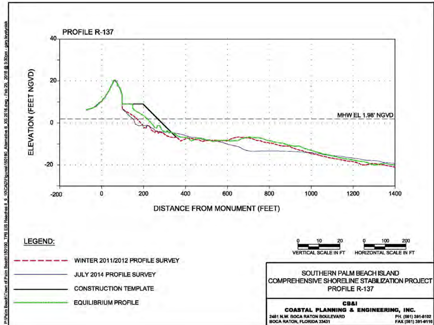
Figure 19. Alternative 4 Profile R-137.
