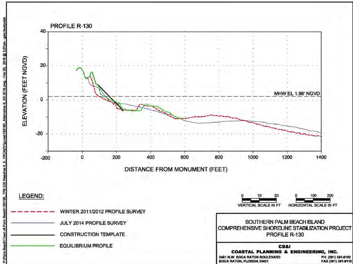
Figure 32. Alternative 6 Profile R-130.
