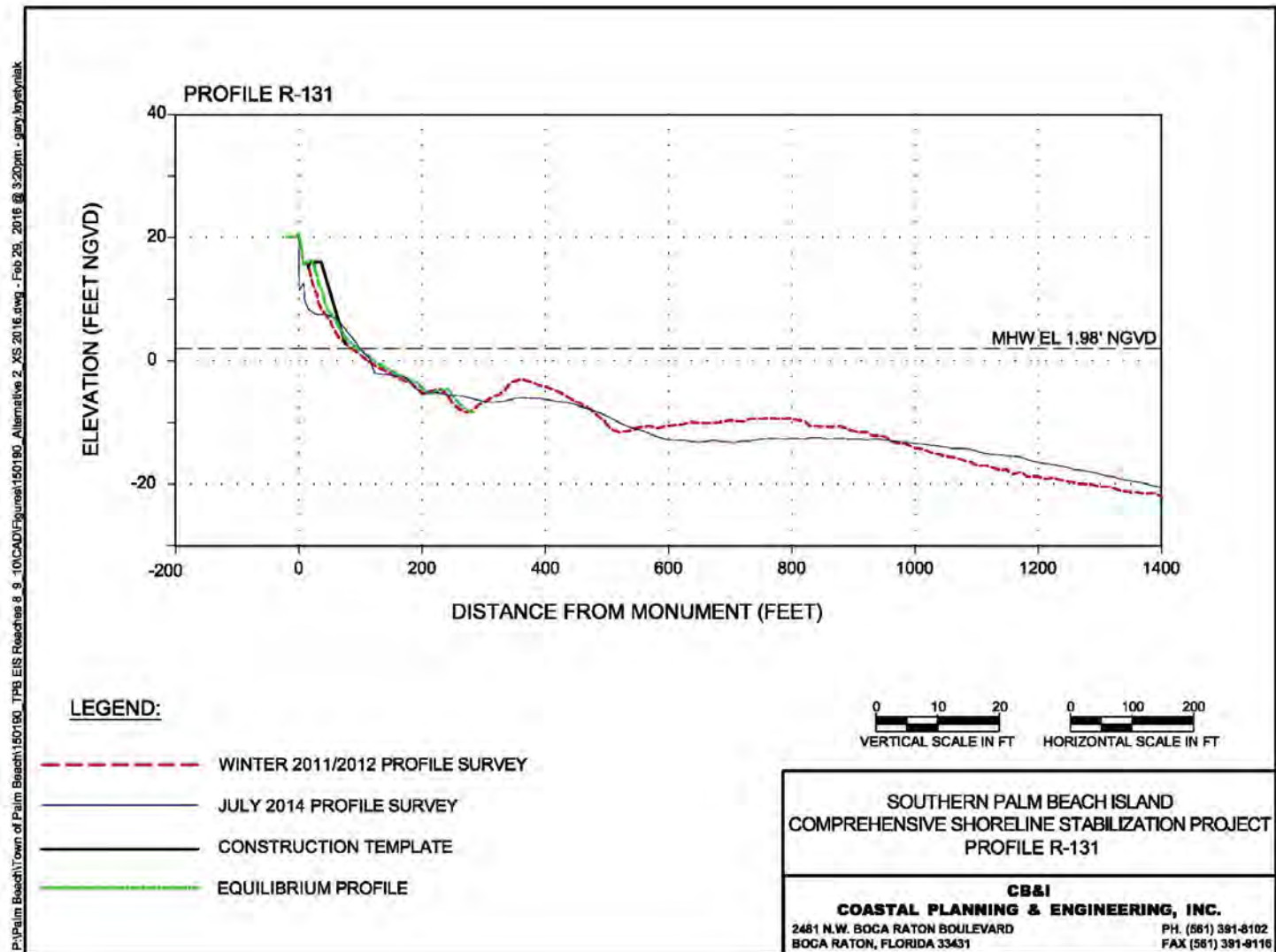
Figure 3. Alternative 2/Alternative 3 Profile R-131.
