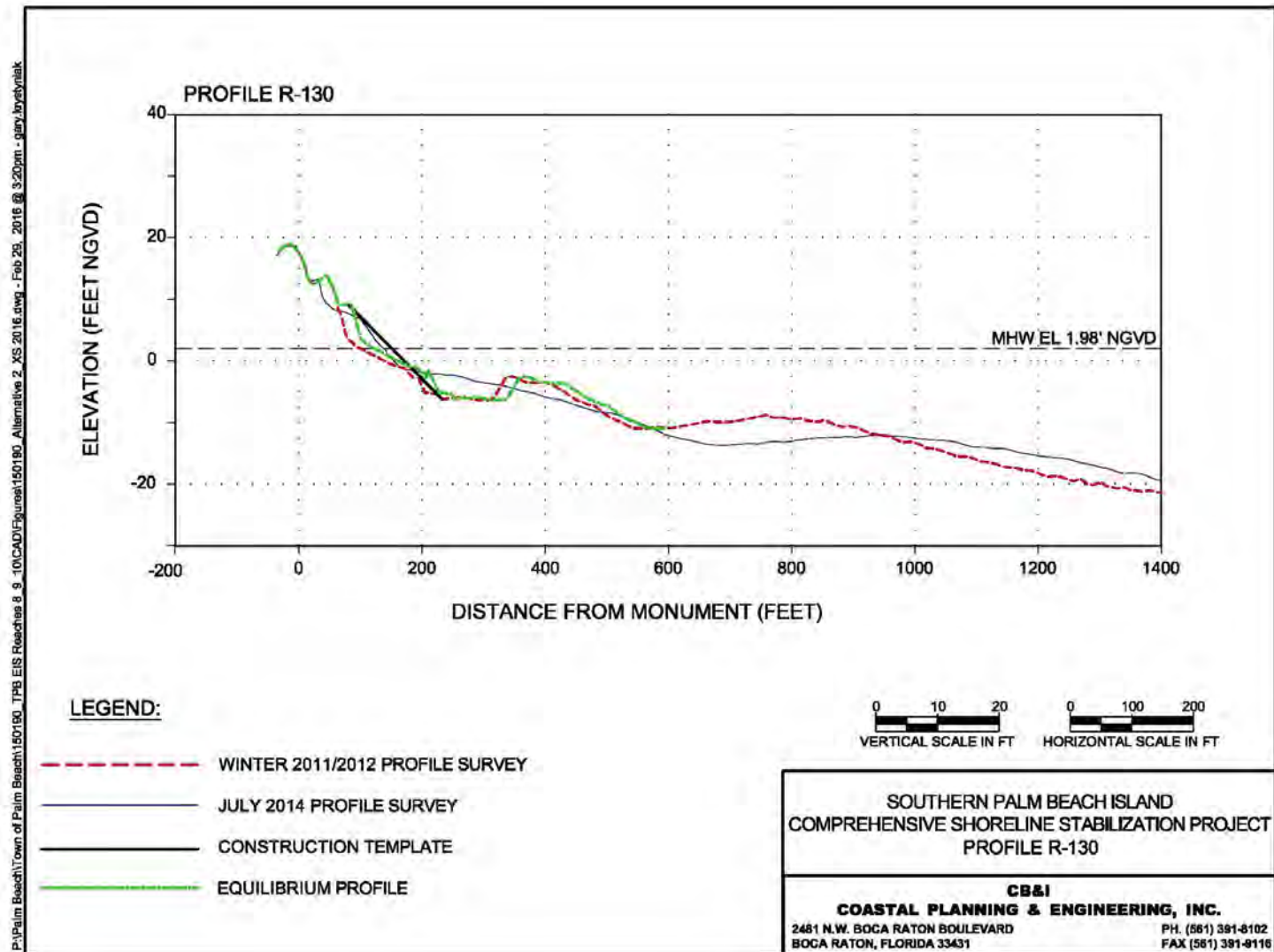
Figure 12. Alternative 4 Profile R-130.
