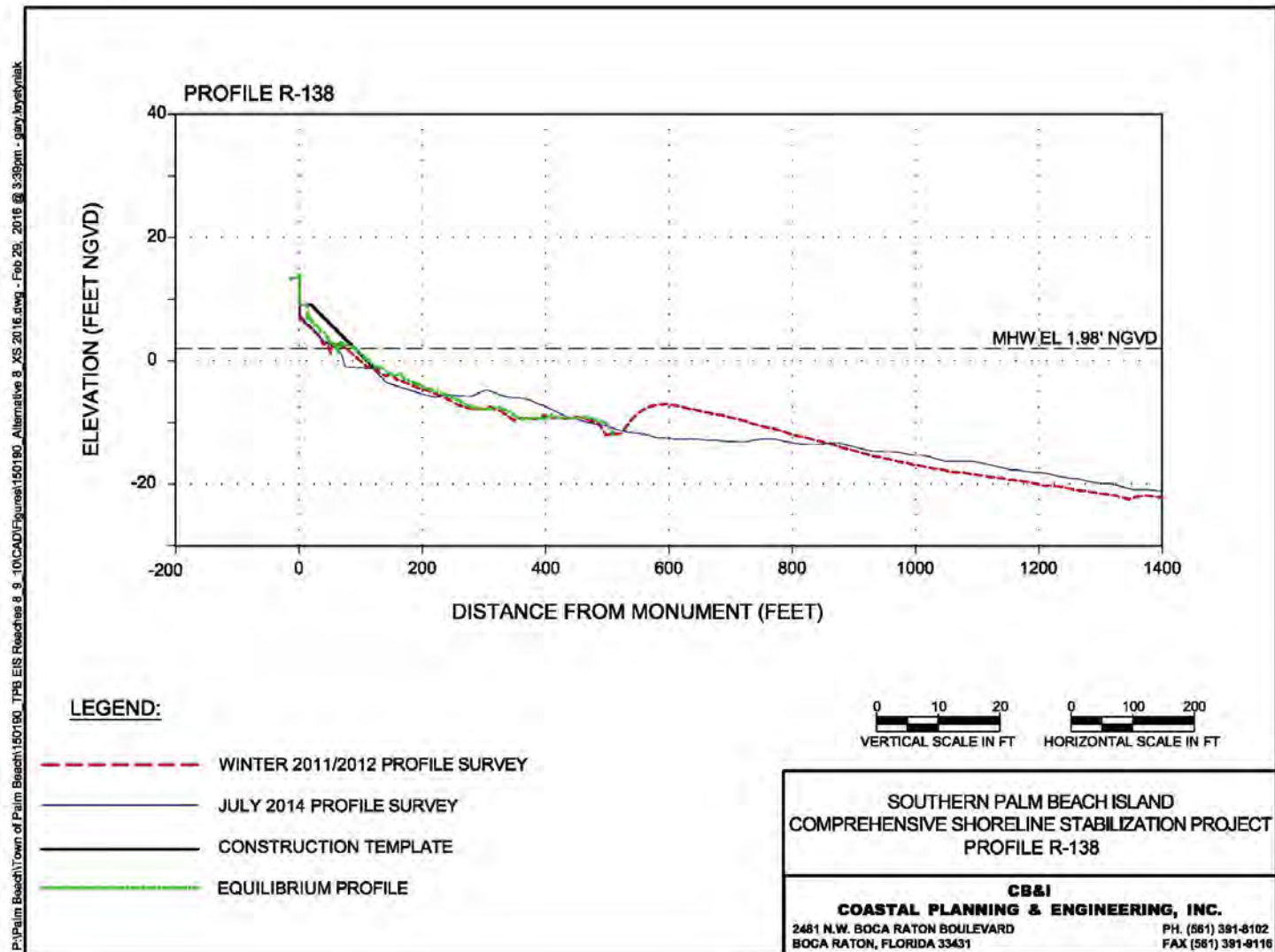
Figure 60. Alternative 7b Profile R-138
