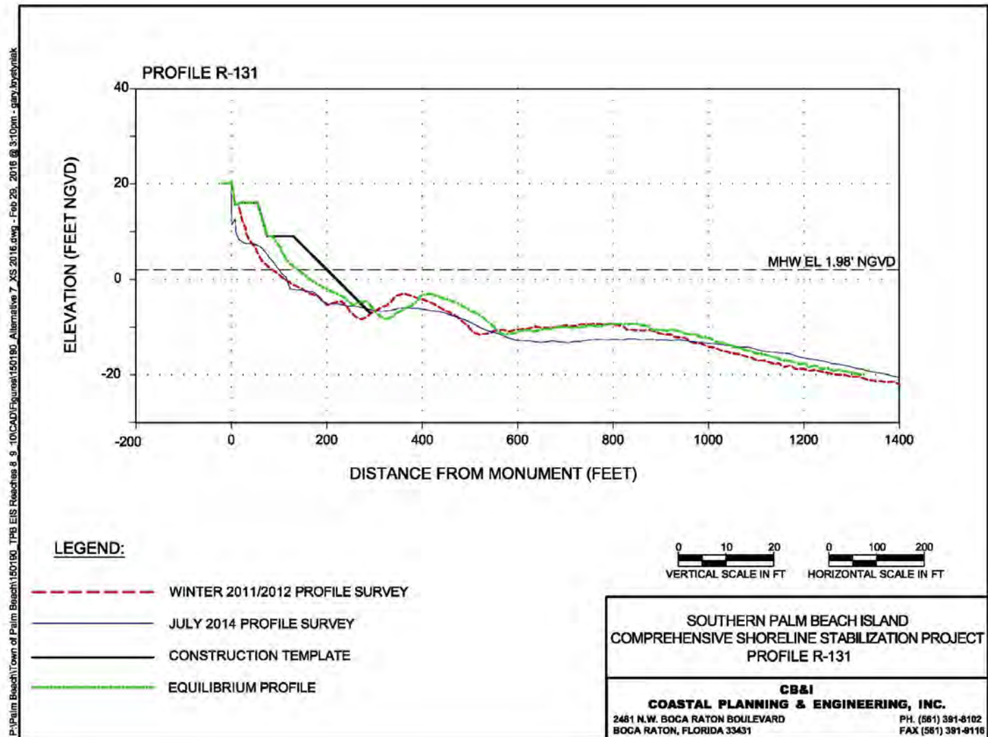
Figure 43. Alternative 7a Profile R-131.
