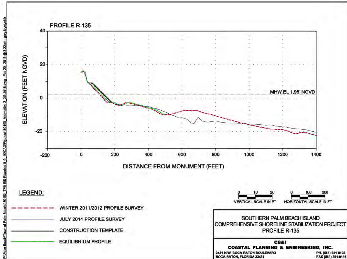
Figure 27. Alternative 5 Profile R-135.
