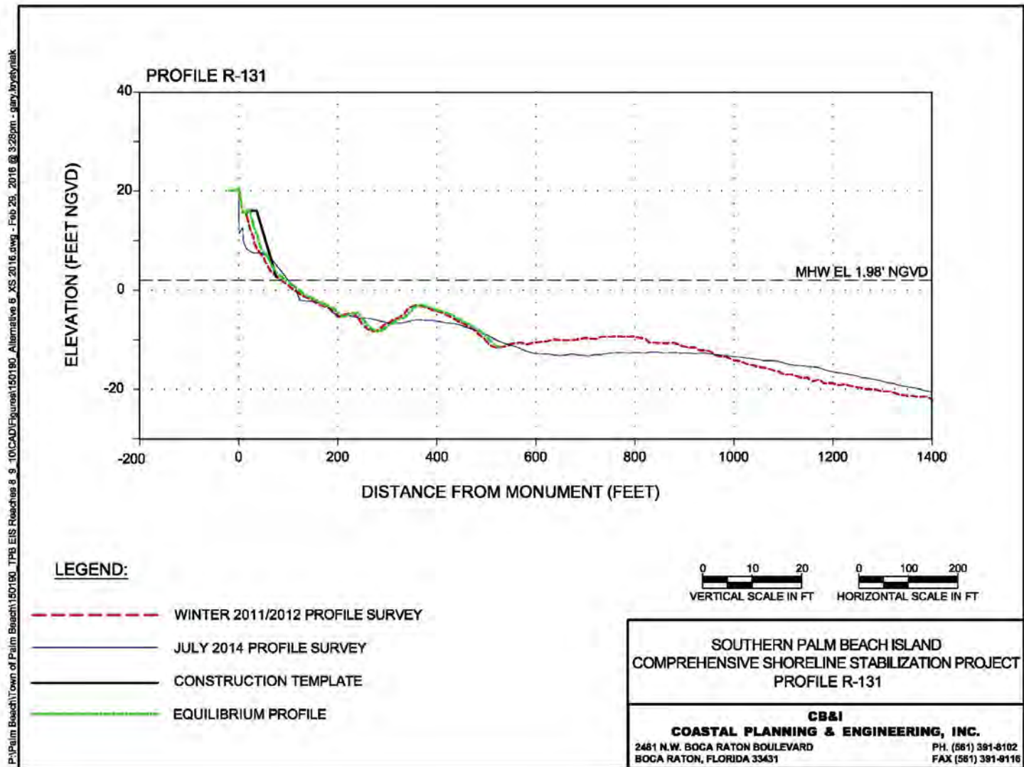
Figure 33. Alternative 6 Profile R-131.
