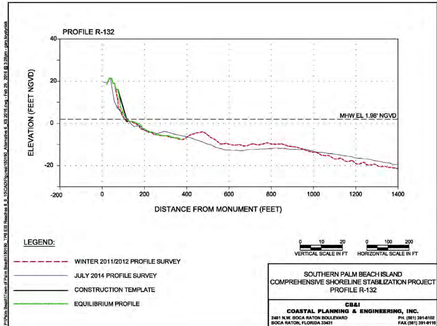
Figure 24. Alternative 5 Profile R-132.
