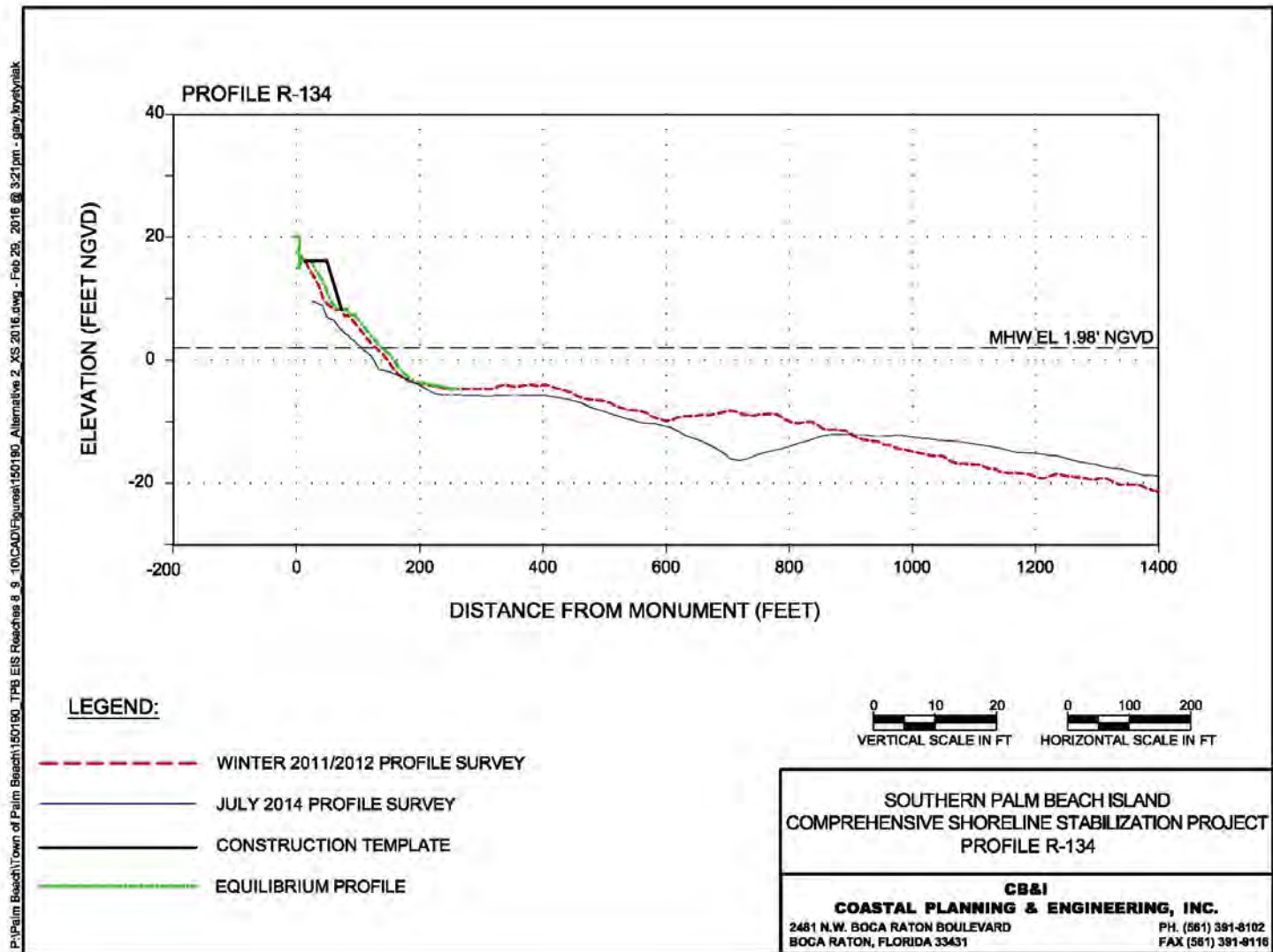
Figure 36. Alternative 6 Profile R-134.
