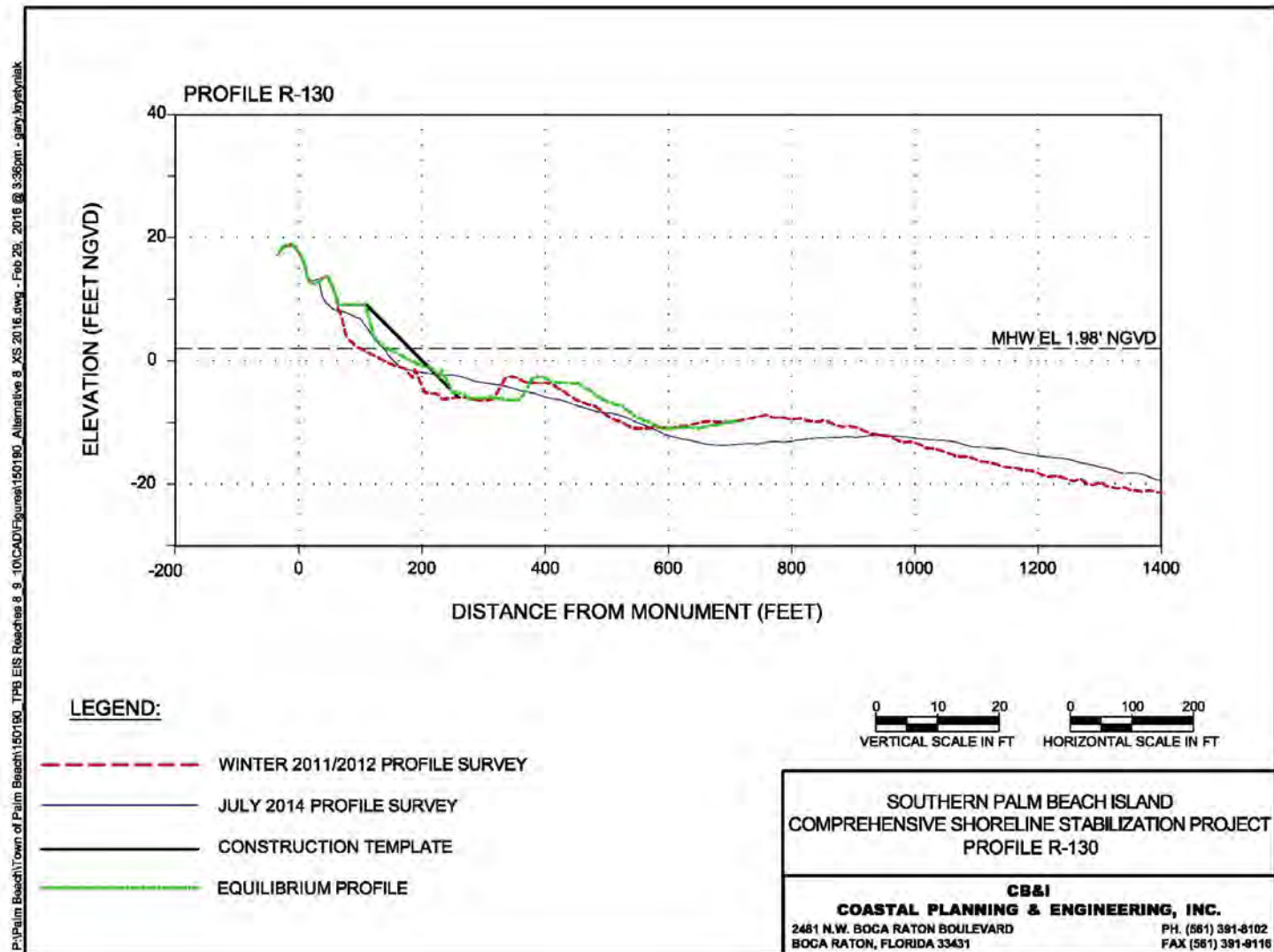
Figure 52. Alternative 7b Profile R-130.
