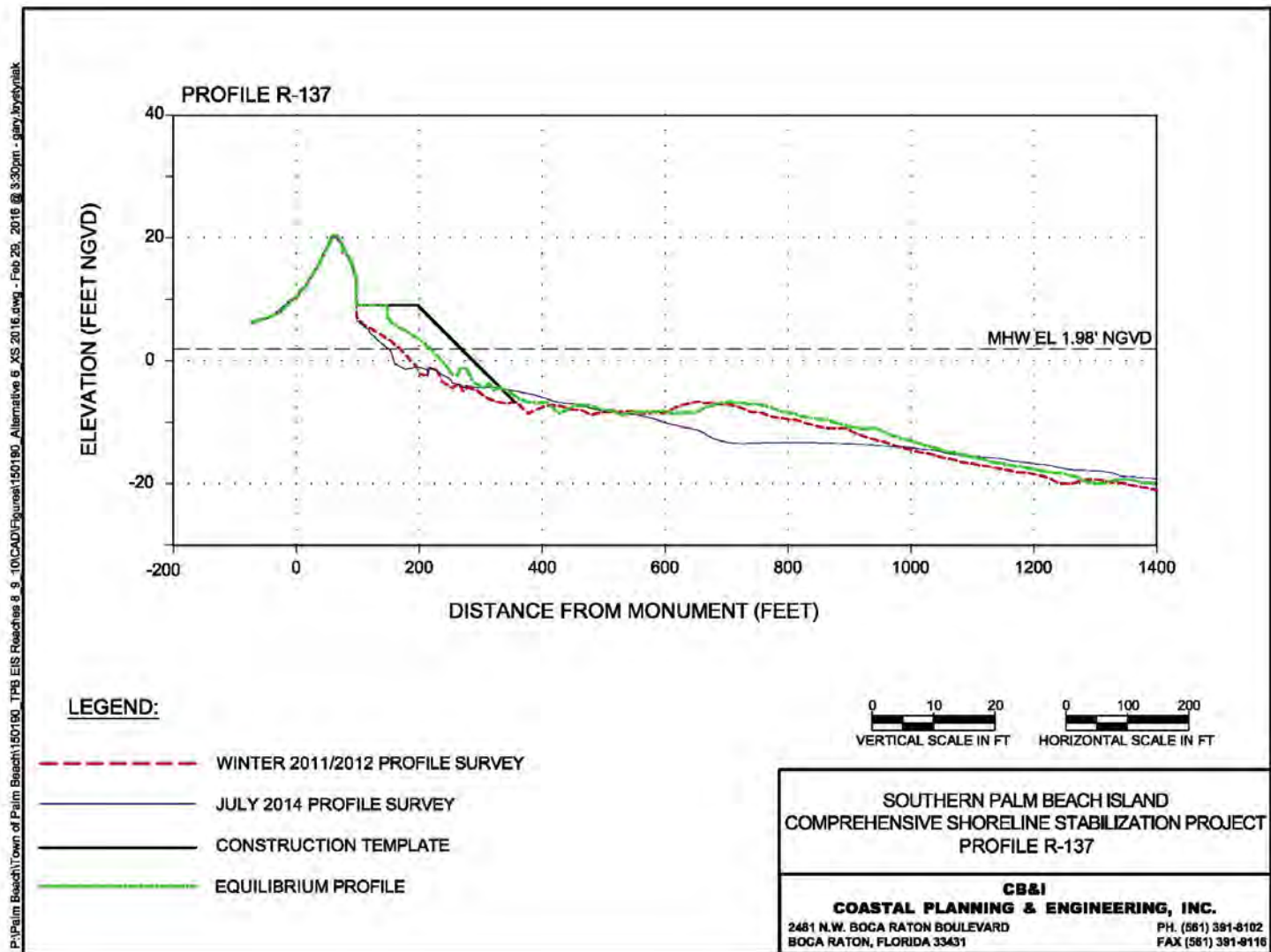
Figure 39. Alternative 6 Profile R-137.
