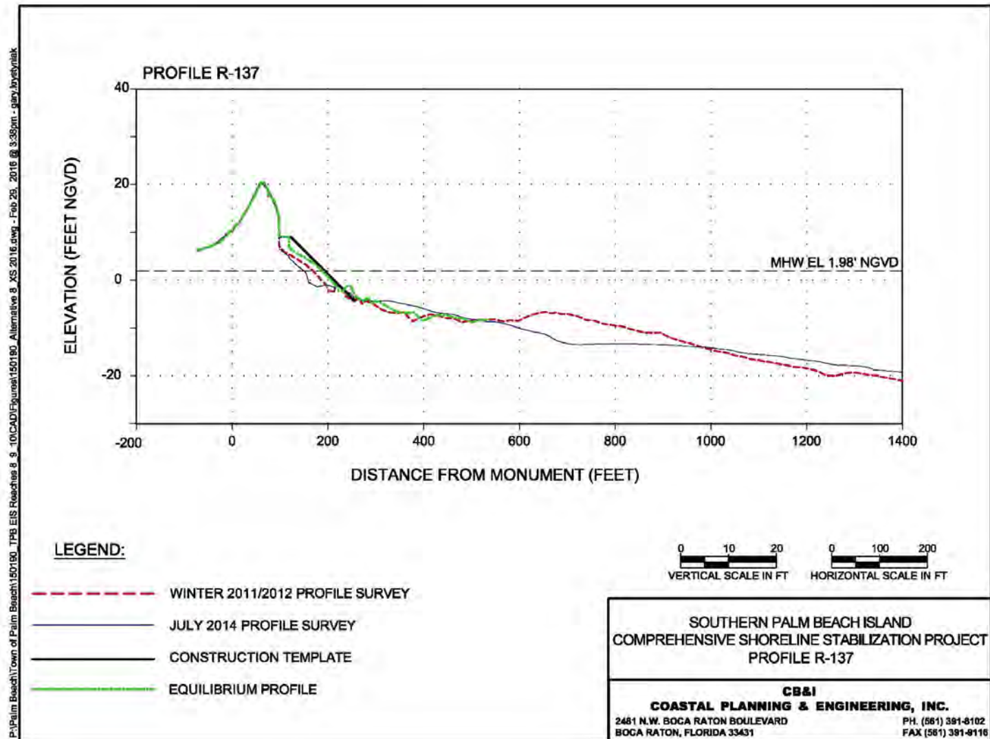
Figure 59. Alternative 7b Profile R-137.
