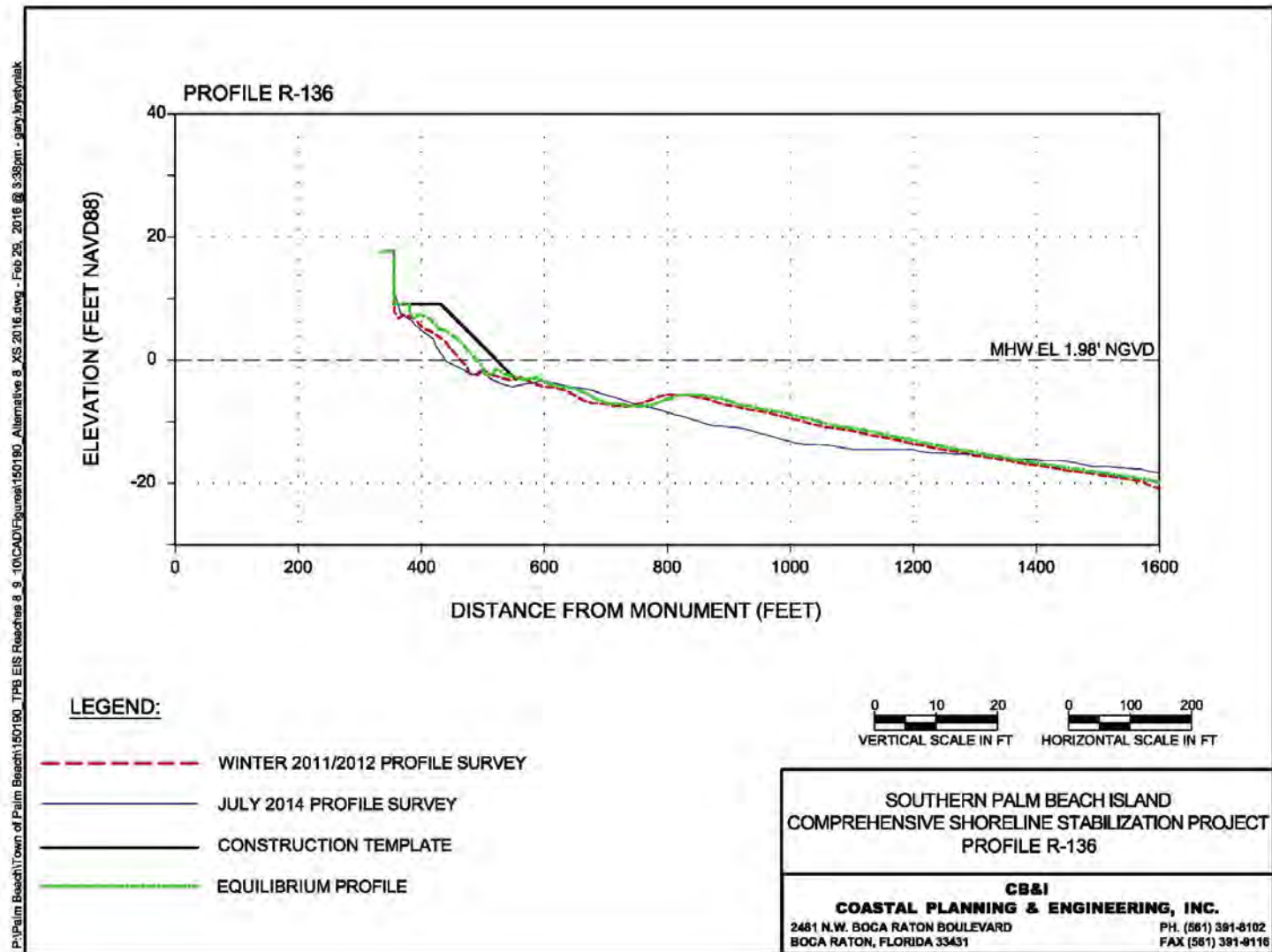
Figure 58. Alternative 7b Profile R-136.
