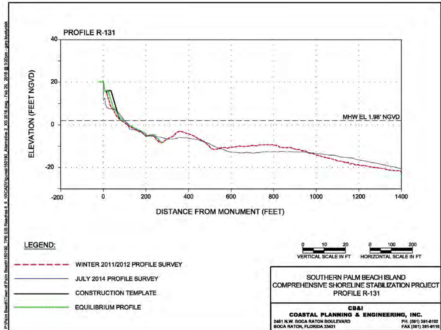
Figure 13. Alternative 4 Profile R-131.
