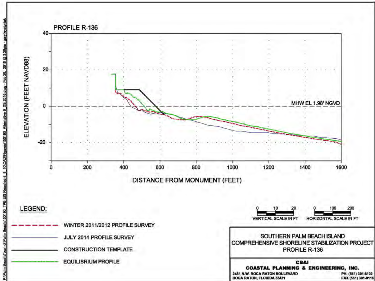
Figure 38. Alternative 6 Profile R-136.
