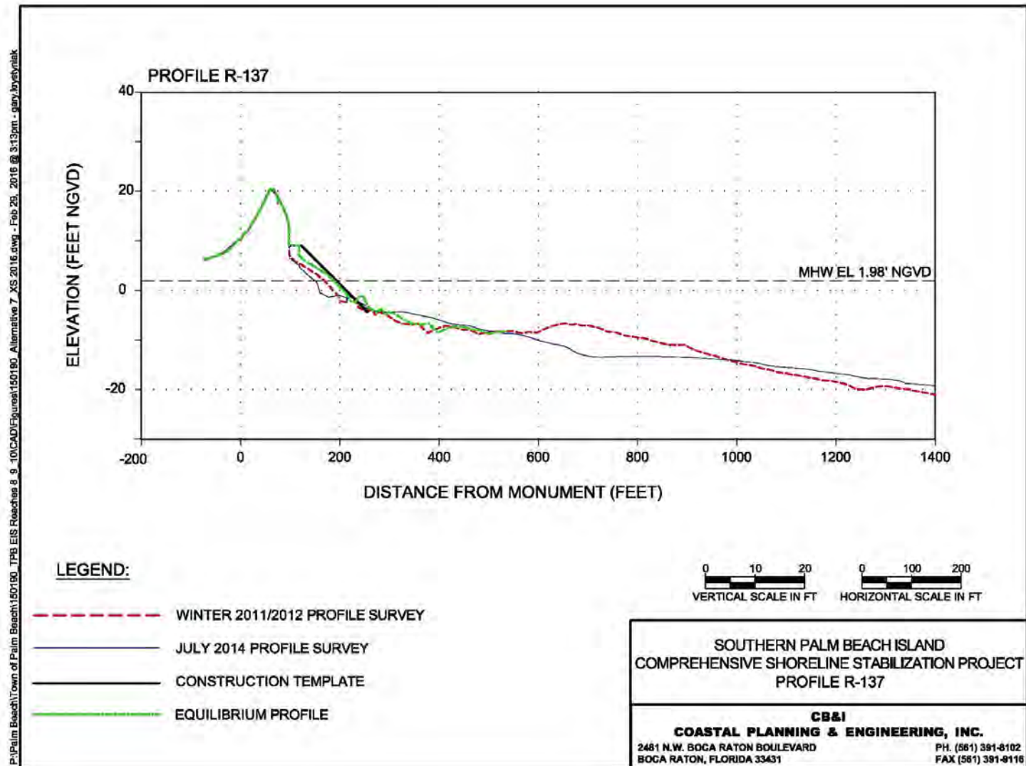
Figure 49. Alternative 7a Profile R-137.
