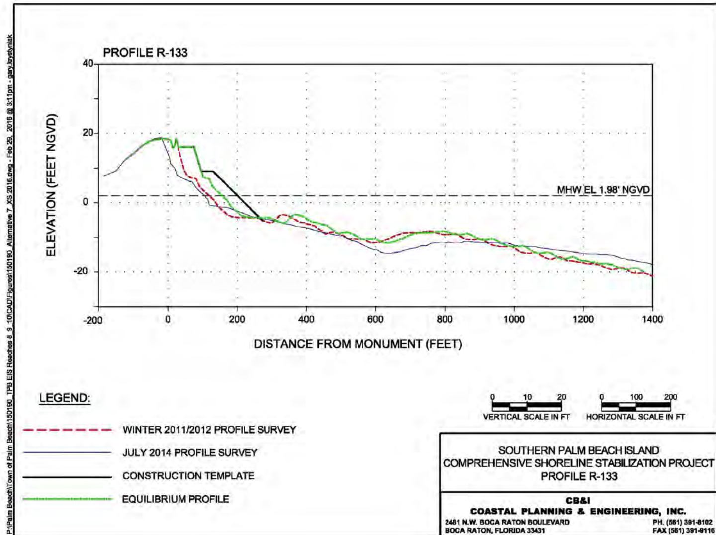
Figure 45. Alternative 7a Profile R-133.
