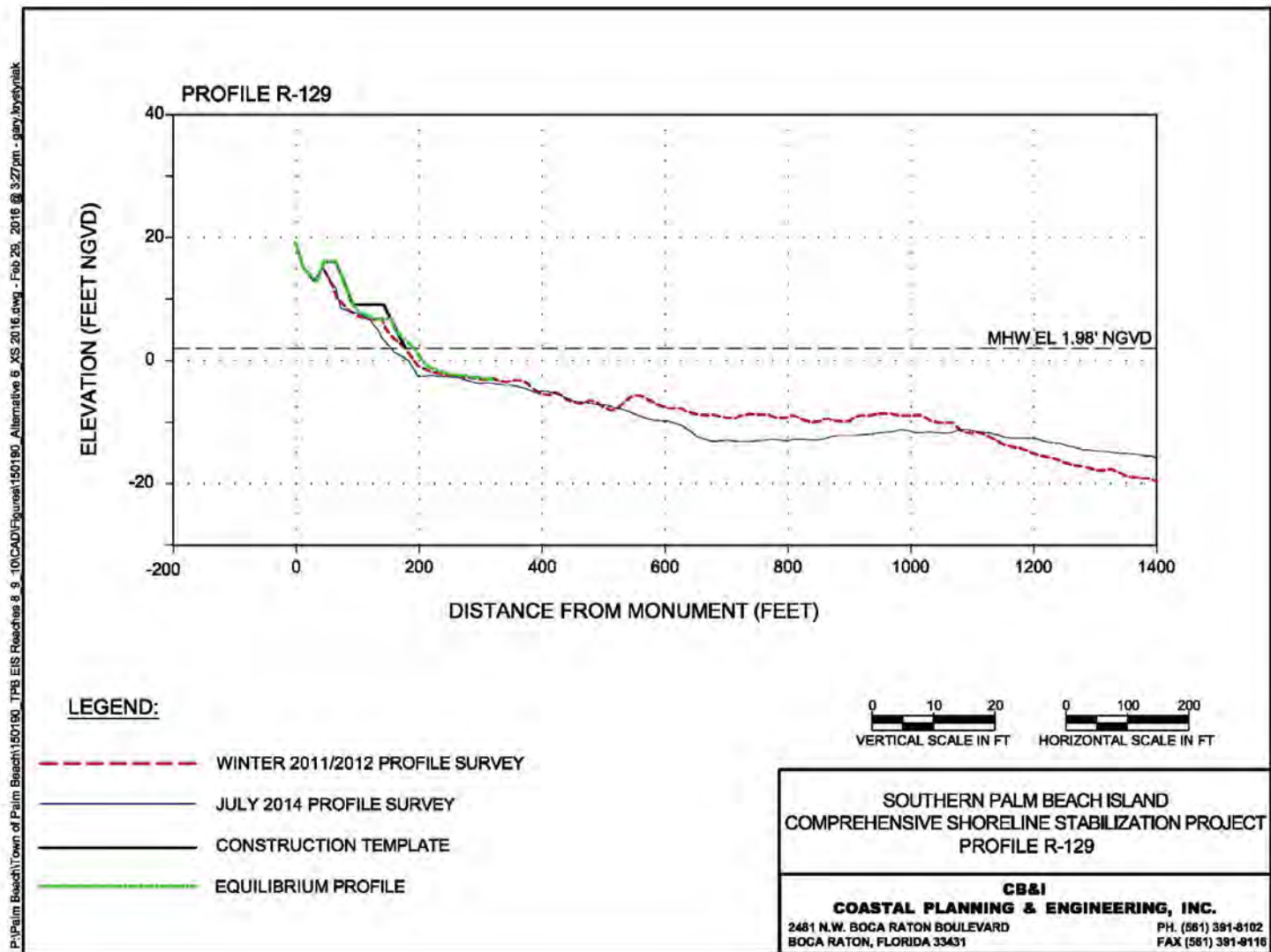
Figure 31. Alternative 6 Profile R-129.
