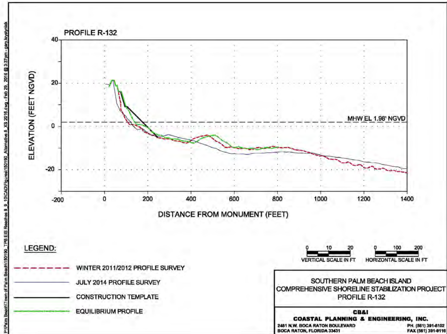
Figure 54. Alternative 7b Profile R-132.
