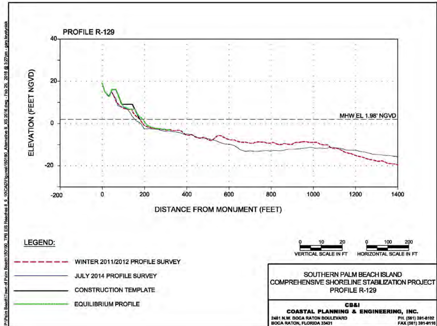
Figure 21. Alternative 5 Profile R-129.
