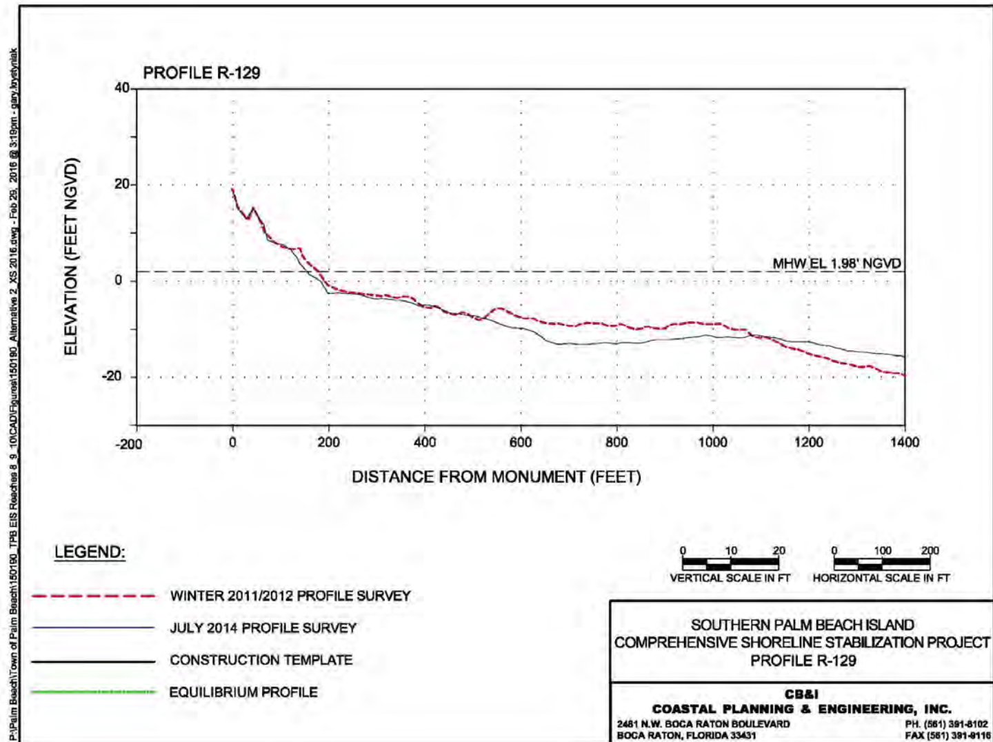
Figure 11. Alternative 4 Profile R-129.
