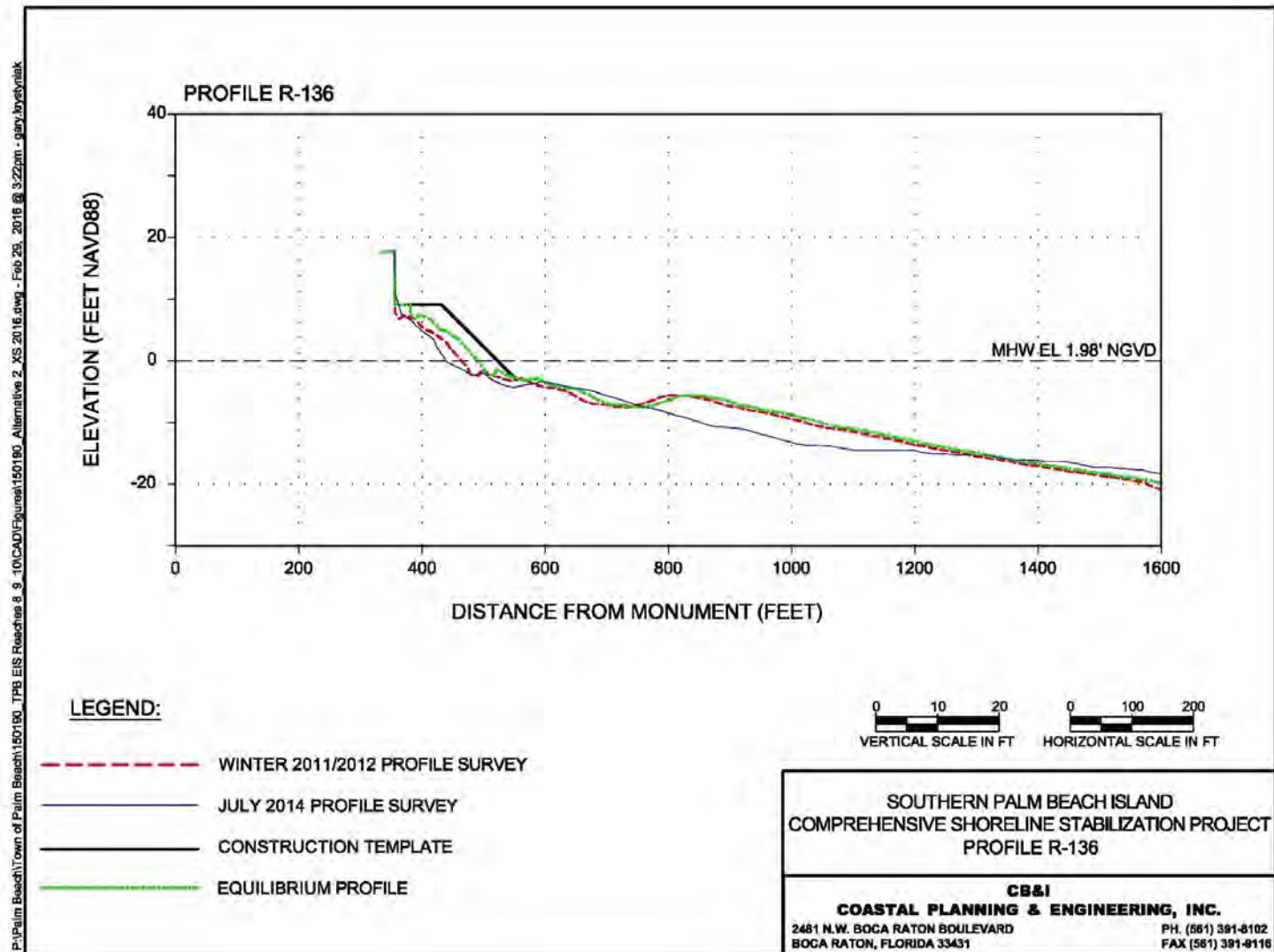
Figure 8. Alternative 2/Alternative 3 Profile R-136.
