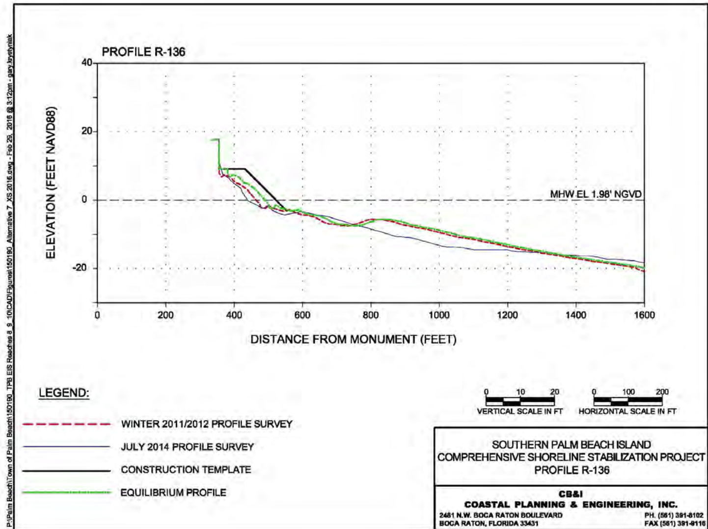
Figure 48. Alternative 7a Profile R-136.
