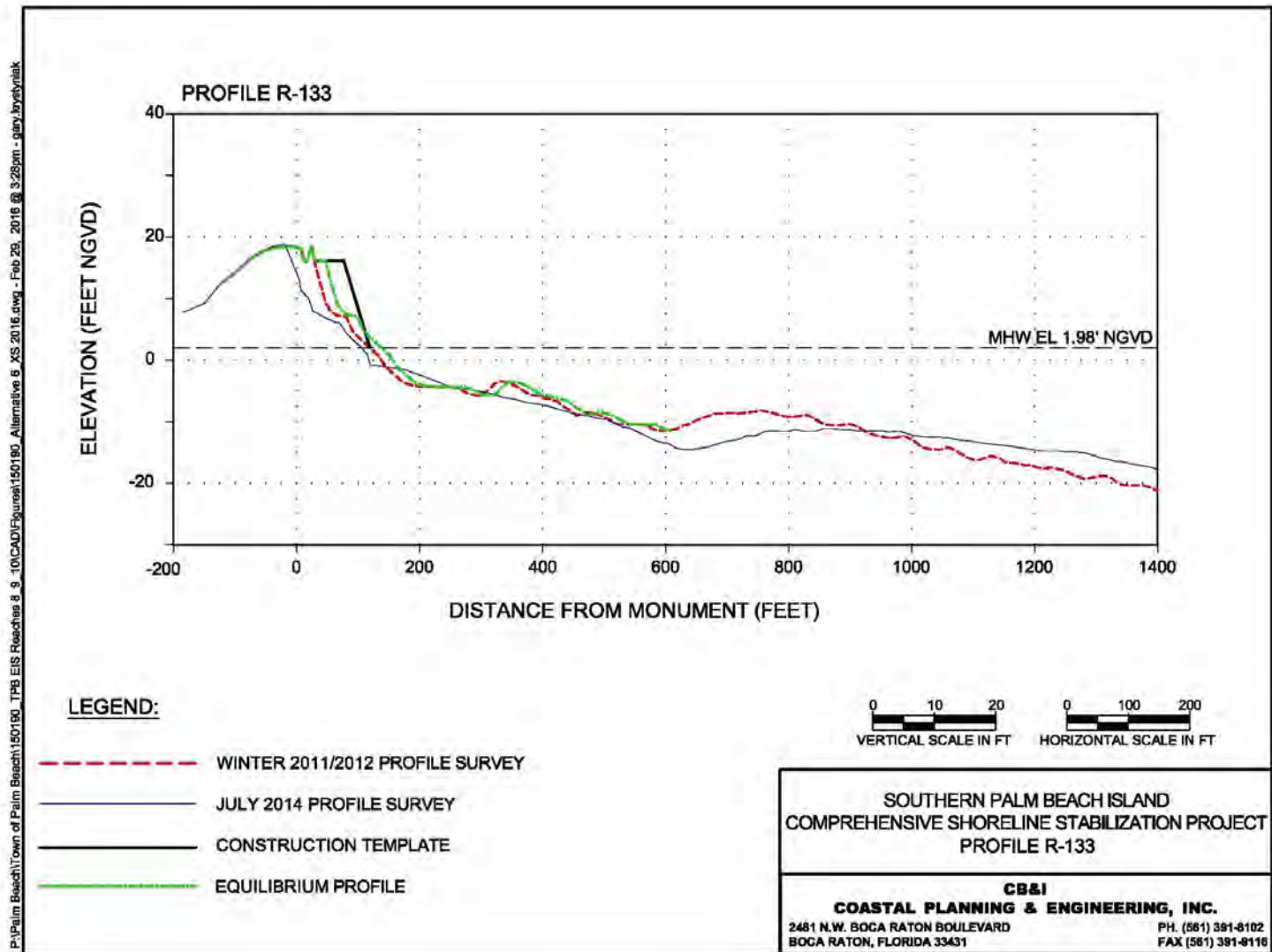
Figure 35. Alternative 6 Profile R-133.
