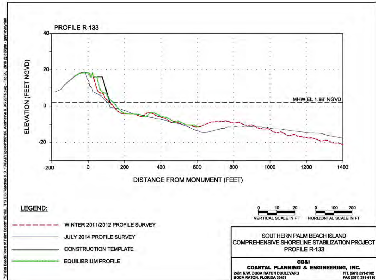
Figure 25. Alternative 5 Profile R-133.
