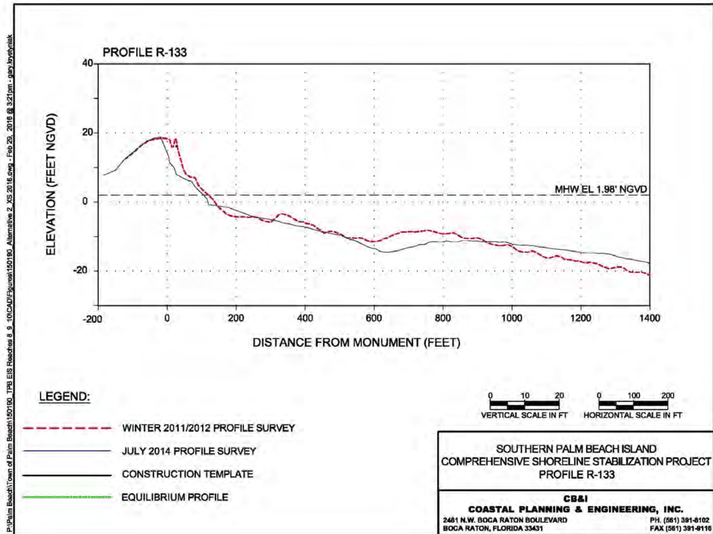
Figure 5. Alternative 2/Alternative 3 Profile R-133.
