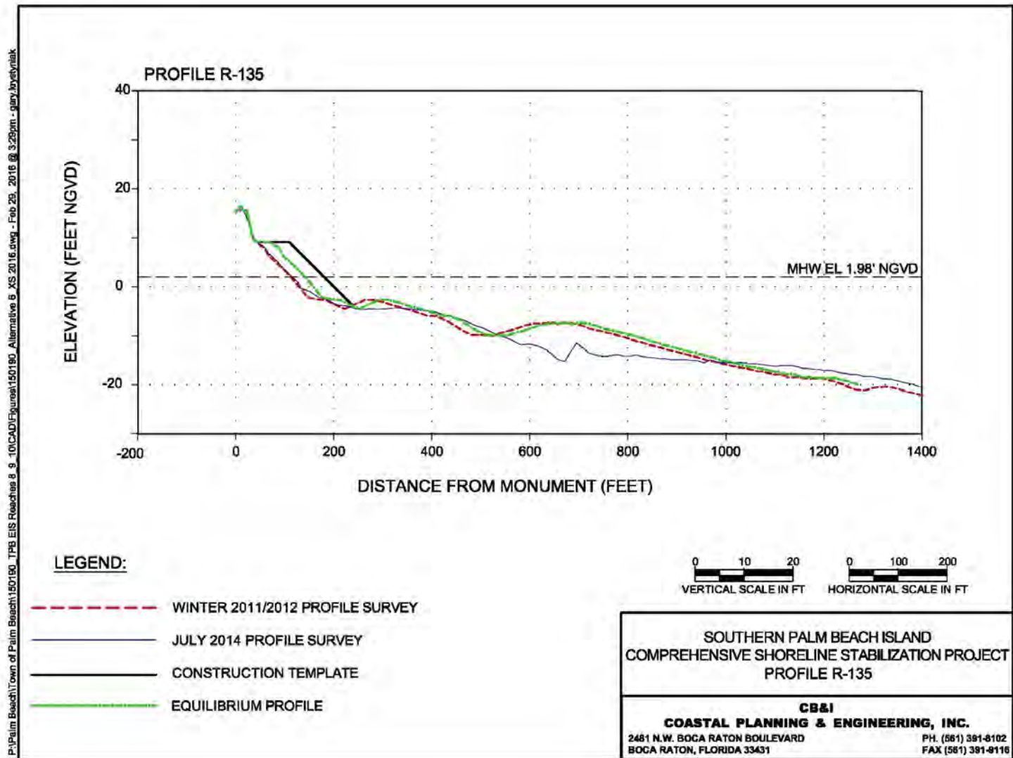
Figure 37. Alternative 6 Profile R-135.
