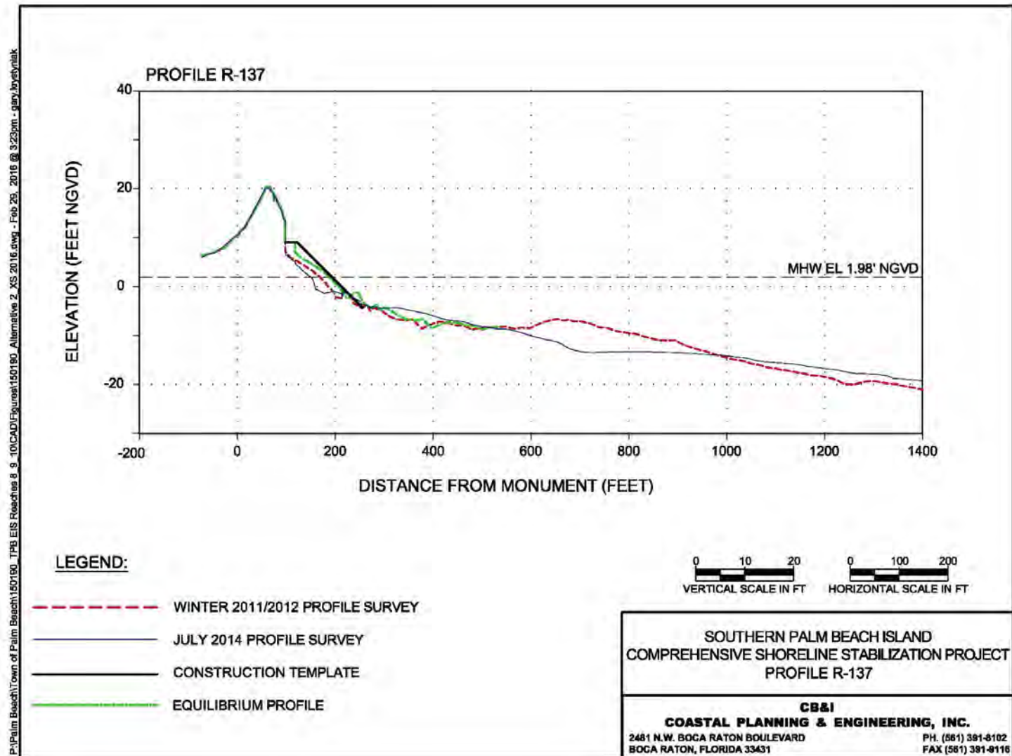
Figure 29. Alternative 5 Profile R-137.
