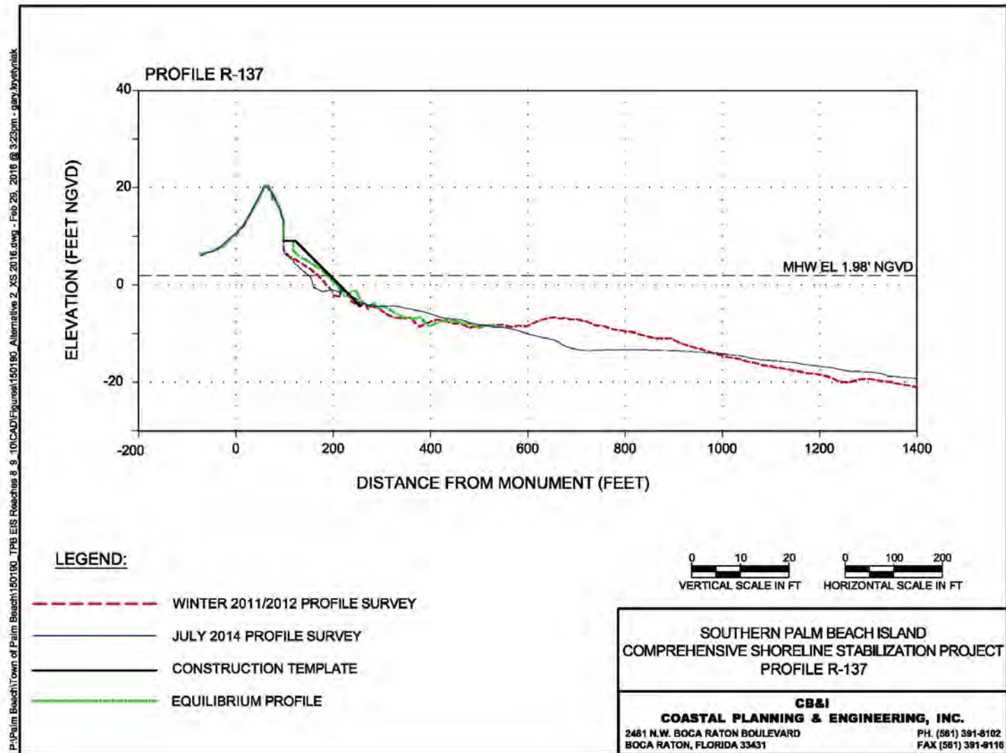
Figure 9. Alternative 2/Alternative 3 Profile R-137.
