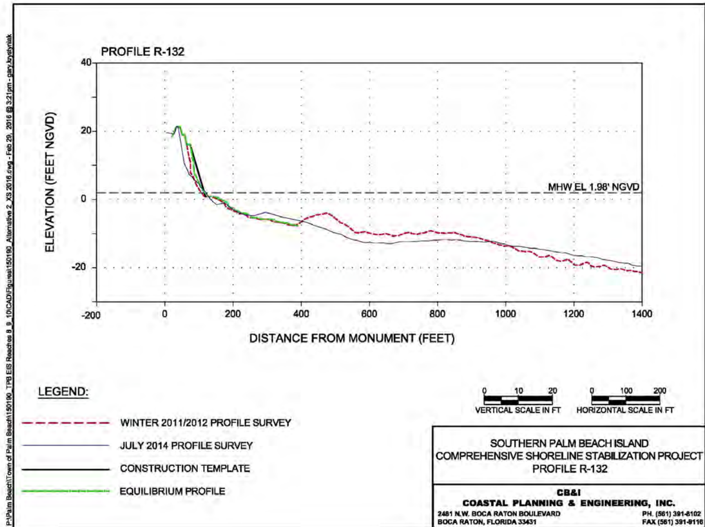
Figure 4. Alternative 2/Alternative 3 Profile R-132.
