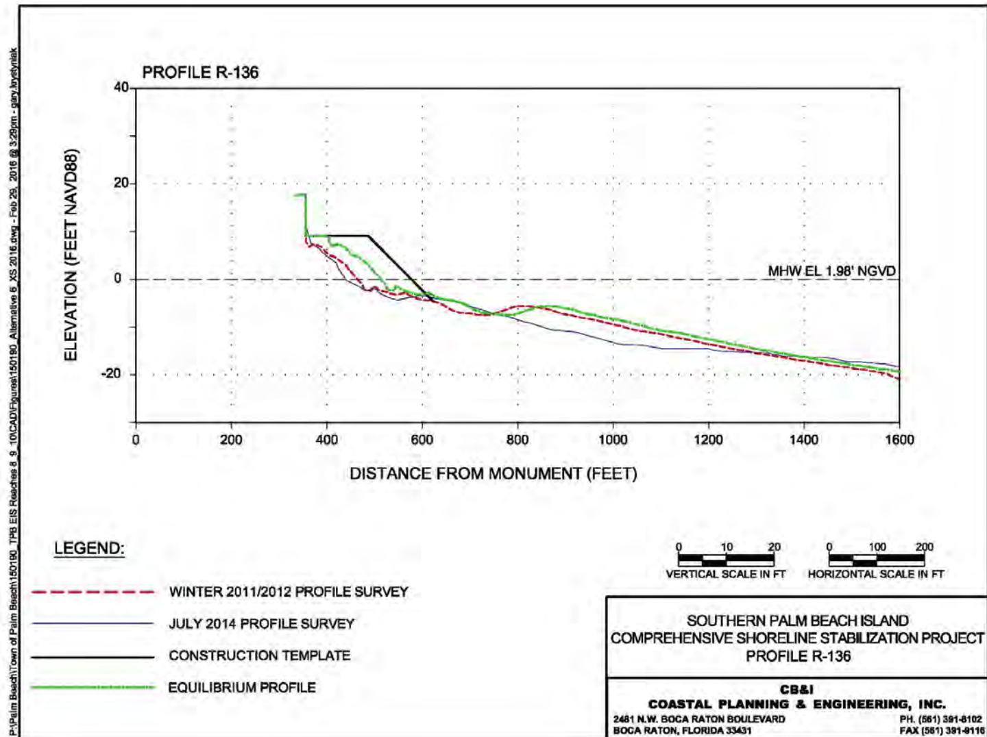
Figure 18. Alternative 4 Profile R-136.
