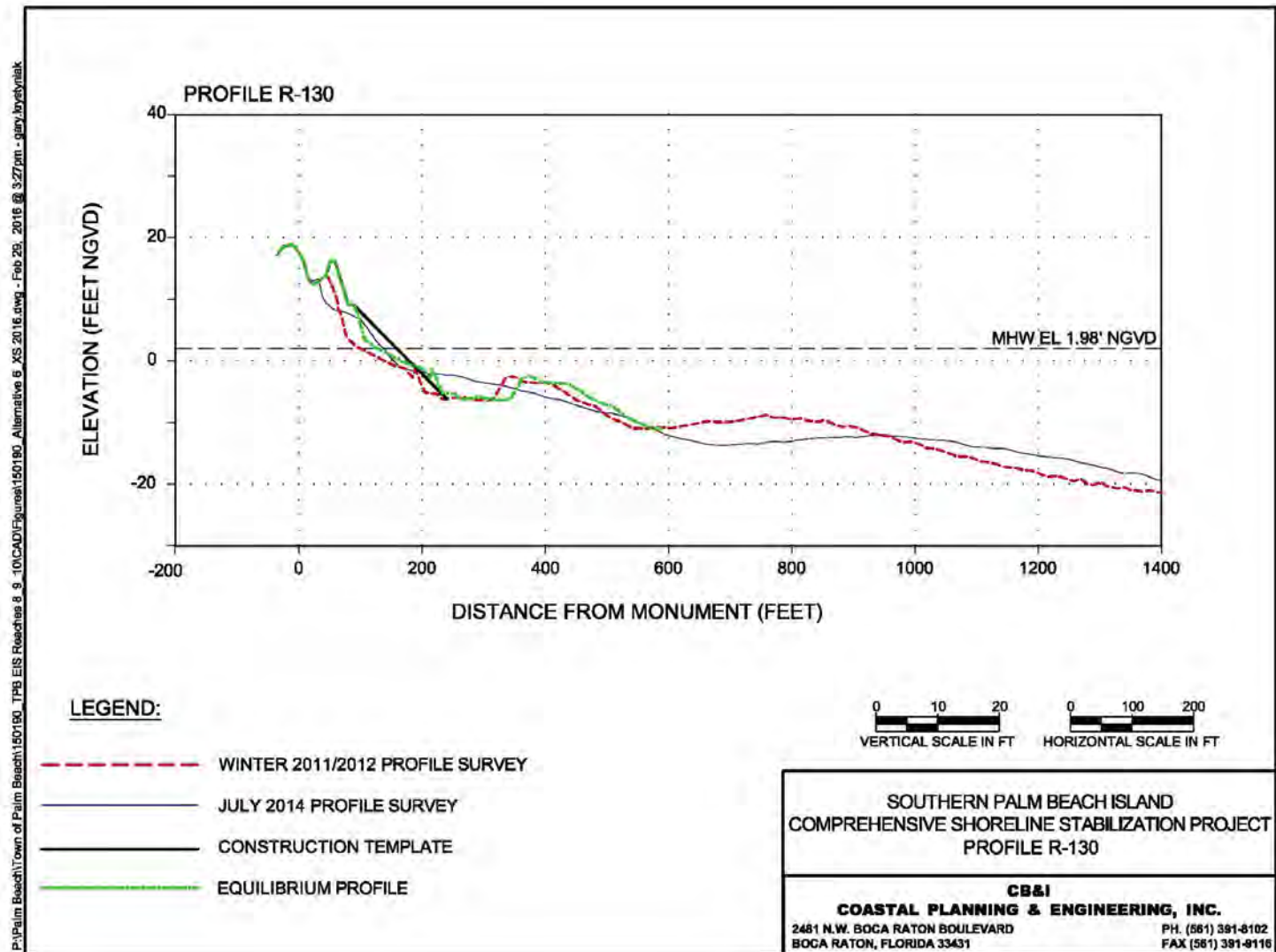
Figure 22. Alternative 5 Profile R-130.
