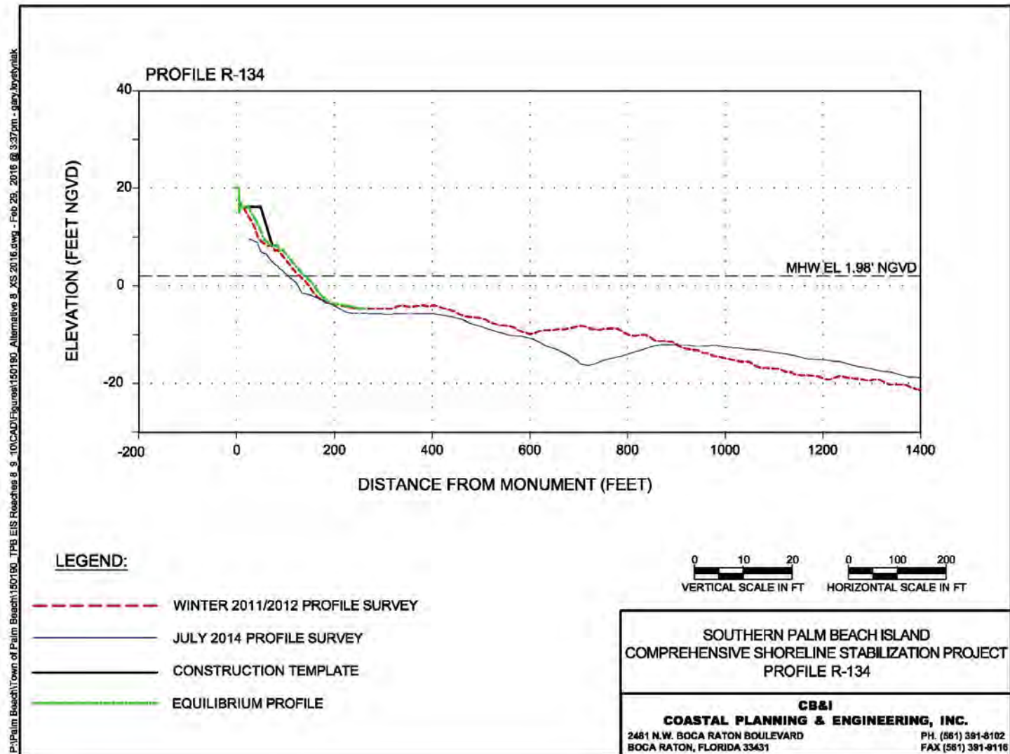
Figure 56. Alternative 7b Profile R-134.
