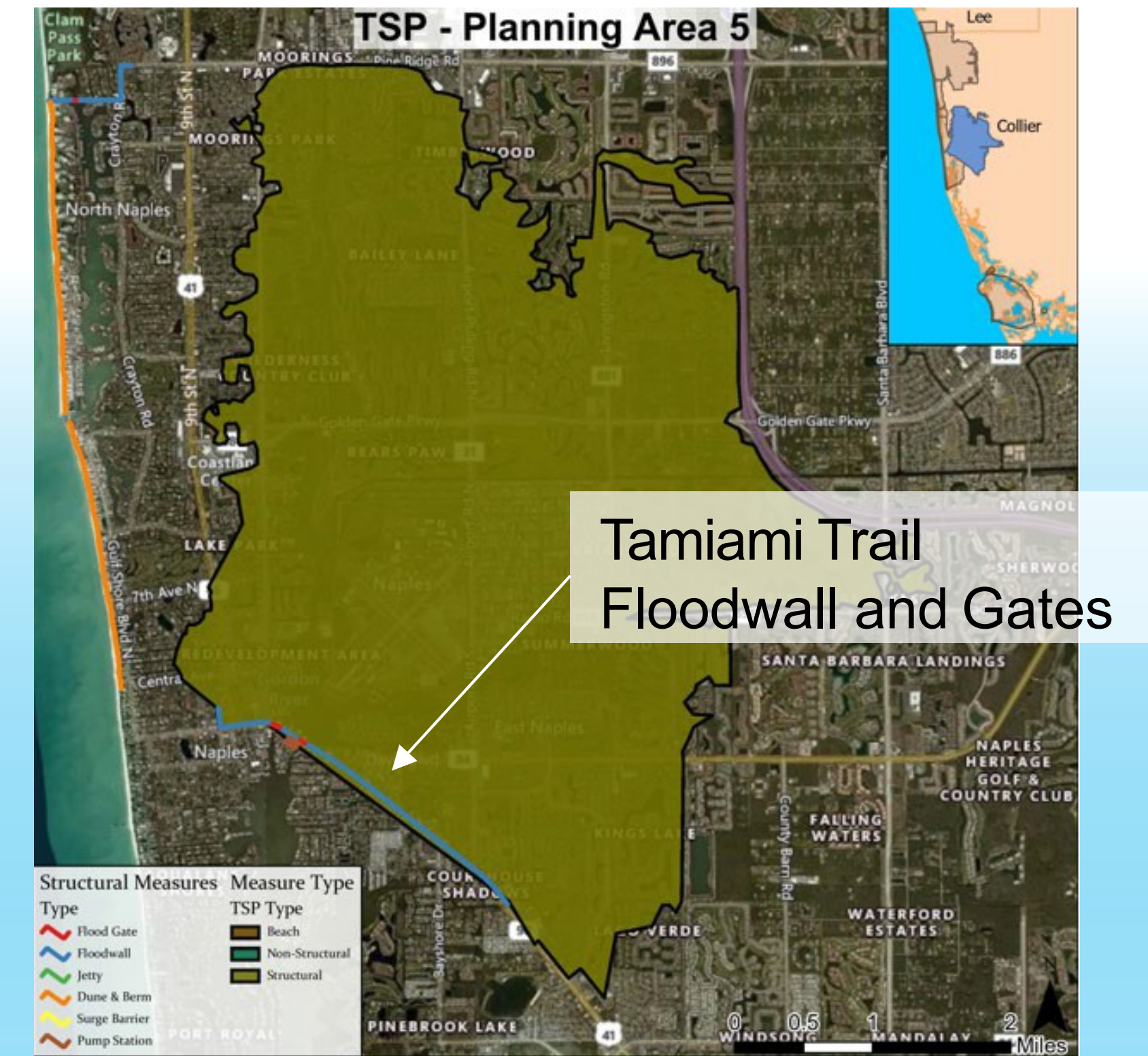
floodwalls
