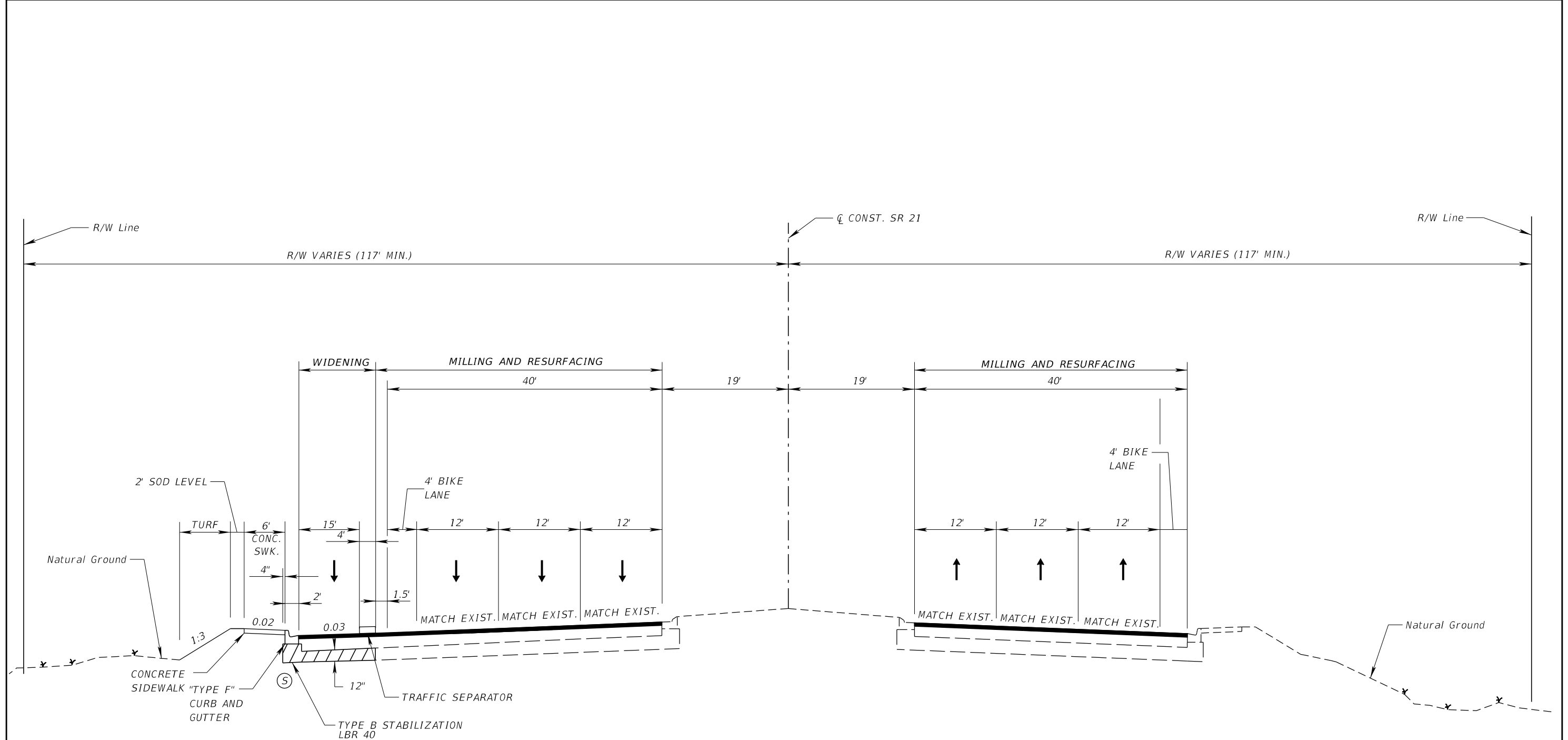
TYPICAL SECTION NO. 14 BLANDING BLVD. (SR 21) STA. 1382+46.79 TO STA. 1411+06.74
