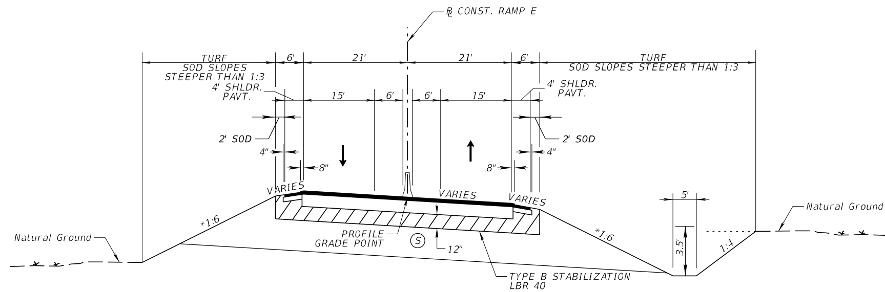
TYPICAL SECTION NO. 18 RAMP E
