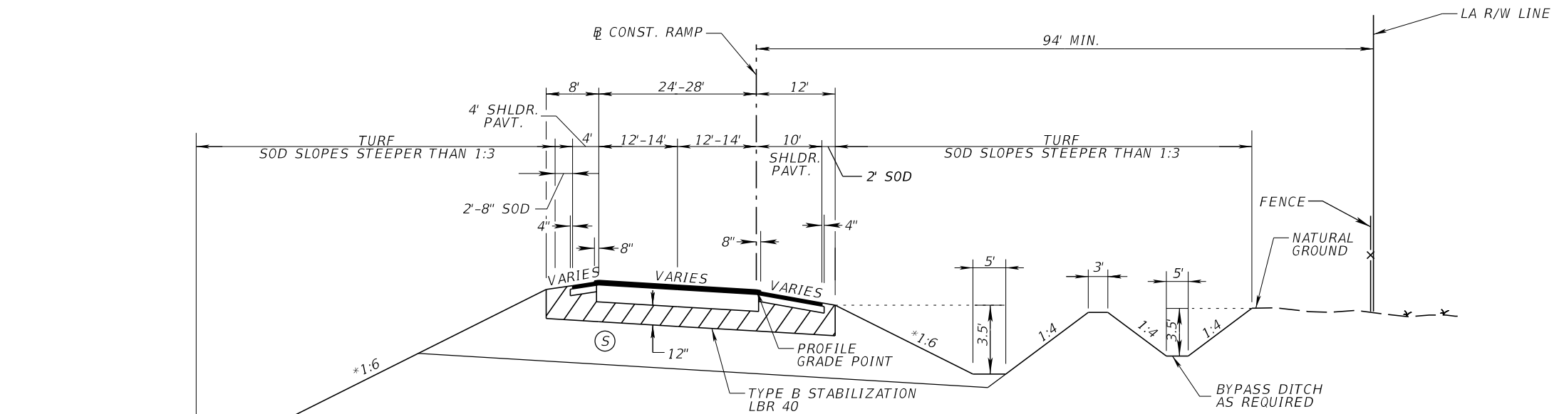
TYPICAL SECTION NO. 19 (TWO LANE RAMP) RAMP C, D, E, F, G, H, I, J, L, M, N-3, O-2, P, Q, R, S, T, U, V, W, X, Y, X, AA, CC AND DD
