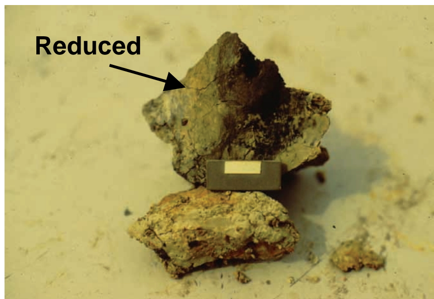
Figure 54. This soil exhibits colors associated with reducing conditions. Scale is 1 cm.
