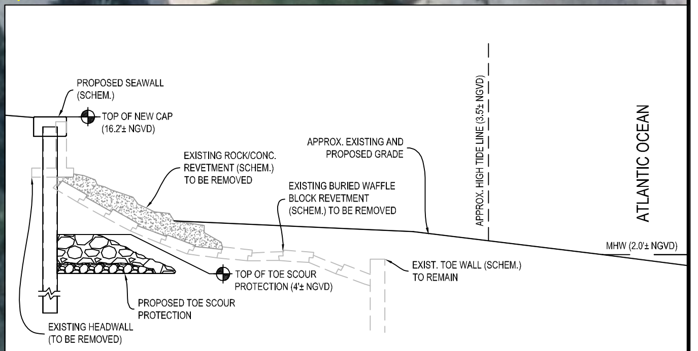
SECTION A-A 0 5 10 SCALE IN FEET 1"=10'
