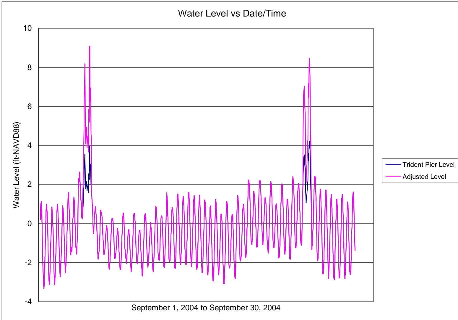
Figure 12. Water Levels – R77 to R84 – Measured (Trident Pier) and Adjusted (August 30, 2004 to September 30, 2004)
