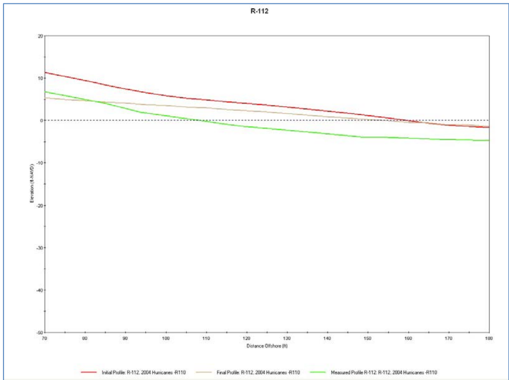
Figure 28. SBEACH Verification Run (2004 Storm Event), R-112 (Dune to Waterline)
