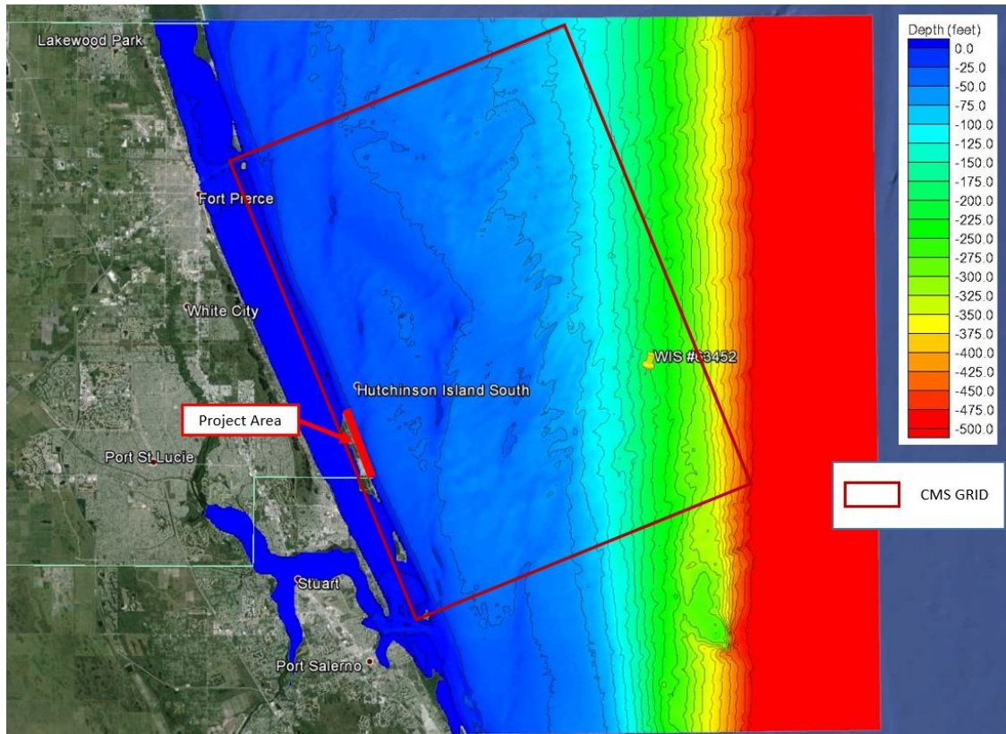
Figure 5-16. CMS Modeling Grid Layout
