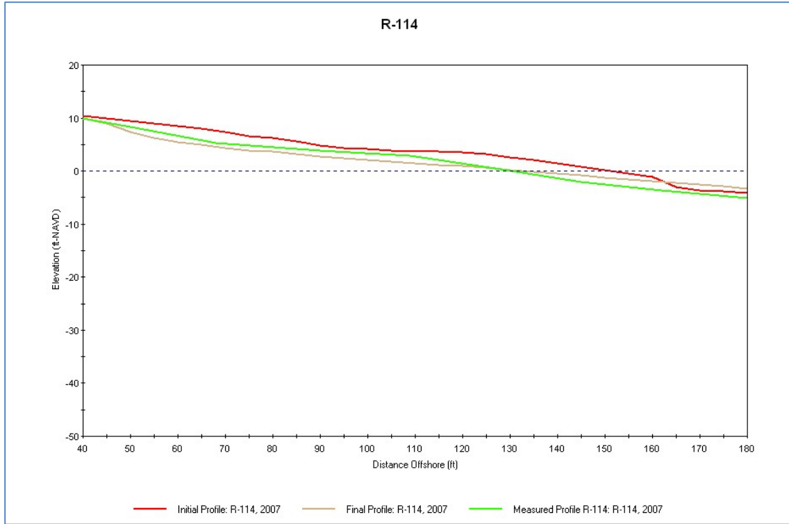
Figure 35. SBEACH Verification Run (2007 Storm Event), R-114 (Dune to Waterline)
