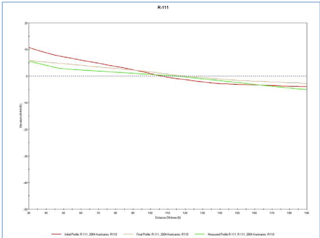
Figure 27. SBEACH Verification Run (2004 Storm Event), R-111 (Dune to Waterline)
