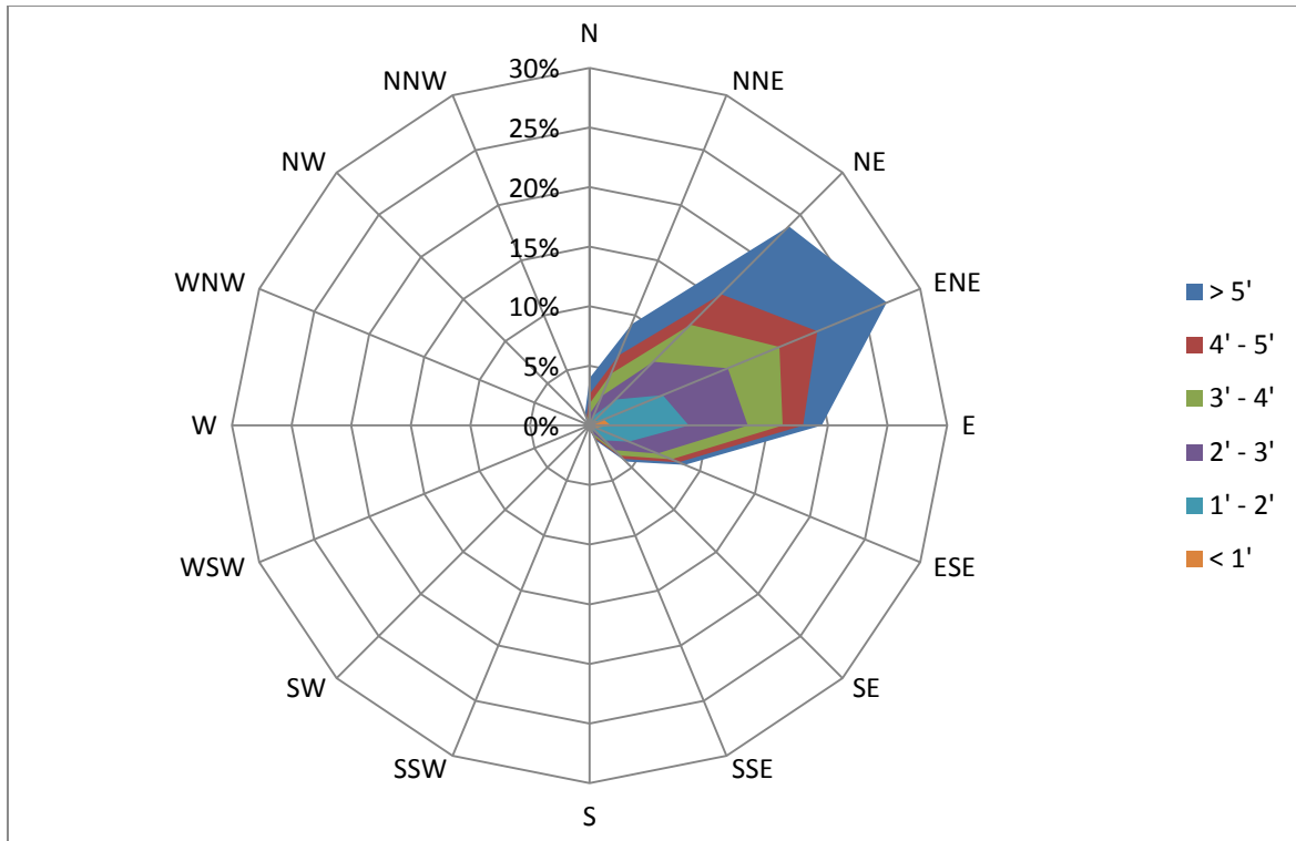
Figure 3-4. Wave Rose – WIS Station 63452
