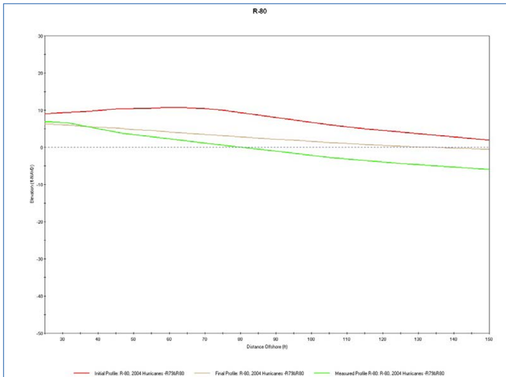
Figure 14. SBEACH Calibration Run (2004 Storm Event), R-80 (Dune to Waterline)
