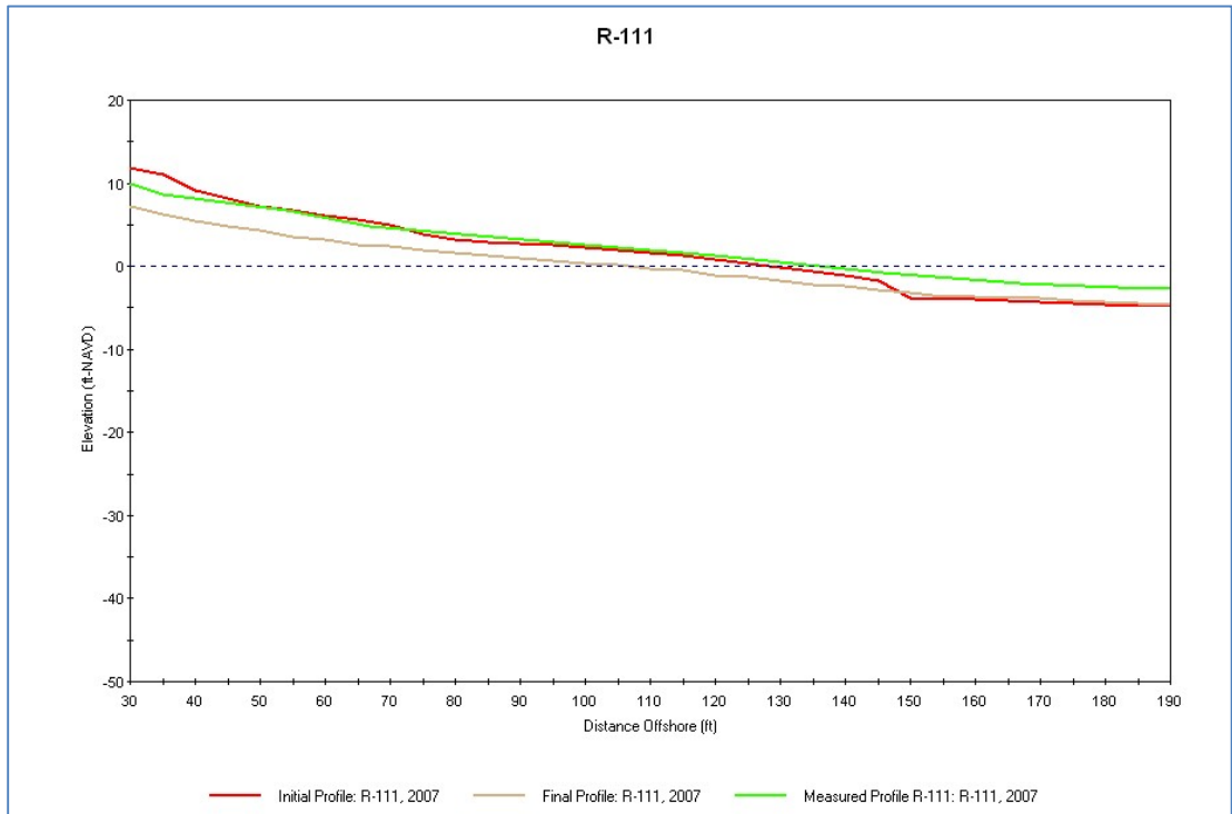
Figure 32. SBEACH Verification Run (2007 Storm Event), R-111 (Dune to Waterline)
