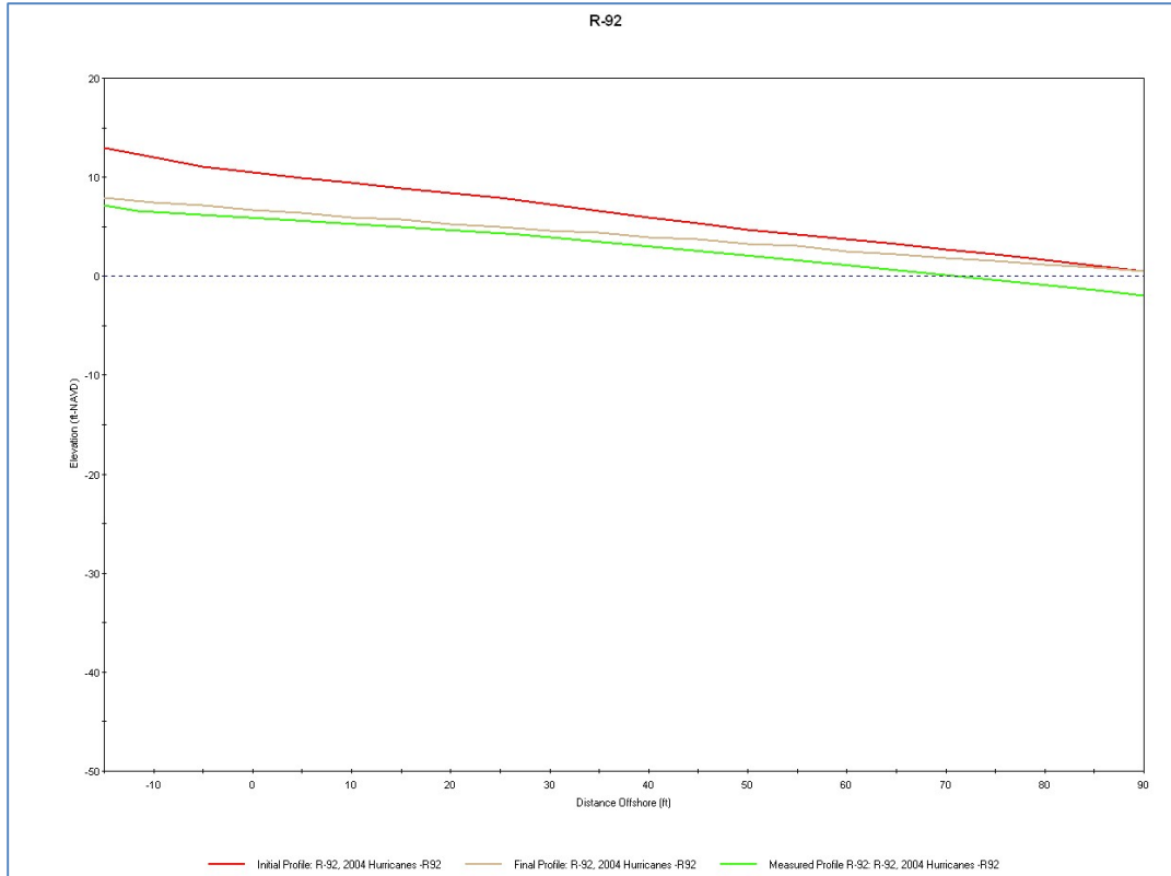
Figure 17. SBEACH Calibration Run (2004 Storm Event), R-92 (Dune to Waterline)
