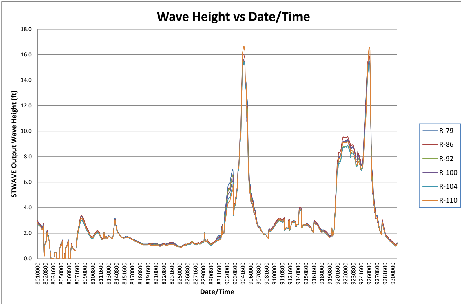
Figure 11. STWAVE Wave Heights (August 1, 2004 to September 30, 2004)
