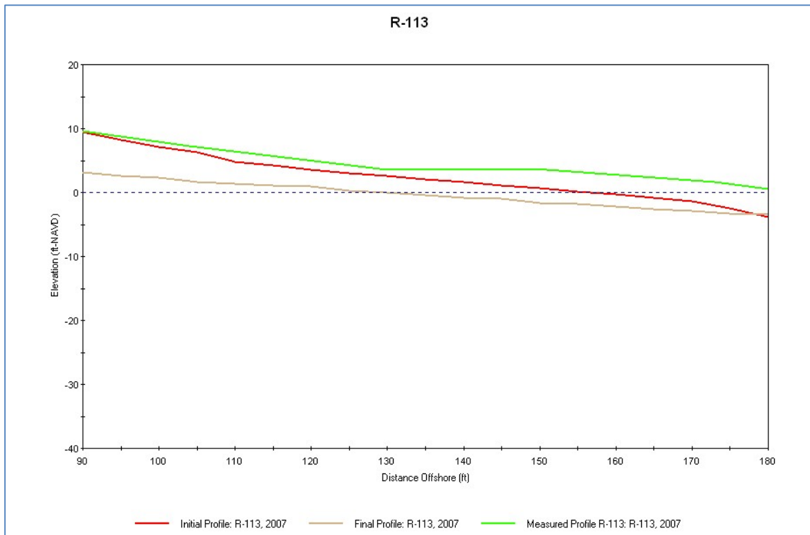
Figure 34. SBEACH Verification Run (2007 Storm Event), R-113 (Dune to Waterline)
