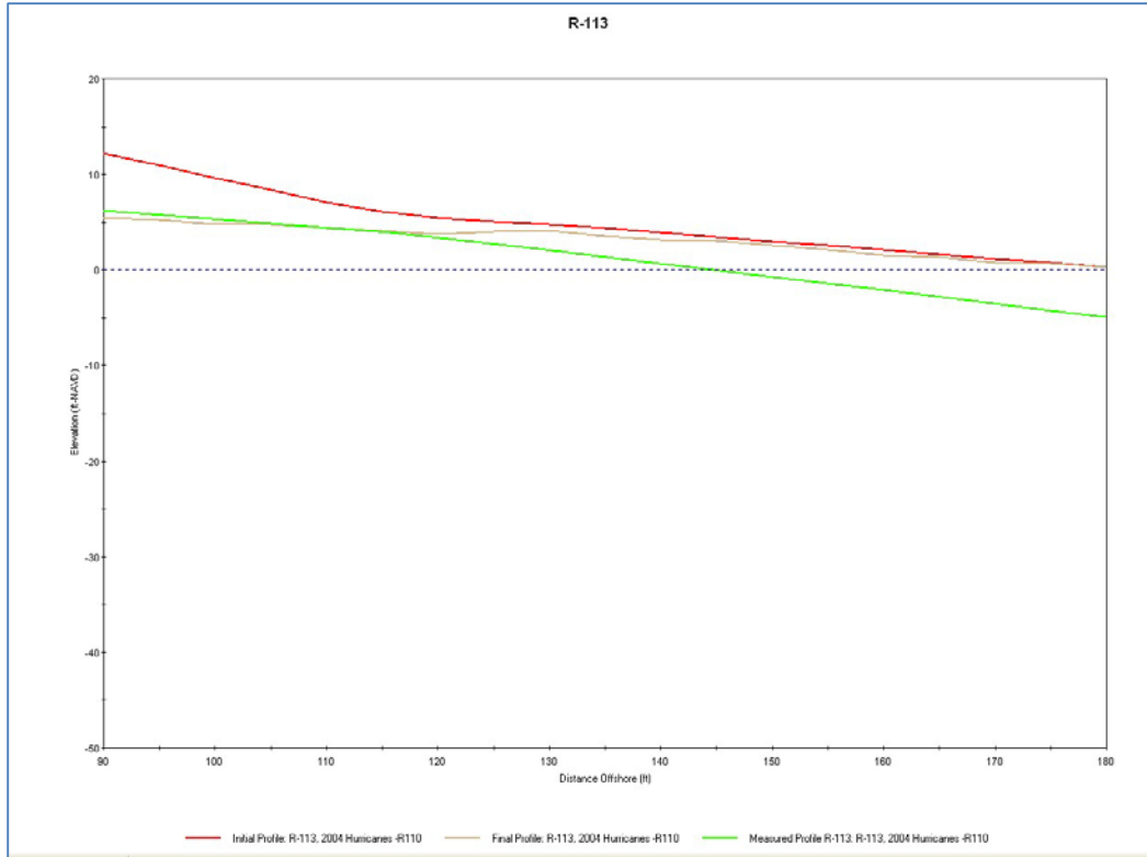
Figure 29. SBEACH Verification Run (2004 Storm Event), R-113 (Dune to Waterline)
