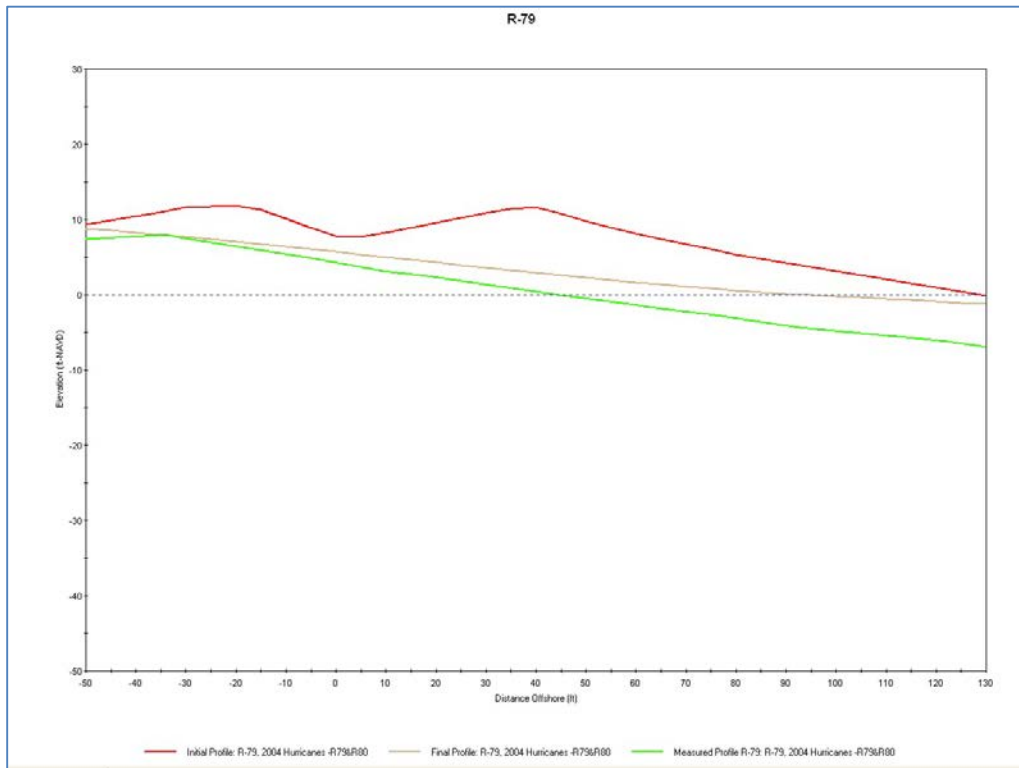
Figure 13. SBEACH Calibration Run (2004 Storm Event), R-79 (Dune to Waterline)
