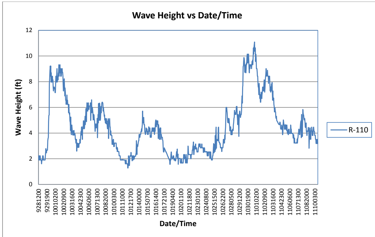
Figure 26. STWAVE Wave Heights (September 28, 2007 to November 10, 2007)
