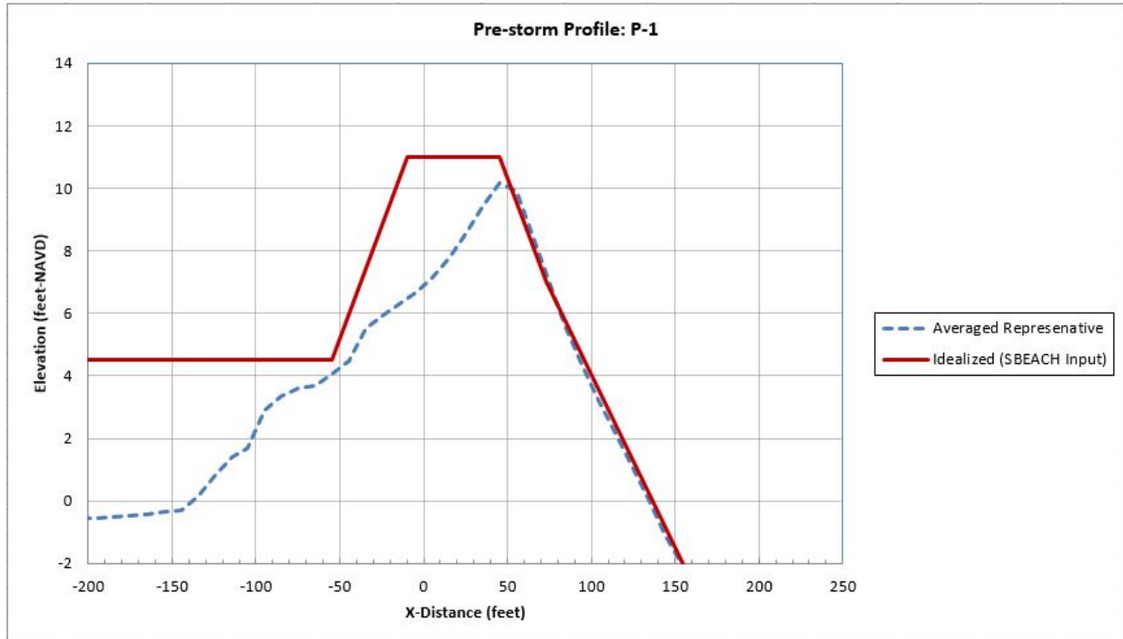
Figure 5-5. Average Measured and Idealized Beach-fx Profiles: P1 Grouping
