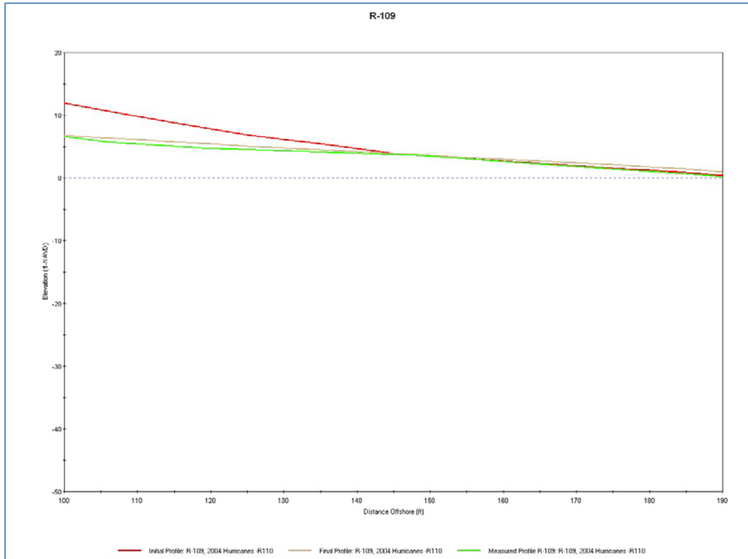
Figure 20. SBEACH Calibration Run (2004 Storm Event), R-109 (Dune to Waterline)
