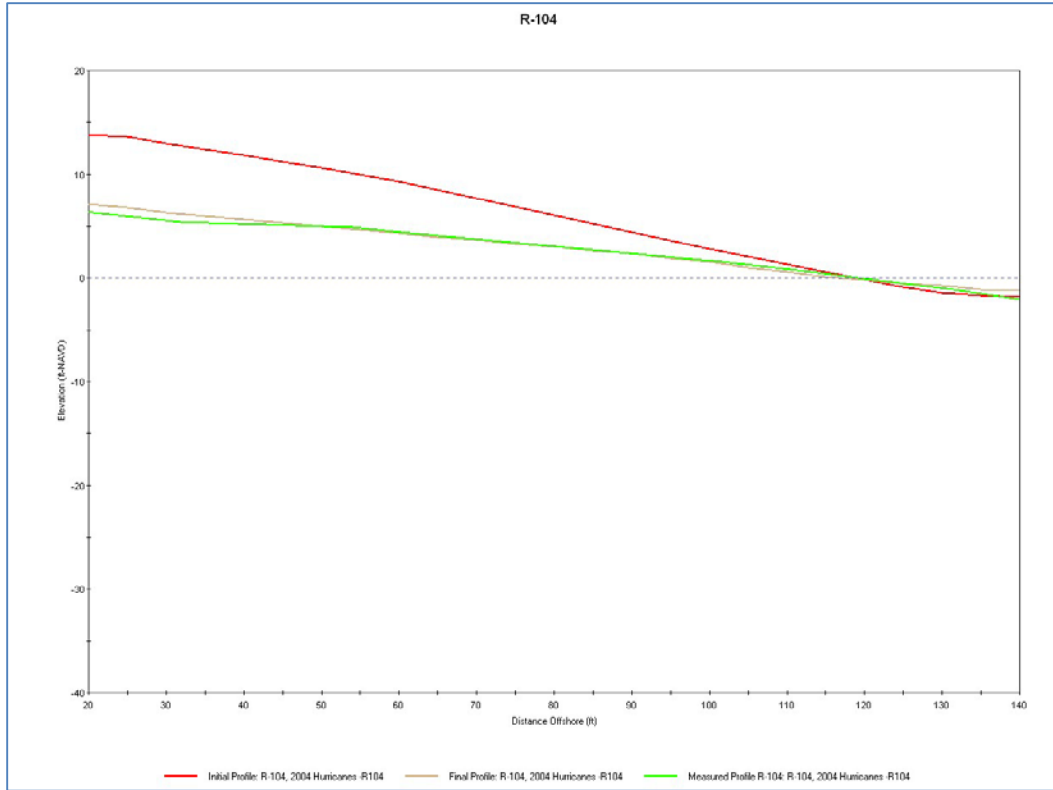
Figure 19. SBEACH Calibration Run (2004 Storm Event), R-104 (Dune to Waterline)
