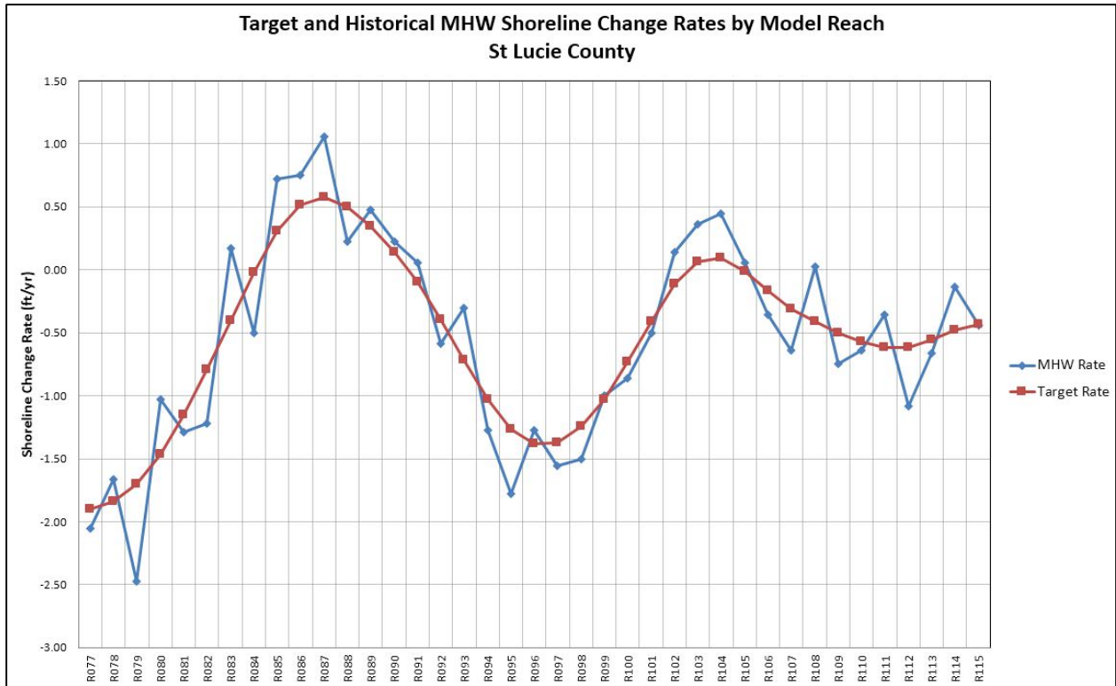
Figure 5-14. Target MHW Shoreline Change Rate
