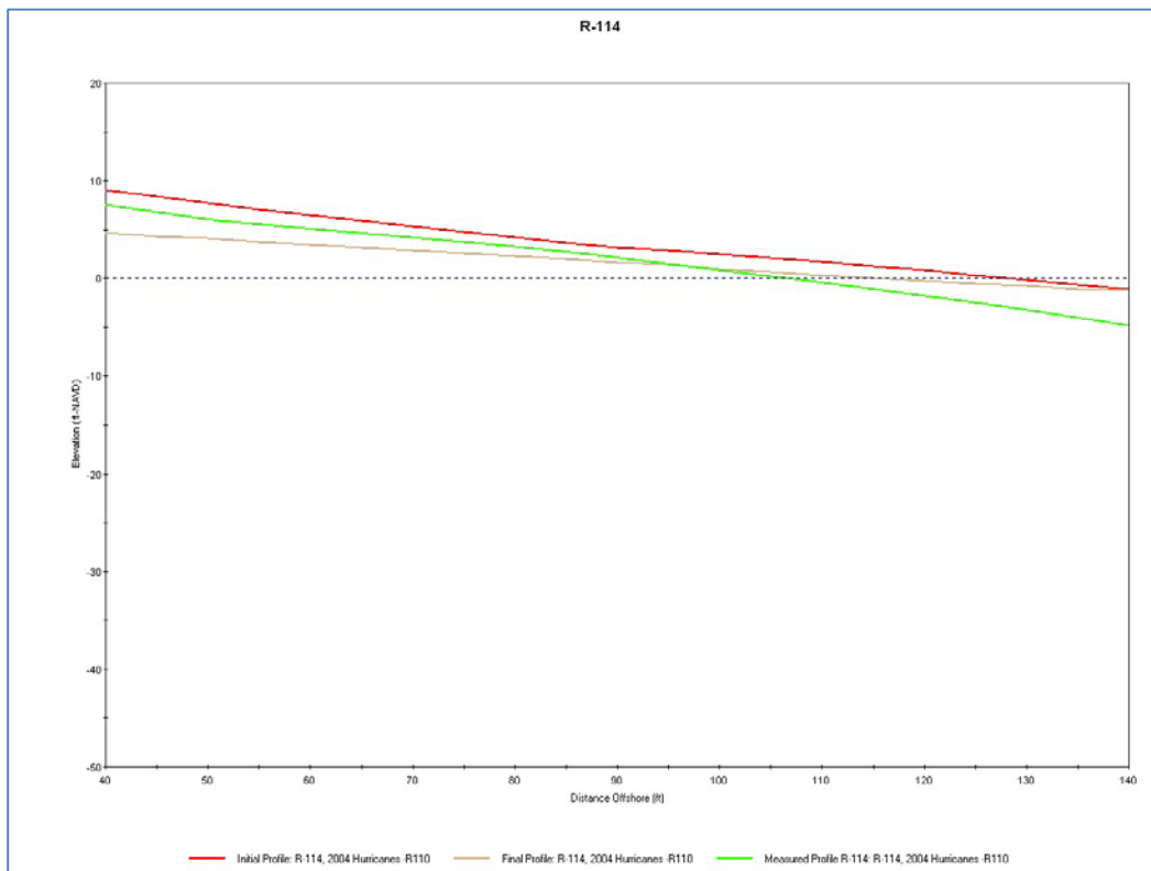
Figure 30. SBEACH Verification Run (2004 Storm Event), R-114 (Dune to Waterline)
