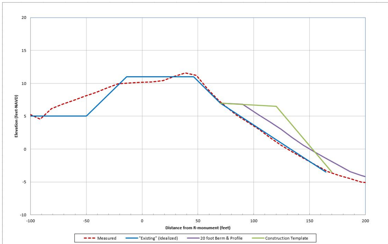
Figure 6-1. Typical Profile Sketch
