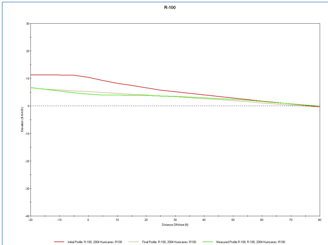
Figure 18. SBEACH Calibration Run (2004 Storm Event), R-100 (Dune to Waterline)
