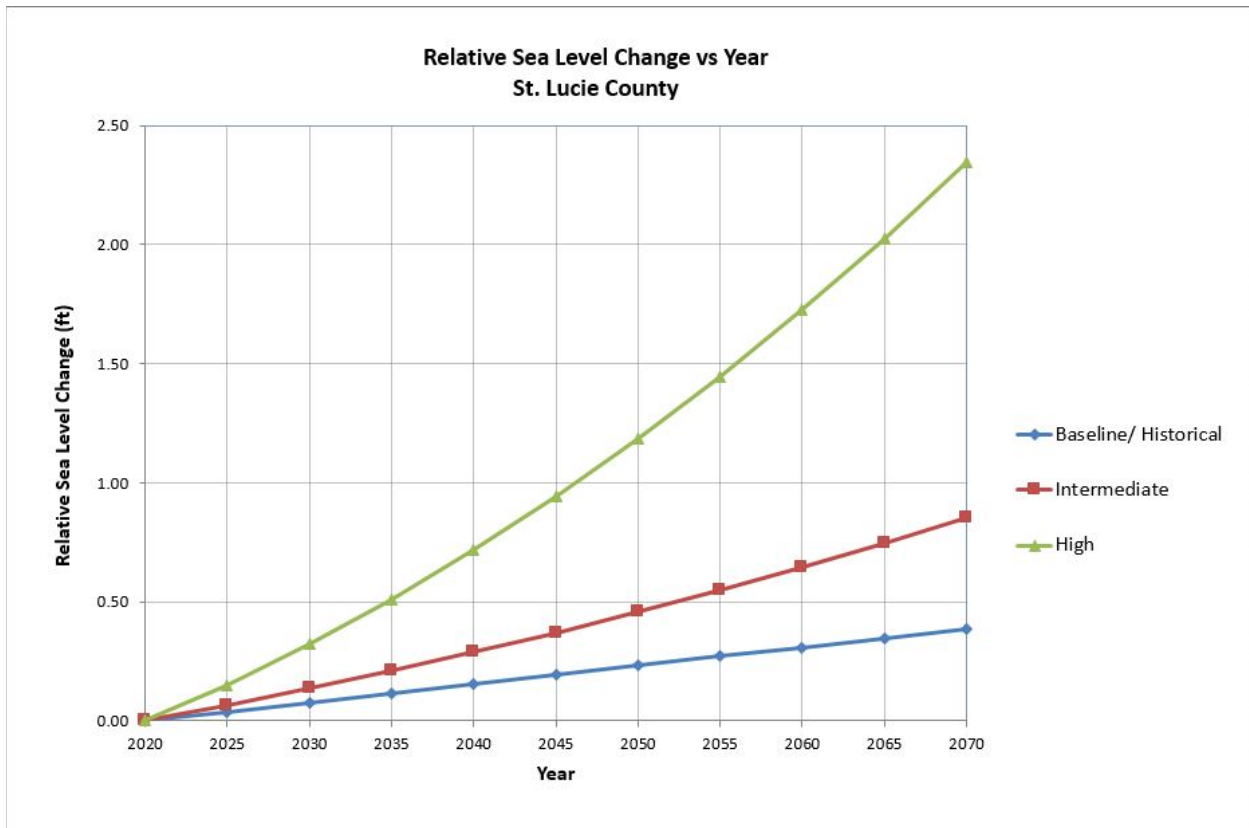
Figure 3-7. Relative Sea level Change, St. Lucie County
