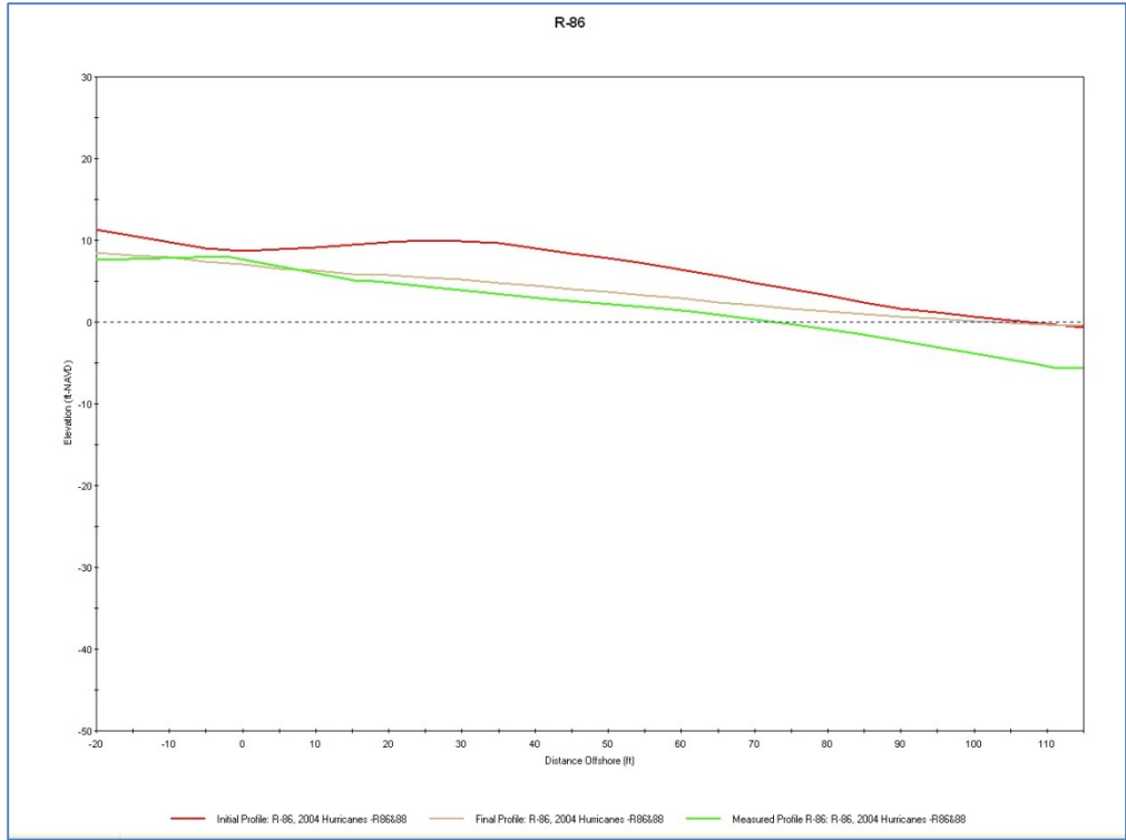
Figure 15. SBEACH Calibration Run (2004 Storm Event), R-86 (Dune to Waterline)
