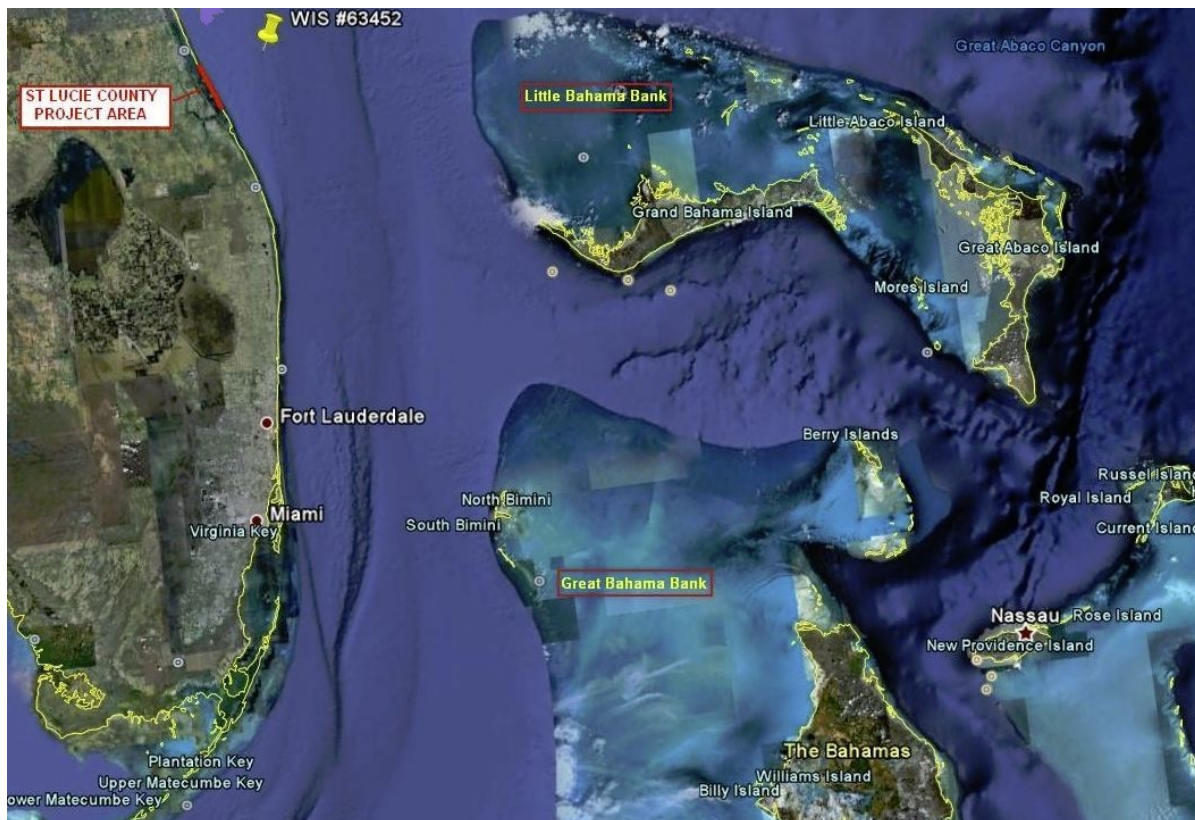
Figure 3-3. Little and Great Bahama Banks
