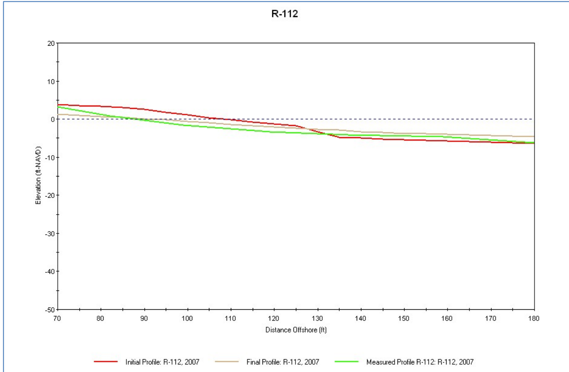
Figure 33. SBEACH Verification Run (2007 Storm Event), R-112 (Dune to Waterline)
