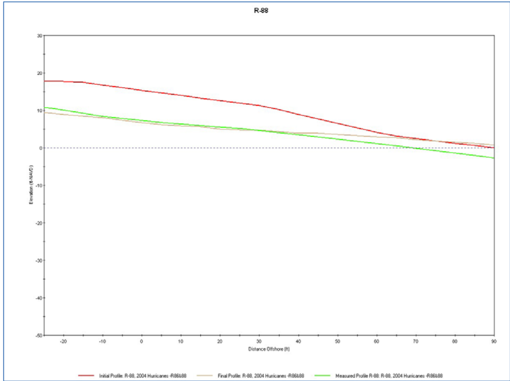
Figure 16. SBEACH Calibration Run (2004 Storm Event), R-88 (Dune to Waterline)
