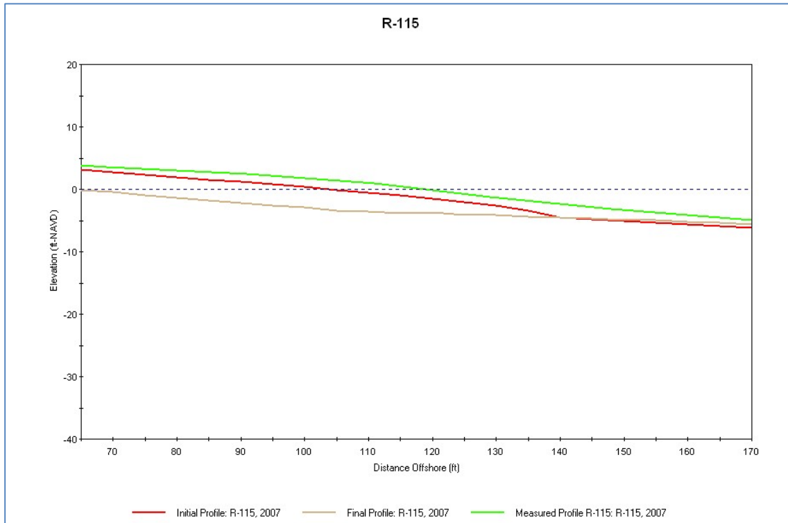
Figure 36. SBEACH Verification Run (2007 Storm Event), R-115 (Dune to Waterline)
