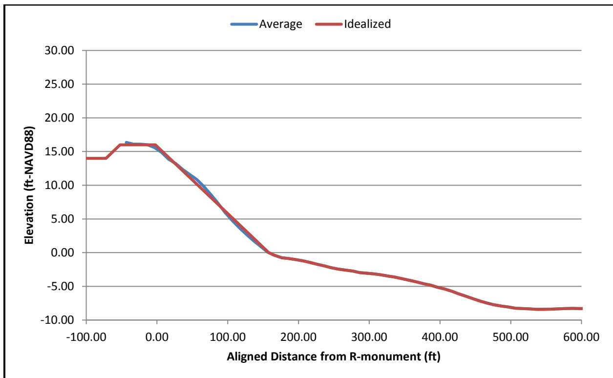
Figure A - 15. Averaged and idealized profiles: P1 grouping.
