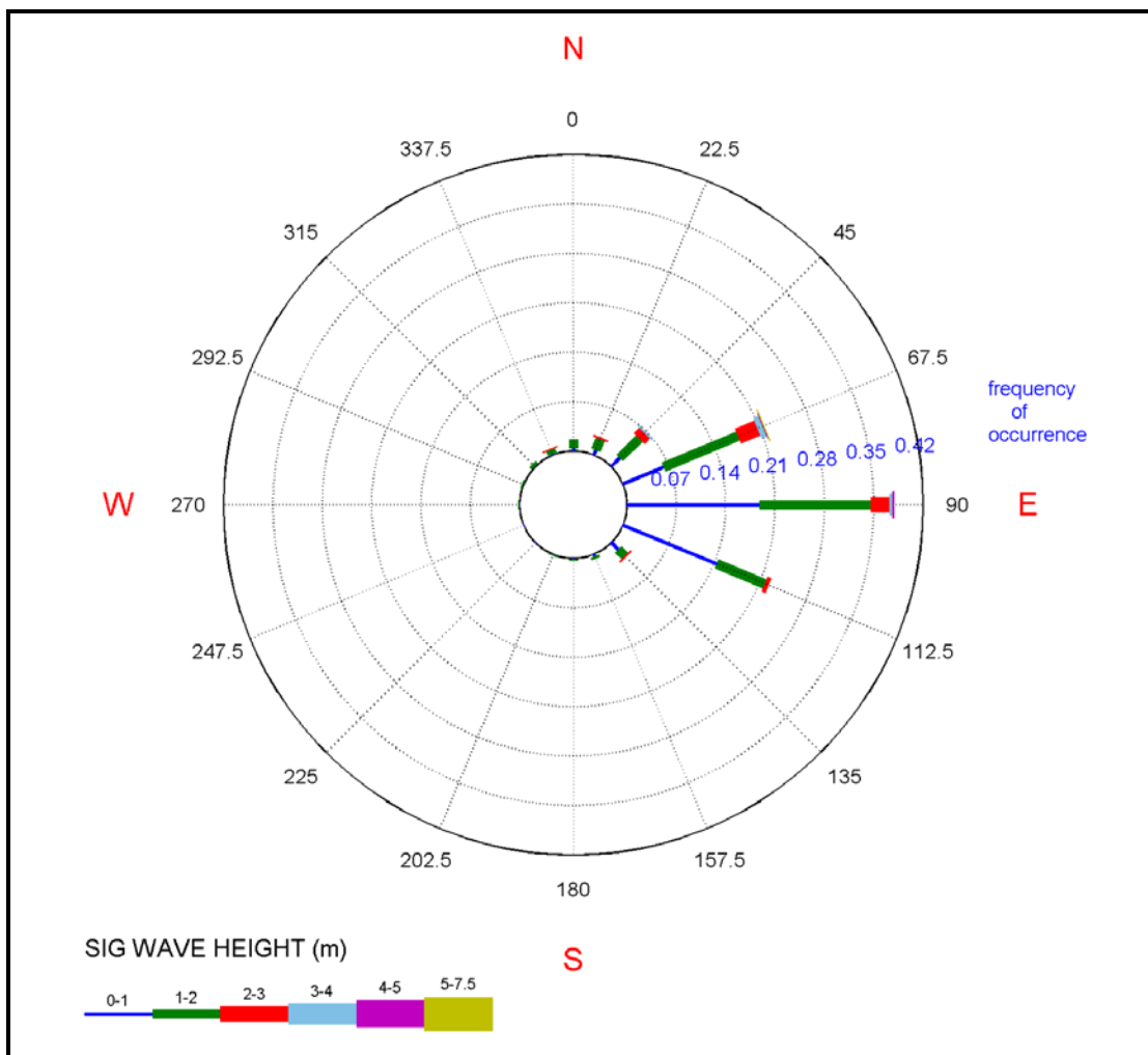
Figure A - 5. Wave rose for WIS Station 63416.
