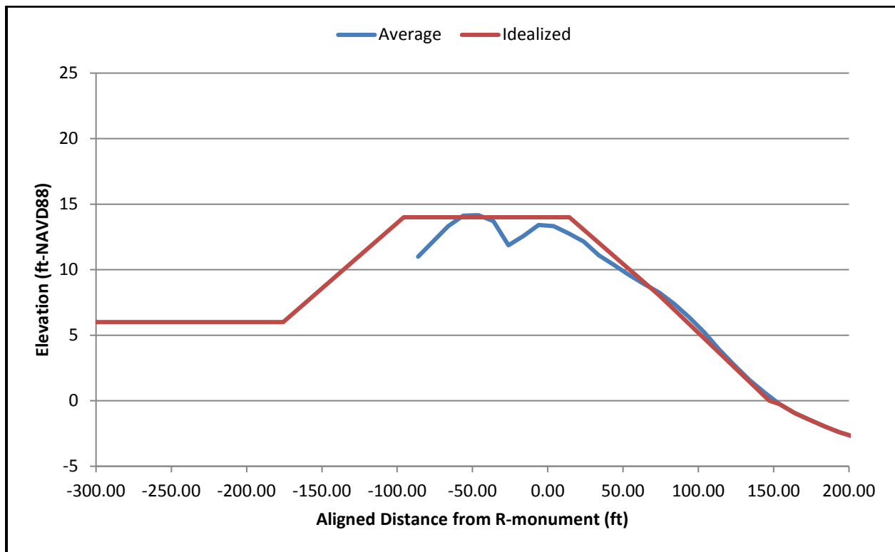
Figure A - 19. Averaged and idealized profiles: P5 grouping.
