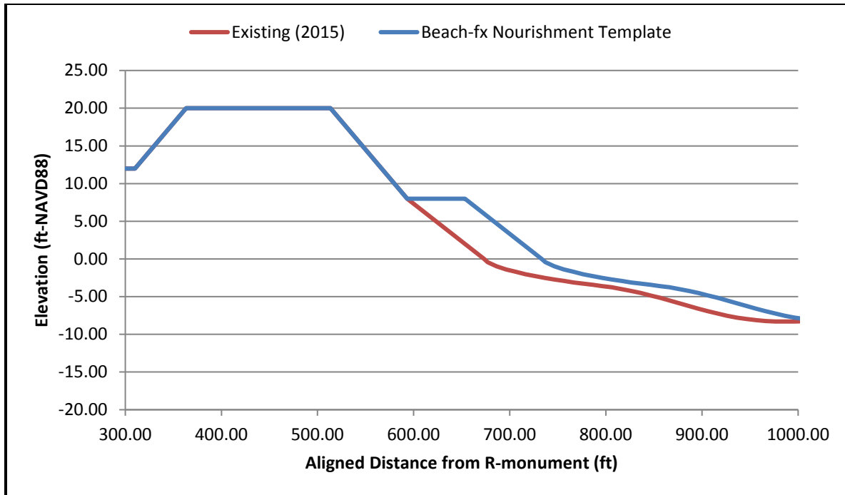
Figure A - 28. Existing profile and Beach-fx nourishment template for idealized Profile 3.
