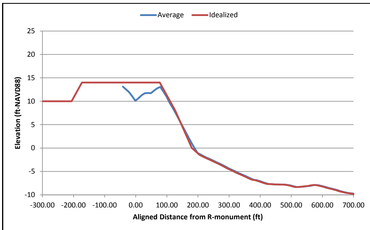
Figure A - 21. Averaged and idealized profiles: P7 grouping.
