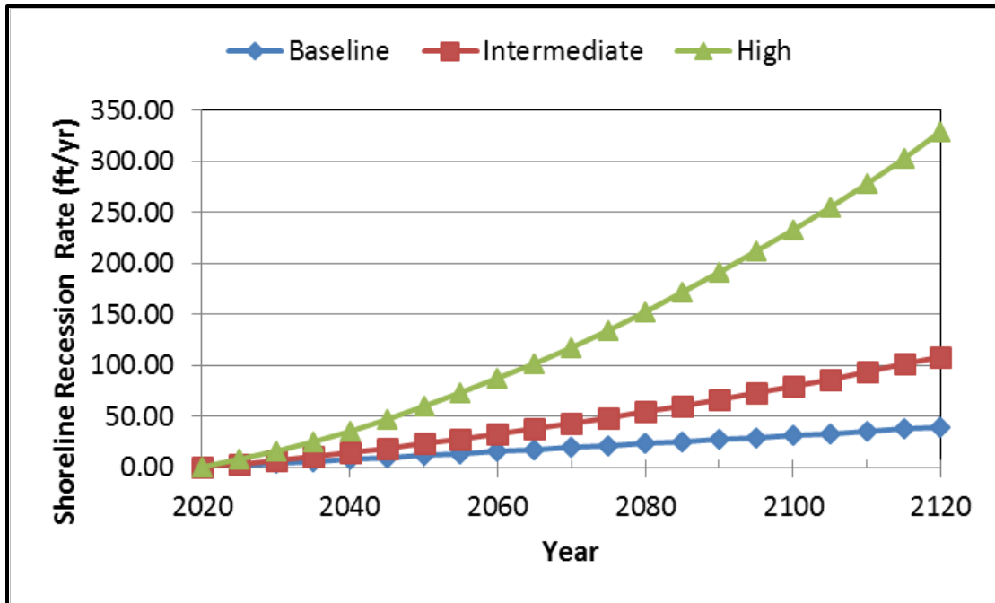
Figure A - 9. Estimated shoreline recession rate due to sea level rise.
