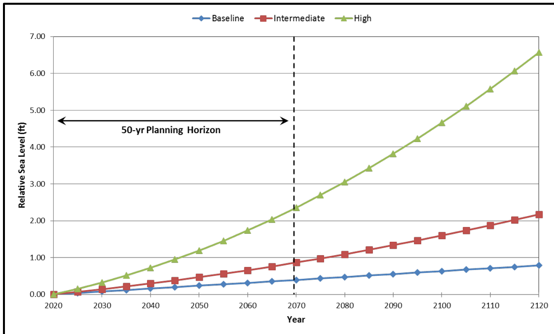
Figure A - 8. Relative sea level change, St. Johns County.
