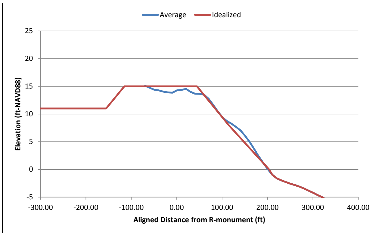
Figure A - 20. Averaged and idealized profiles: P6 grouping.
