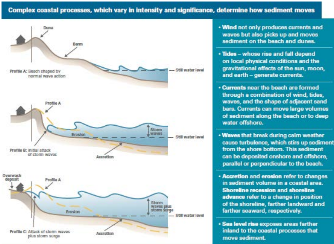
Figure A - 6. Typical coastal processes (from Shore Protection Assessment primer published by USACE-Engineer Research Development Center).
