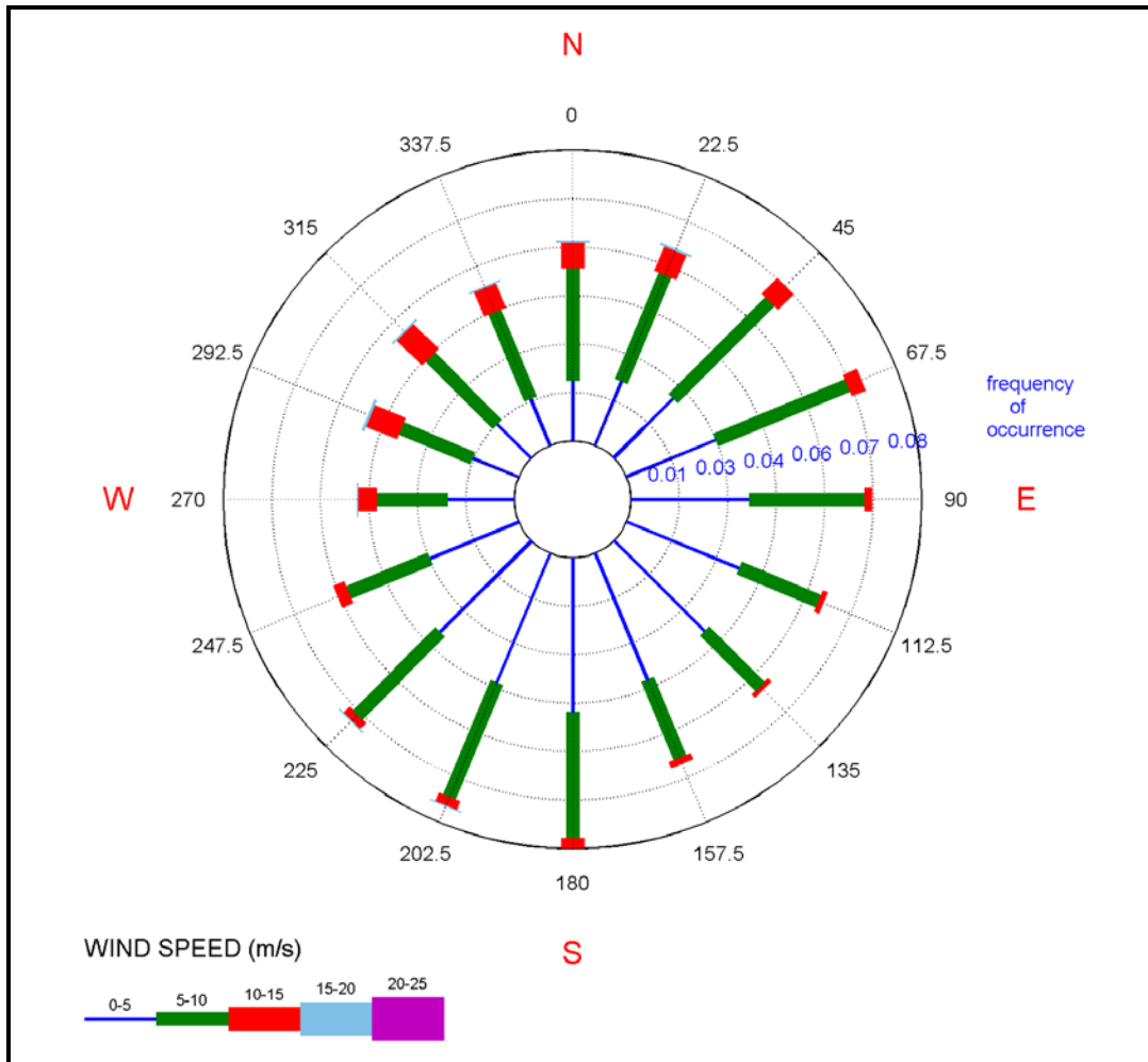
Figure A - 4. Wind rose for WIS Station 63416.
