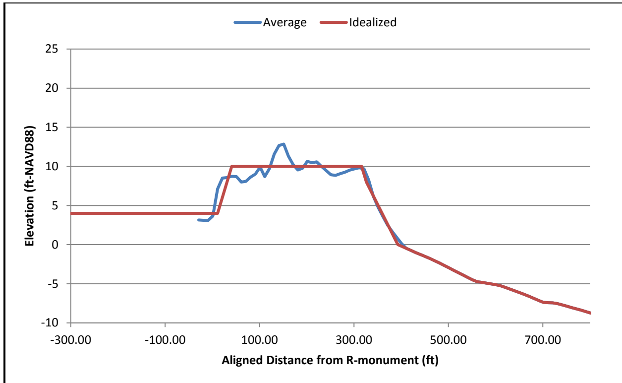
Figure A - 22. Averaged and idealized profiles: P8 grouping.
