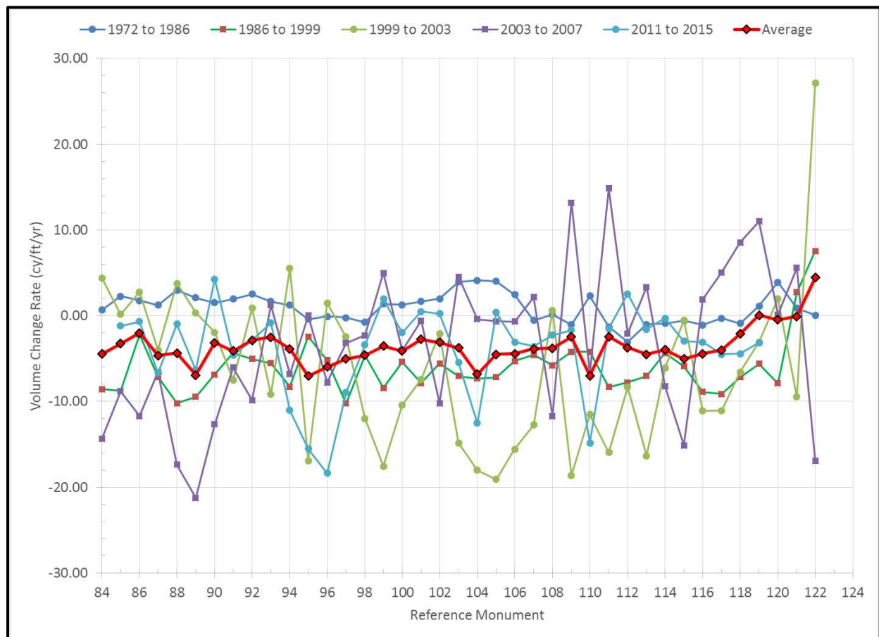
Figure A - 13. Unit volume change rates for the study area.
