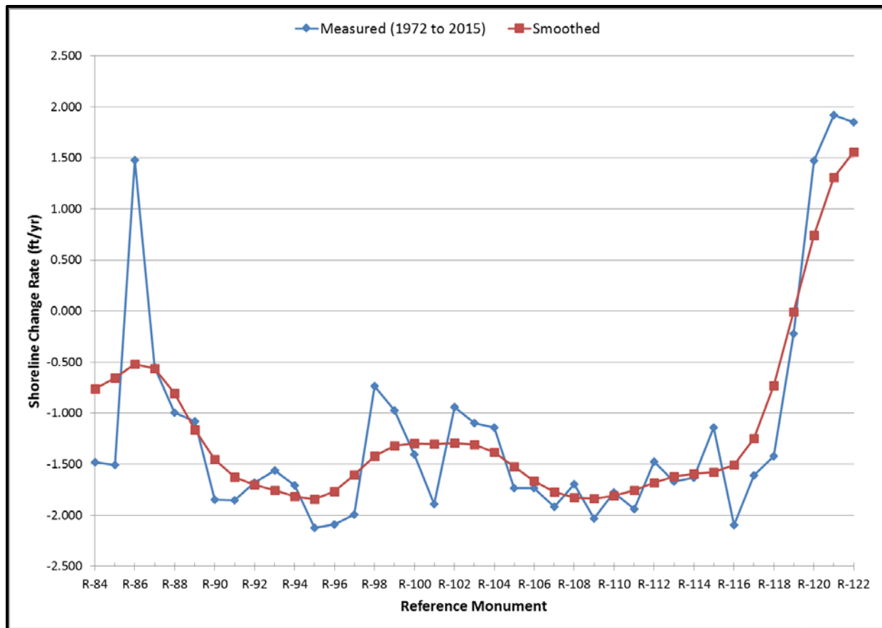
Figure A - 26. Target MHW shoreline change rate.
