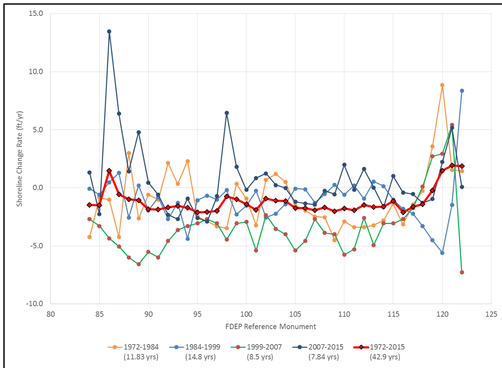
Figure A - 12. Study area shoreline change rates.
