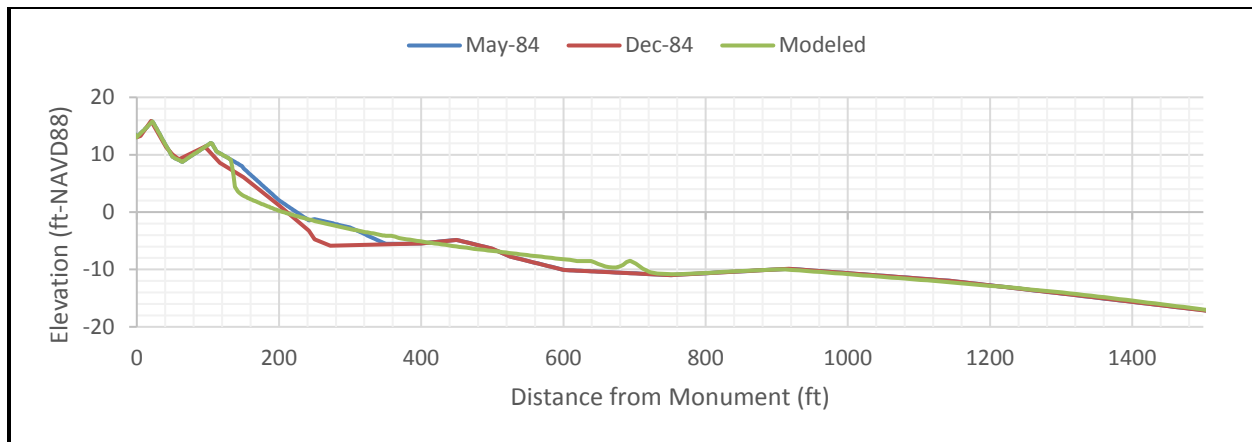
Figure A - 24. Measured and modeled profile change during SBEACH calibration.
