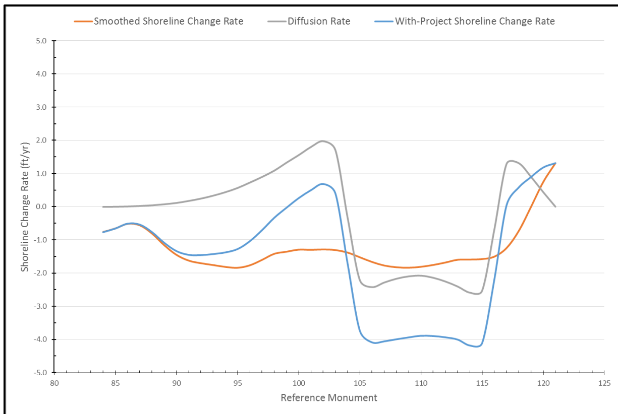
Figure A - 27. Shoreline change rates for with- and without-project simulations.
