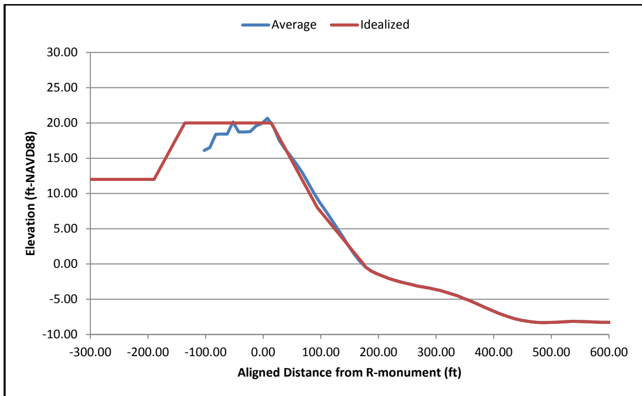
Figure A - 17. Averaged and idealized profiles: P3 grouping.
