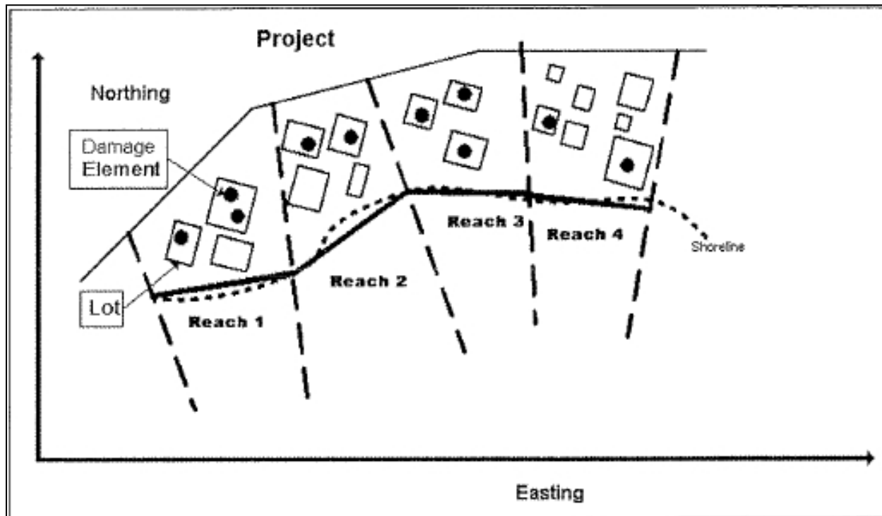
Figure A - 14. Beach- fx model setup representation.
