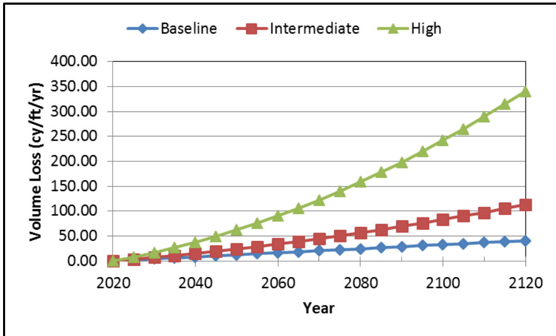
Figure A - 10. Estimated volume loss due to sea level rise.
