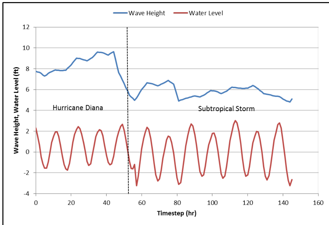
Figure A - 23. Hurricane Diana and 1984 subtropical storm wave and water level data for SBEACH calibration.
