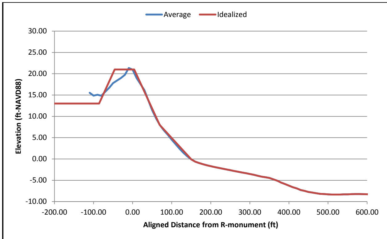
Figure A - 16. Averaged and idealized profiles: P2 grouping.
