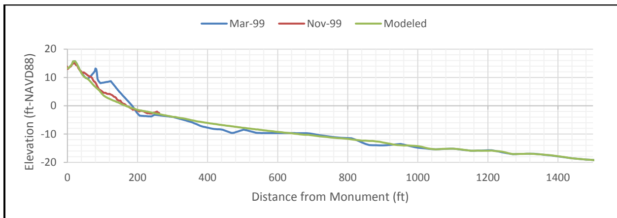
Figure A - 25. Measured and modeled profile change during SBEACH verification.
