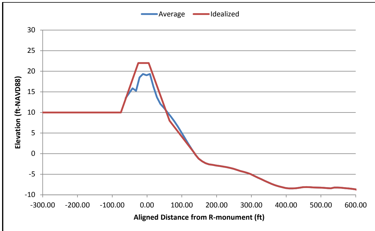
Figure A - 18. Averaged and idealized profiles: P4 grouping.
