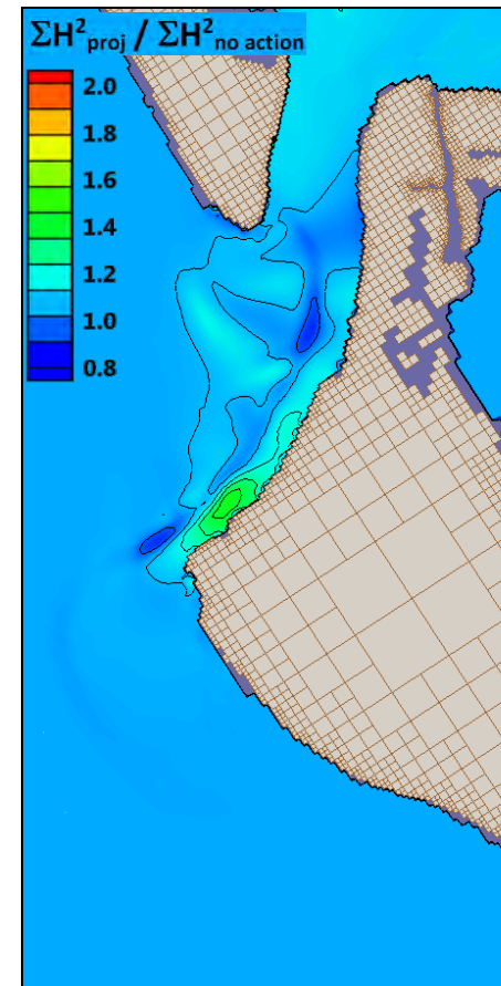
Figure 179: Cumulative Wave Energy May 2004 - November 2004 Alternativ
