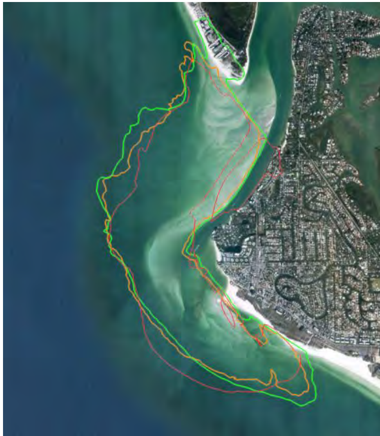
Figure 27: Ebb Shoal Contours 1883, Red; 1991, Orange; 2010, Green
