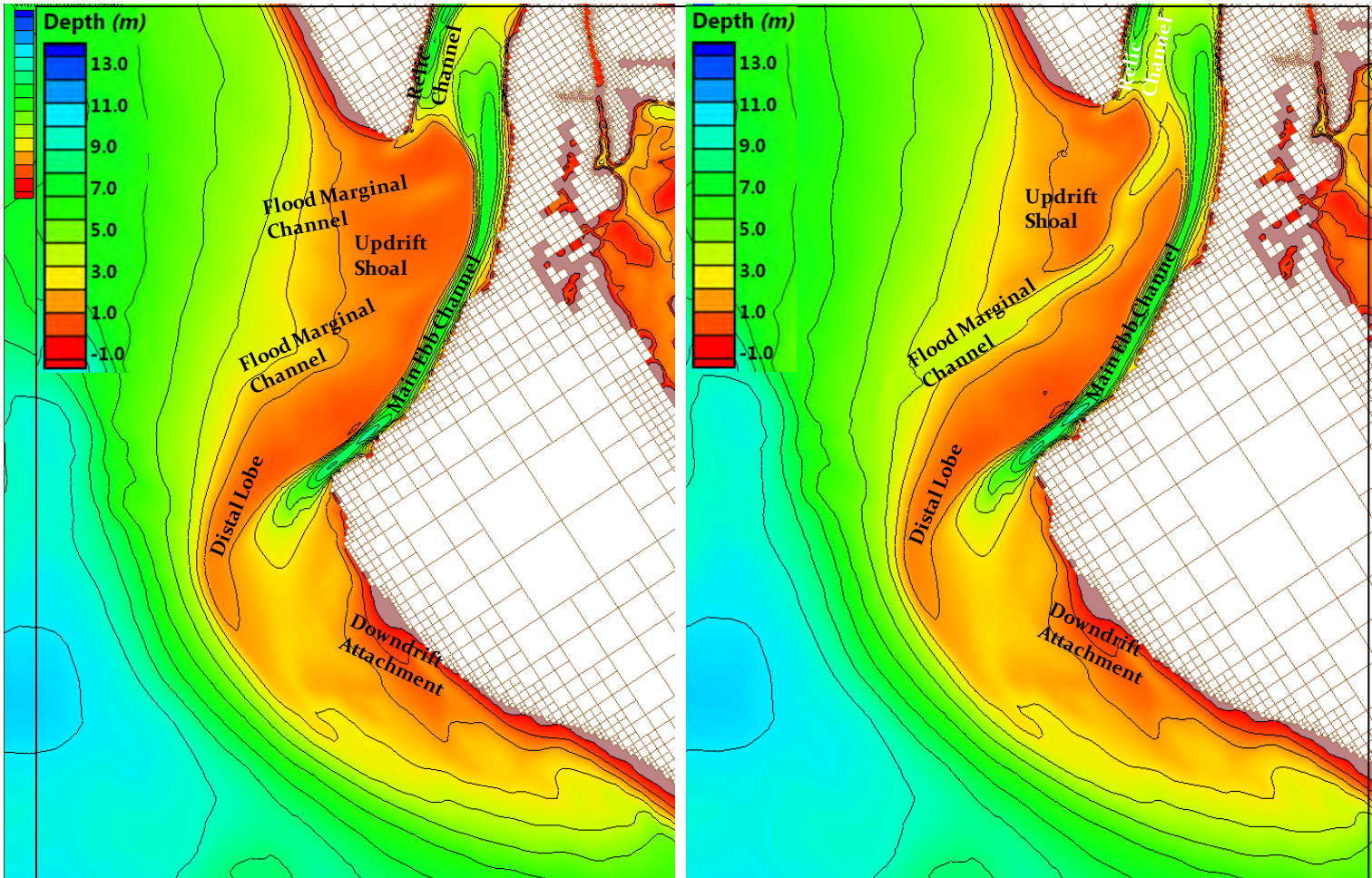
Figure 168: “No Action” Alternative (left), Alternative C (right); end state November 2004
