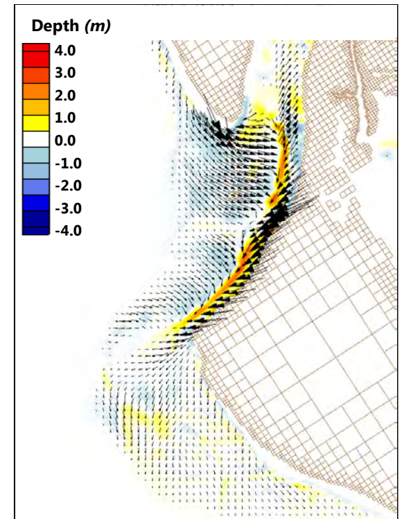
Figure 157: Integrated sediment transport vectors final morphologic change for 2004 bathymetry
