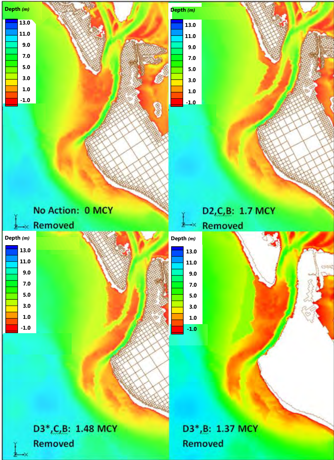
Figure 98: Model grid bathymetry for the 2013 existing condition and the three selected alternatives
