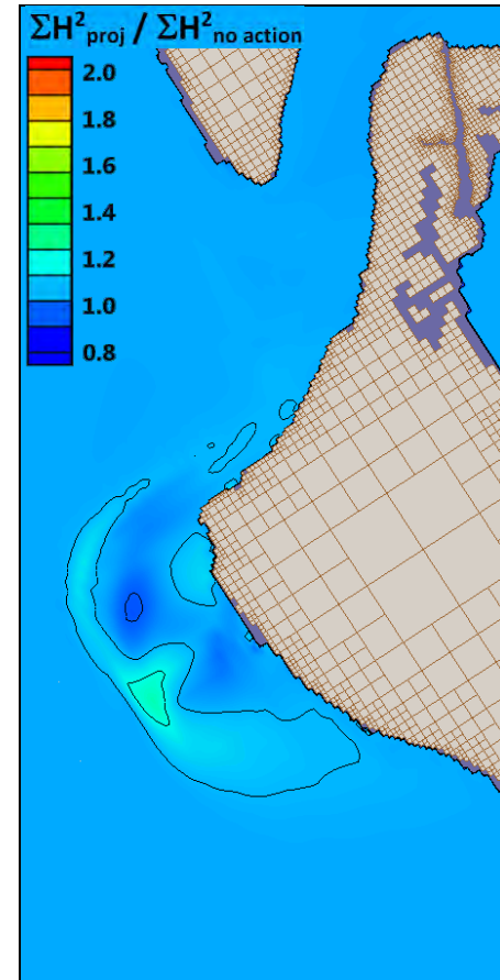
Figure 175: Cumulative Wave Energy May 2004 - November 2004 Alternative B
