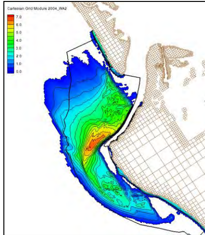
Figure 19: Bathymetry BSP 2004; 20.3MCY
