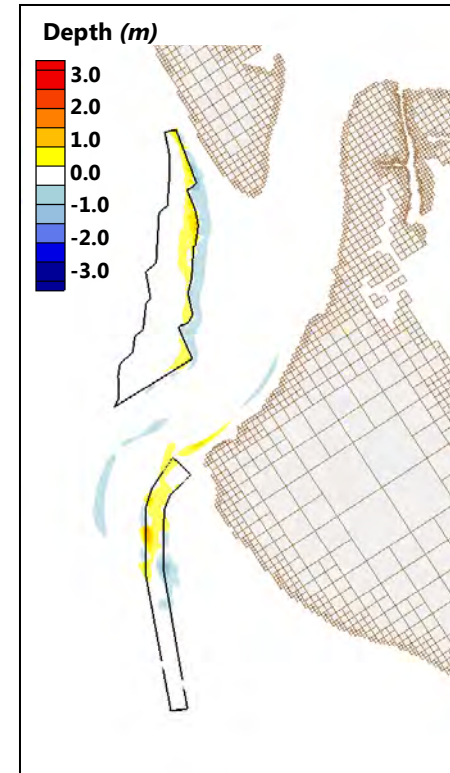
Figure 108: delta Morphology: D3**-B vs. NA
