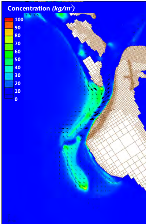
Figure 152: Integrated sediment transport concentration and transport vectors for 1883 bathymetry
