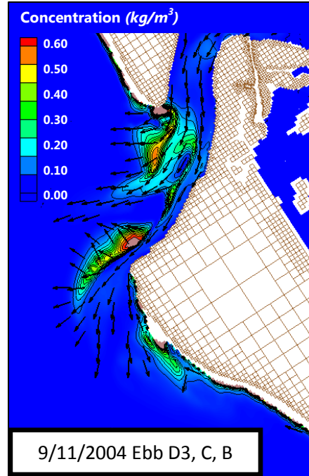
Figure 81: Sediment transport pathways for the 11 September 2004 9:00 pm; Alternative D3*-C-B under southerly storm waves and an ebbing current
