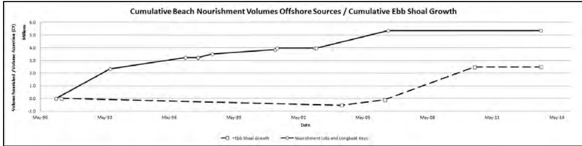
Figure 26: Cumulative Beach Nourishment from Offshore Sources and Ebb Shoal Growth
