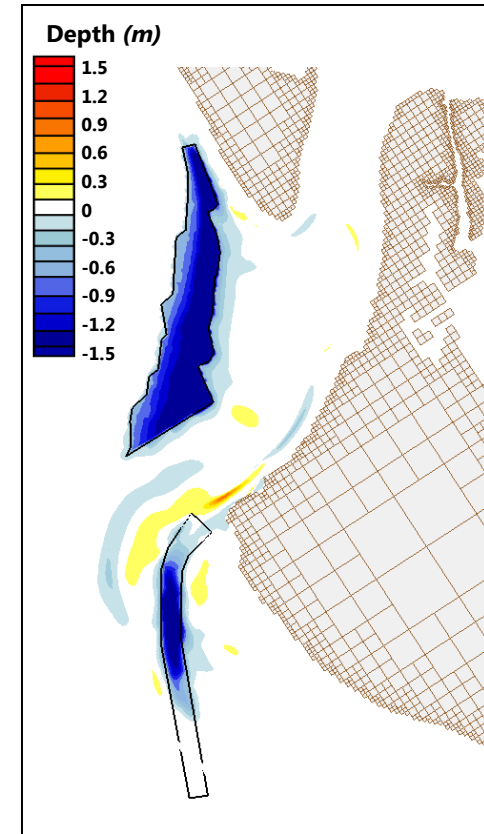
Figure 105: delta Depth: D3**-B vs. NA
