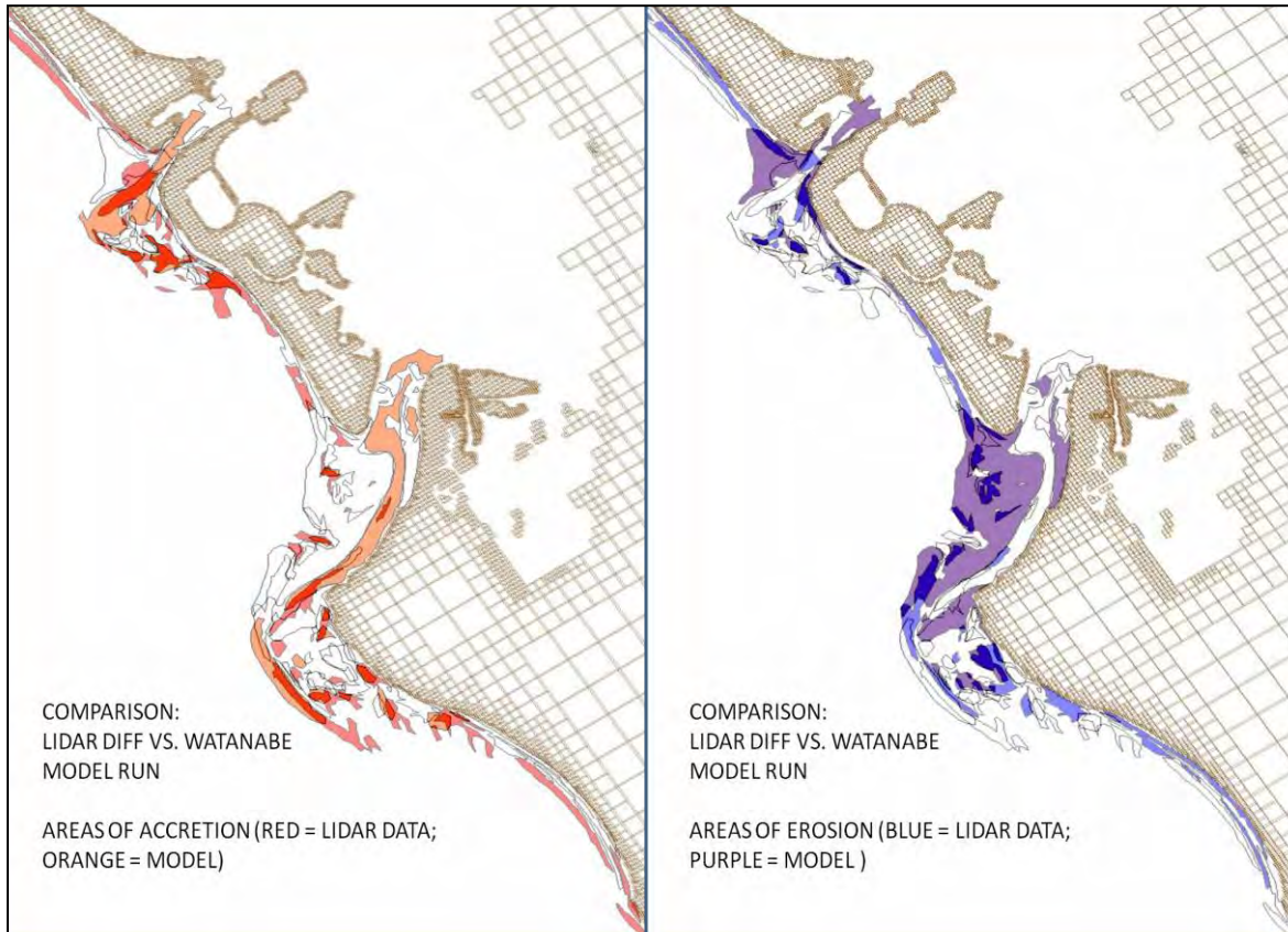
Figure 57: Comparison of Measured 2004 Bathymetry with Calculated 2004 Bathymetry for planform region of Accretion and Erosion
