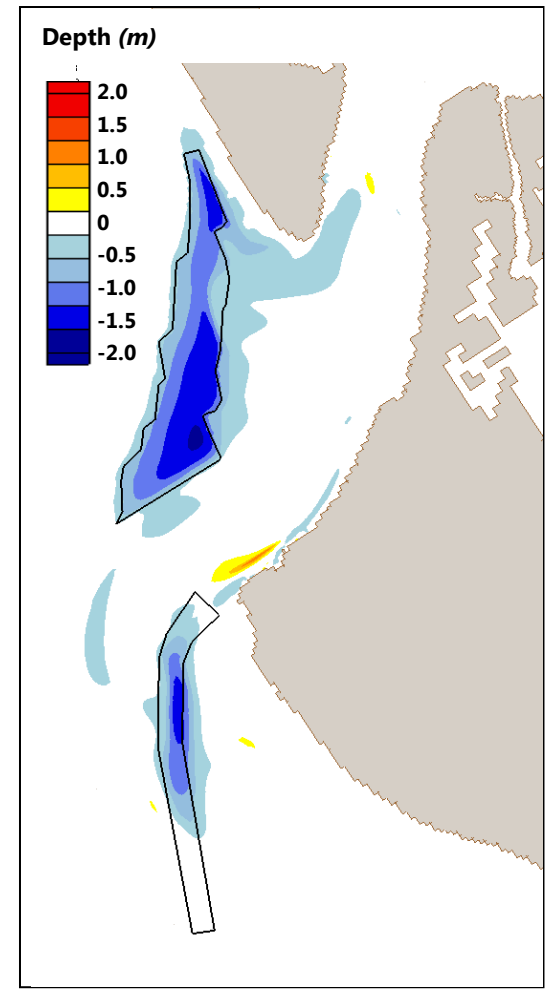
Figure 138: delta Depth: D3**-B vs NA
