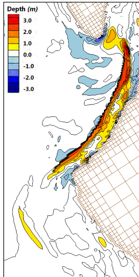
Figure 178: Temporal evolution of the Ebb Shoal; May 2004 - November 204 Alternative C
