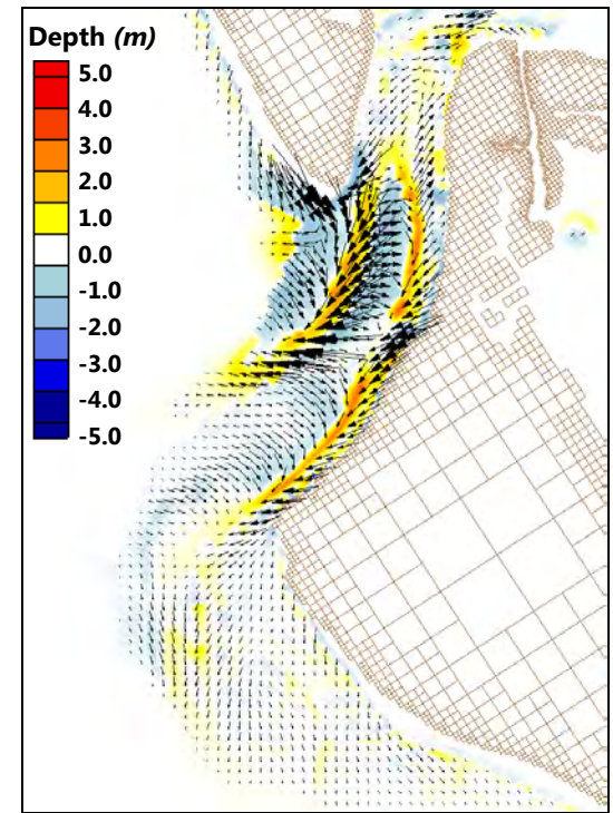
Figure 114: Integrated transport vectors for alternative D2-C B: May 2004 - 2004 waves and final morphologic change
