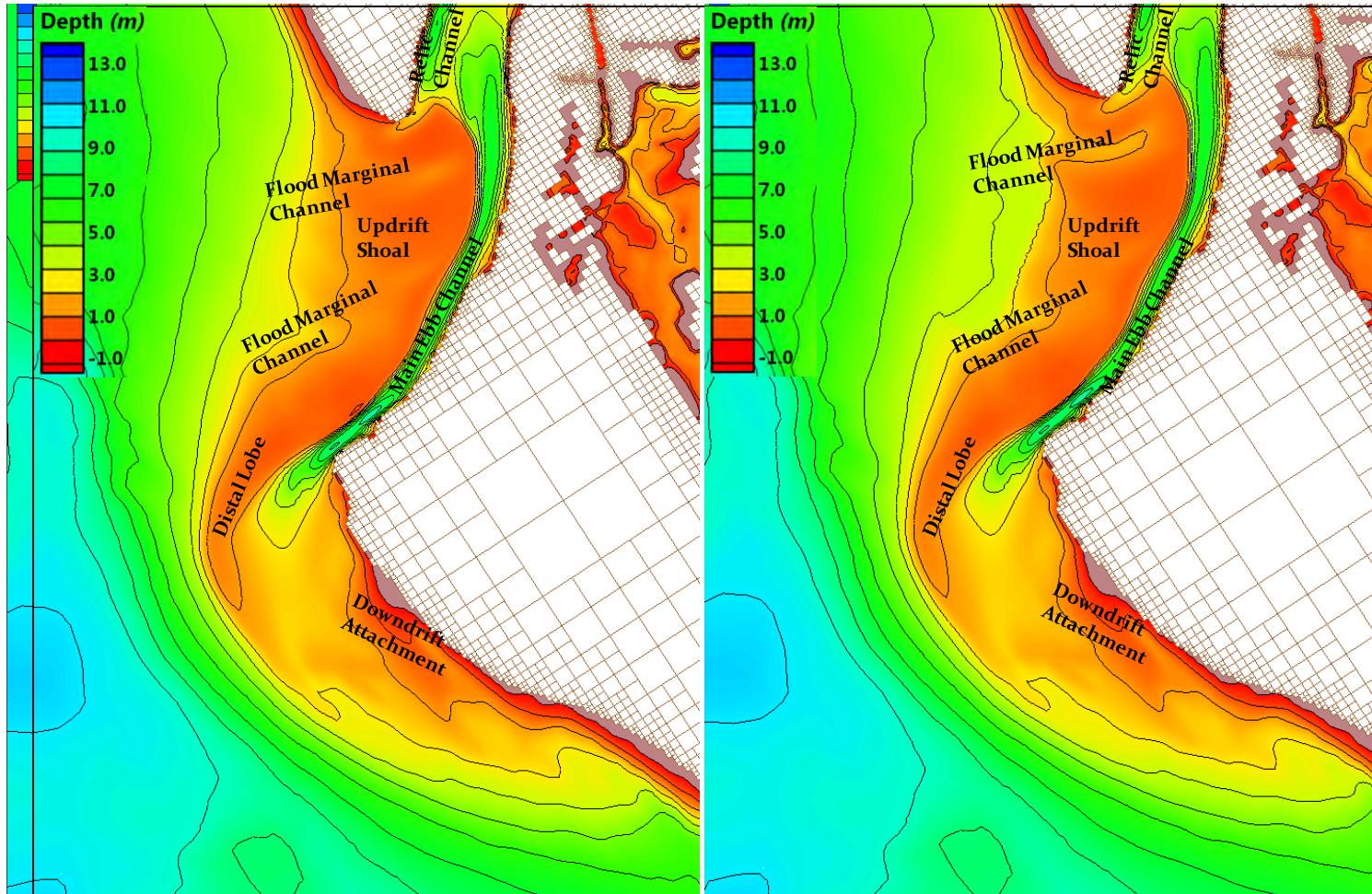
Figure 164: “No Action” Alternative (left), Alternative D2 (right); end state November 2004
