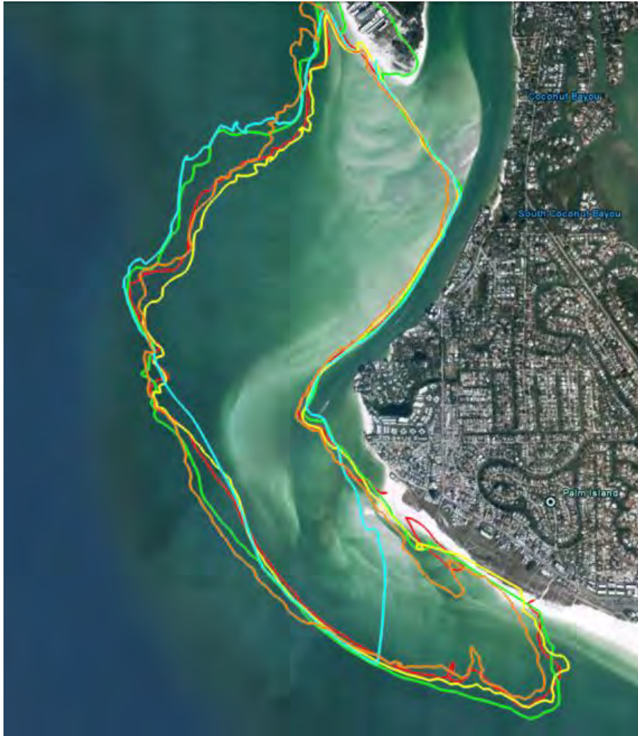
Figure 28: Ebb Shoal Contours: 1991, Orange; 2004, Red; 2006, Yellow; 2010, Green; 2013, Cyan
