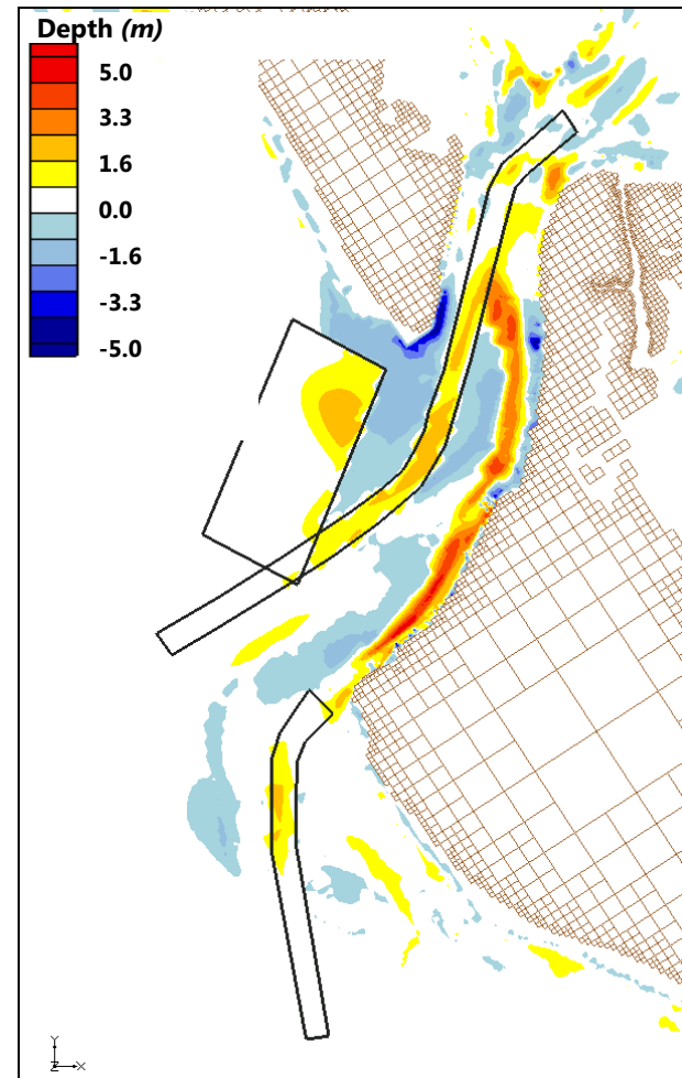
Figure 133: Morphology Change D2-C-B
