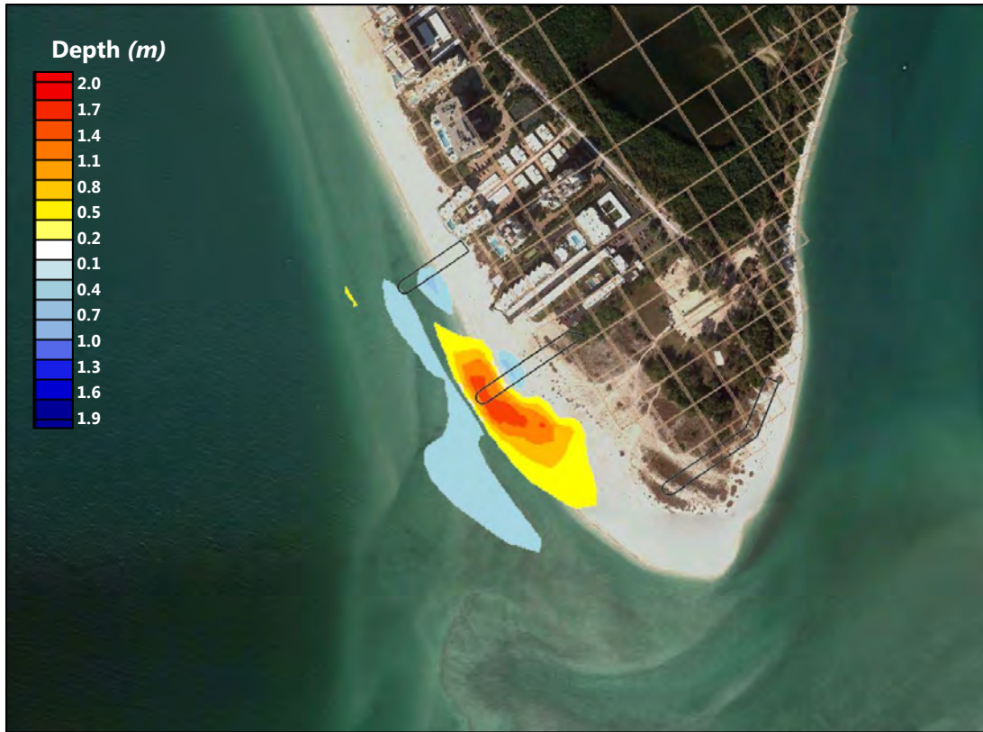
Figure 97: Groins with nourishment; Ending morphology difference for six month run 2004 = (groins were in place with beach nourishment) – (no groins with beach nourishment)
