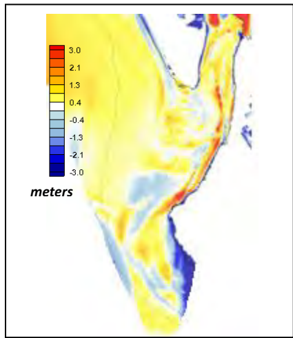
Figure 23: D BSP 2004-2013 3.02MCY
