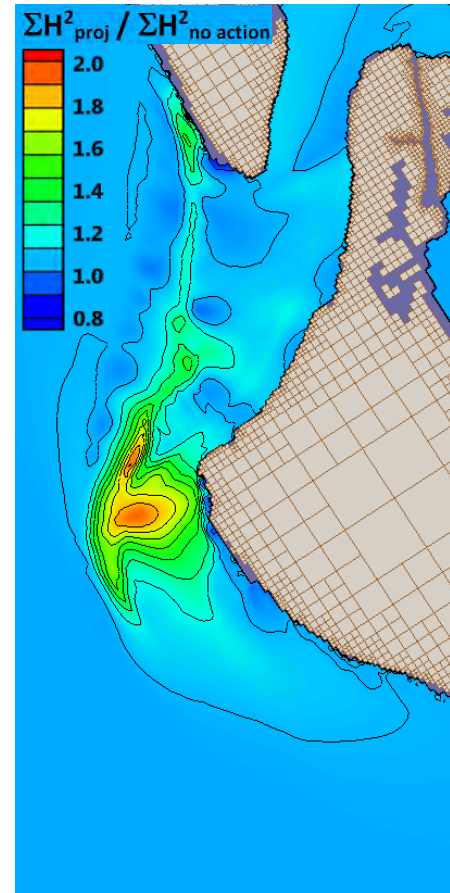
Figure 163: Cumulative Wave Energy May 2004 - November 2004 Alternative D3*-C-B
