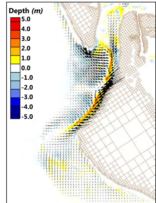
Figure 111: Integrated sediment transport vectors final morphologic change "No Action" Alternative November 2004
