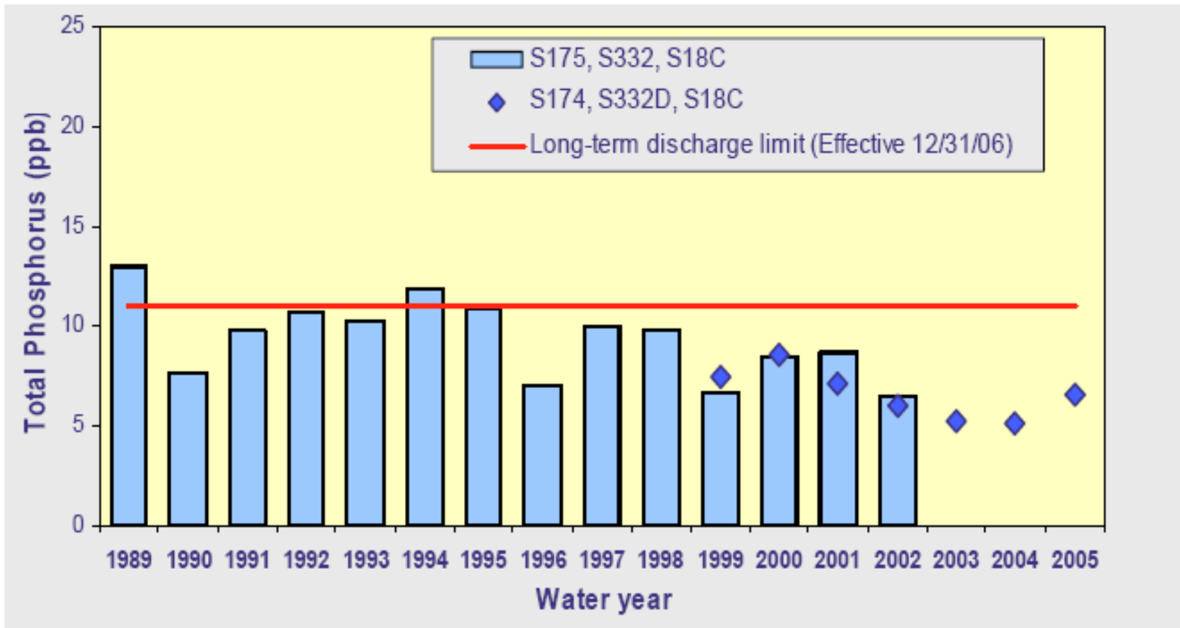
Figure 10 The 12-month flow-weighted mean total phosphorus concentrations in inflows to Everglades National Park through Taylor Slough and the Coastal Basins at the end of each year compared to the 11 ppb long-term total phosphorus limit.
