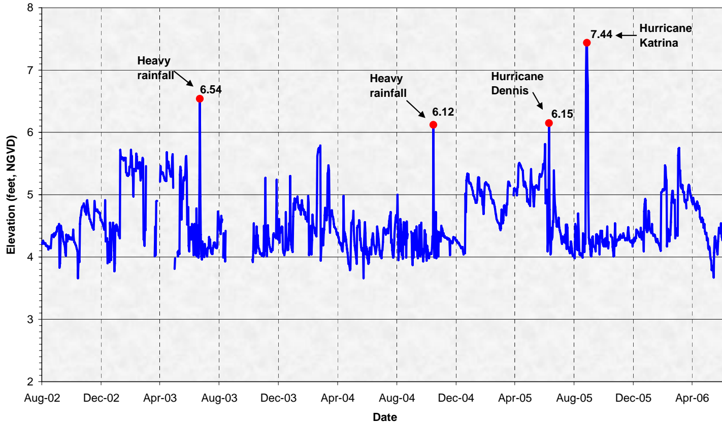
Figure 18 Observed Stages in Middle Reach of L-31N (above S-331)
