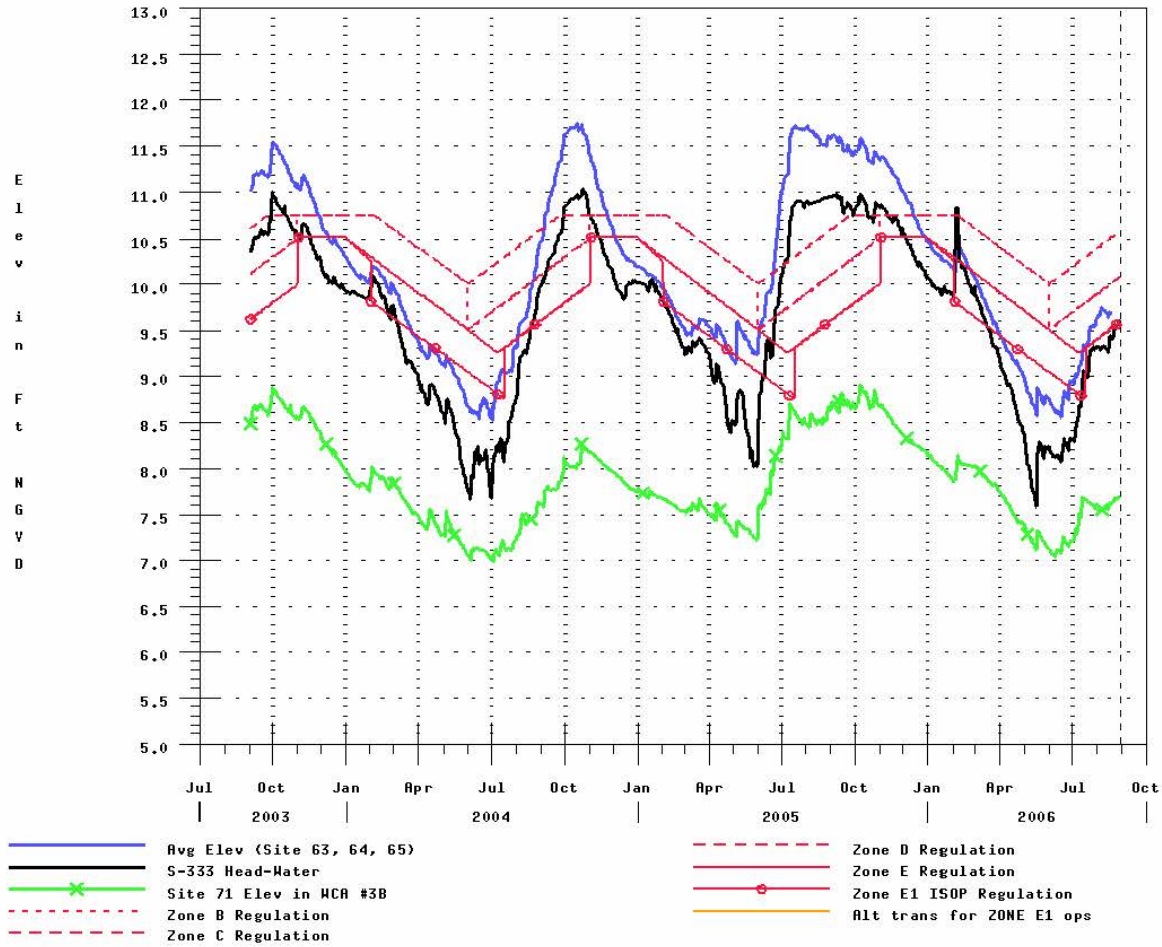
Figure 9. WCA 3A Average Water Elevations and Regulatory Schedule August 2002 – August 2006
