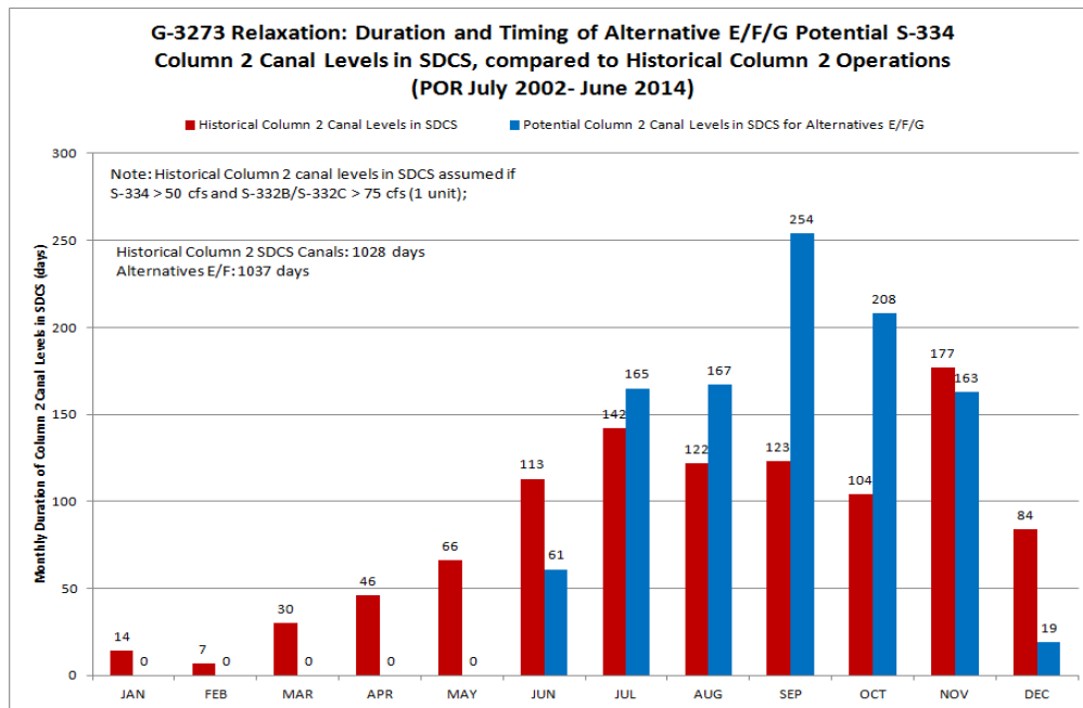
FIGURE 4-27. COMPARISON OF INTRA-ANNUAL VARIABILITY DIFFERENCES BETWEEN HISTORICAL 2002-2014 SDCS COLUMN 2 CANAL OPERATIONS AND THE MODIFIED CRITERIA PROPOSED IN ACTION ALTERNATIVES E/F/G (2002--2014)
