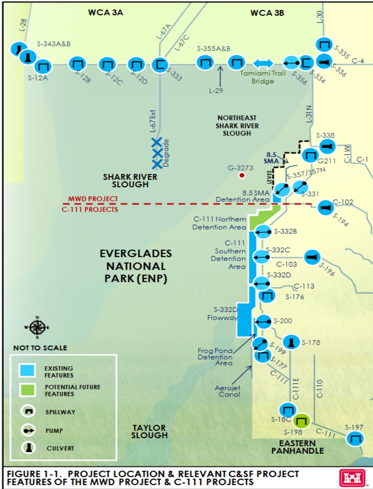
FIGURE 1-1. PROJECT LOCATION AND RELEVANT C&SF PROJECT FEATURES OF THE MWD PROJECT AND C-111 PROJECTS
