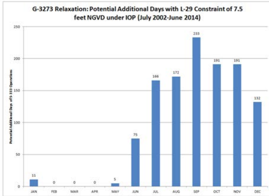
FIGURE 4-5. POTENTIAL ADDITIONAL DAYS OF S-333 OPERATIONS WITH E RTP L-29 CONSTRAINT, 2002-2014 INTRA-ANNUAL VARIABILITY
