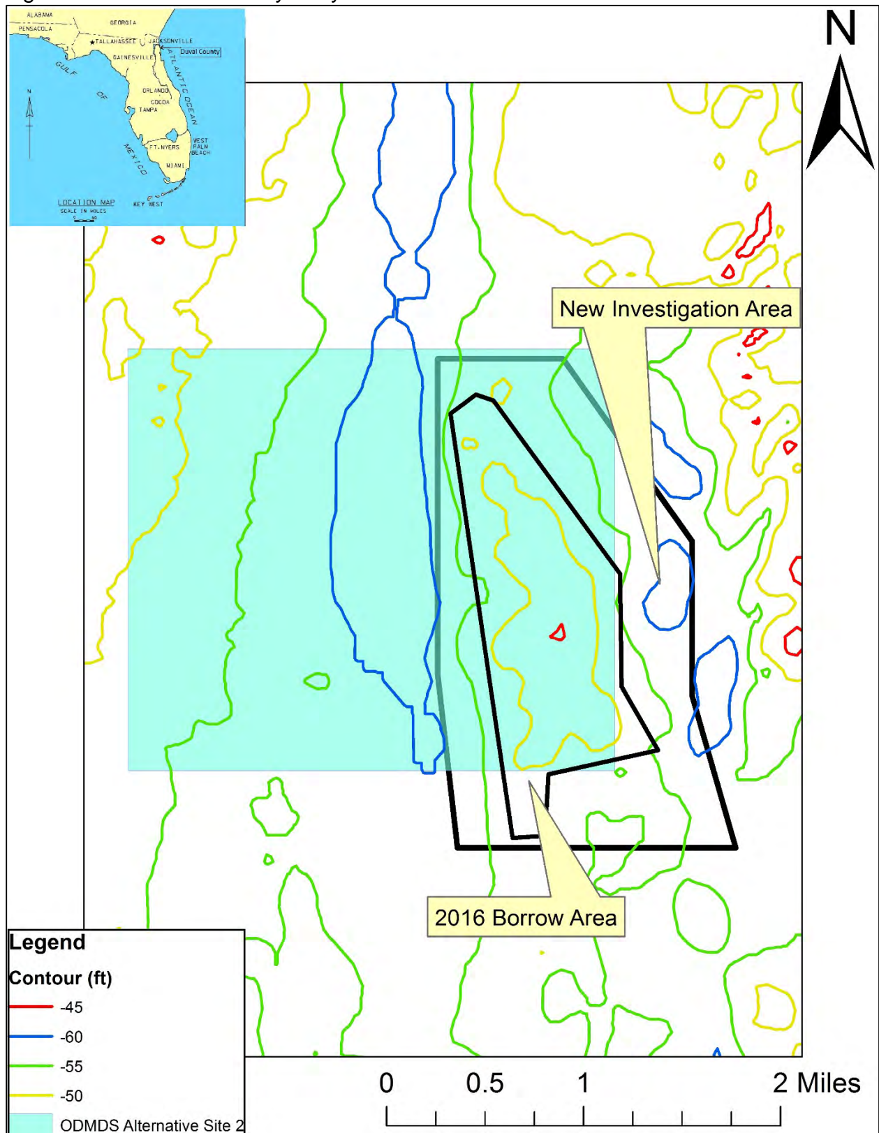
Figure 4. Borrow Area Bathymetry
