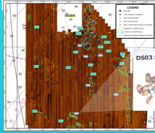
Diver verification stations and example of a diver-extracted sample
