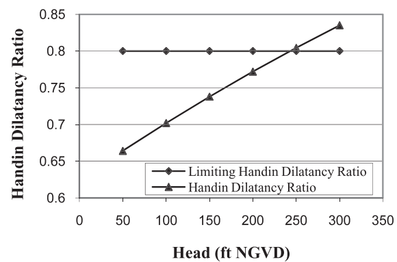
Figure 6. Predictive relation of the Handin Dilatancy Ratio (HDR) and total head in feet (ft), based on the 1929 National Geodetic Vertical Datum (NGVD), for operational recharge phase using the microfracture method. 1 ft = 0.3048 m; 1 psi = 0.006895 MPa.
